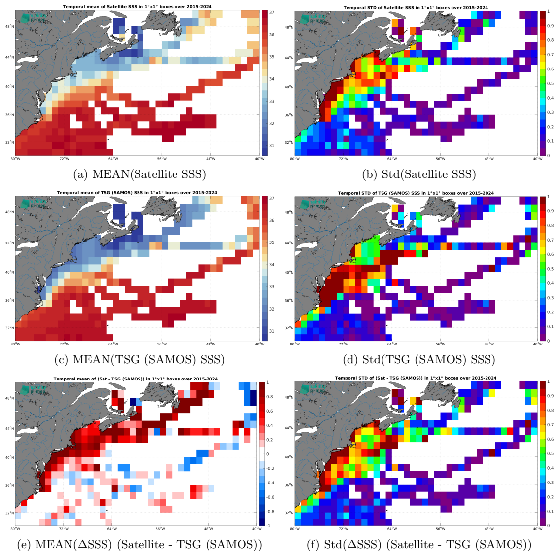
Figure 7: Temporal mean (left) and Std (right) of SSS from SMAP SSS L3 v5.0 - 8-Day running (JPL) (top), TSG (SAMOS) (middle), and of \Delta SSS (Satellite - TSG (SAMOS)). Only match-up pairs are used to generate these maps.
