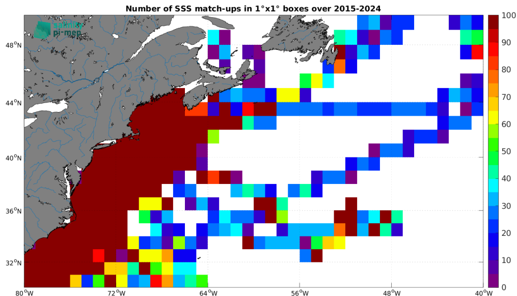
Figure 5: Number of SSS match-ups between TSG (SAMOS) SSS and the SMAP SSS L3 v5.0 - 8-Day running (JPL) SSS product for the Gulf Stream Pi-MEP region over 1^\circ \times 1^\circ boxes and for the full satellite product period.
