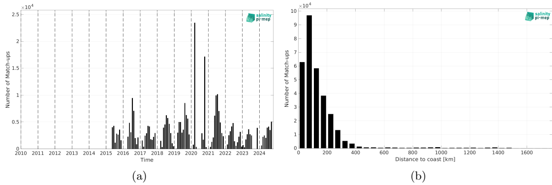
Figure 2: Number of match-ups between TSG (SAMOS) and SMAP SSS L3 v5.0 - 8-Day running (JPL) SSS as a function of time (a) and as function of the distance to coast (b) over the Gulf Stream Pi-MEP region and for the full satellite product period.
