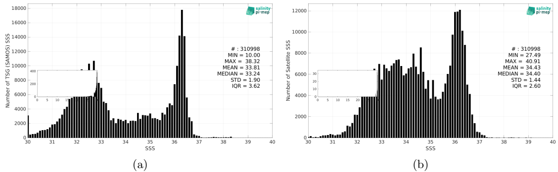
Figure 3: Histograms of SSS from TSG (SAMOS) (a) and SMAP SSS L3 v5.0 - 8-Day running (JPL) (b) considering all match-up pairs per bins of 0.1 over the Gulf Stream Pi-MEP region and for the full satellite product period.
