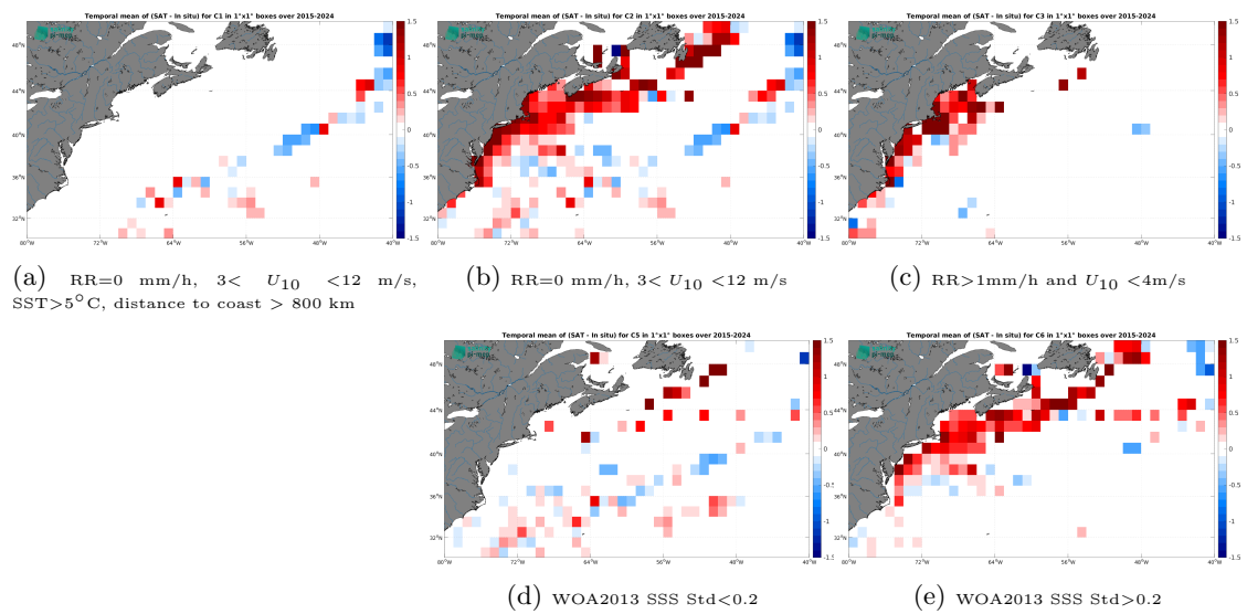
Figure 14: Temporal mean gridded over spatial boxes of size 1^\circ \times 1^\circ of \Delta SSS (SMAP SSS L3 v5.0 - 8-Day running (JPL) - TSG (SAMOS)) for 5 different subdatasets corresponding to:RR=0 mm/h, 3 < U_{10} < 12 m/s, SST > 5^\circ C , distance to coast > 800 km (a), RR=0 mm/h, 3 < U_{10} < 12 m/s (b), RR>1mm/h and U_{10} < 4 m/s (c), WOA2013 SSS Std<0.2 (d), WOA2013 SSS Std>0.2 (e).
