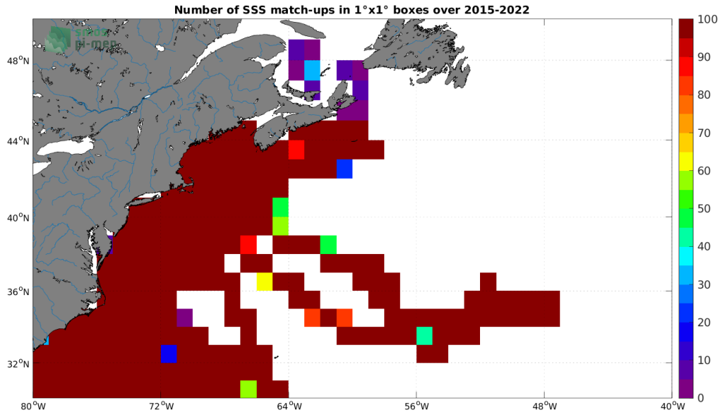
Figure 4: Number of SSS match-ups between TSG (SAMOS) SSS and the SMAP SSS L3 v5.0 - 8-Day running (JPL) SSS product for the Gulf Stream Pi-MEP region over 1^\circ \times 1^\circ boxes and for the full satellite product period.
