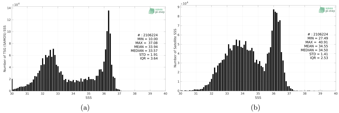
Figure 2: Histograms of SSS from TSG (SAMOS) (a) and SMAP SSS L3 v5.0 - 8-Day running (JPL) (b) considering all match-up pairs per bins of 0.1 over the Gulf Stream Pi-MEP region and for the full satellite product period.
