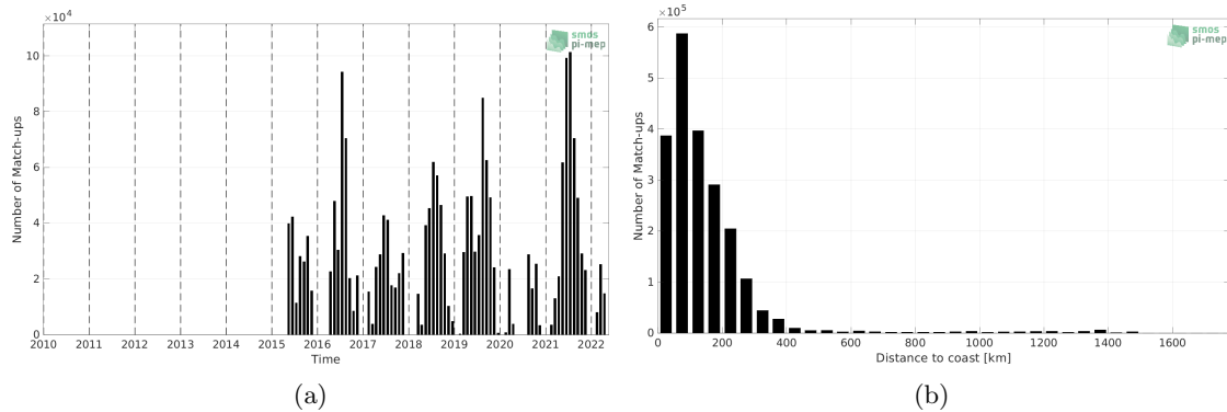
Figure 1: Number of match-ups between TSG (SAMOS) and SMAP SSS L3 v5.0 - 8-Day running (JPL) SSS as a function of time (a) and as function of the distance to coast (b) over the Gulf Stream Pi-MEP region and for the full satellite product period.
