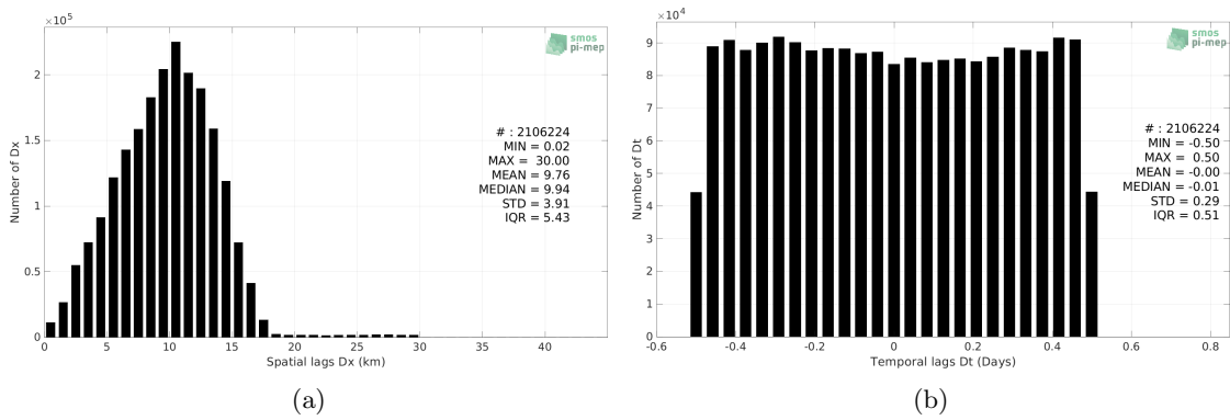
Figure 5: Histograms of the spatial (a) and temporal (b) lags between the location/time of the TSG (SAMOS) measurement and the date of the corresponding SMAP SSS L3 v5.0 - 8-Day running (JPL) SSS pixel.
