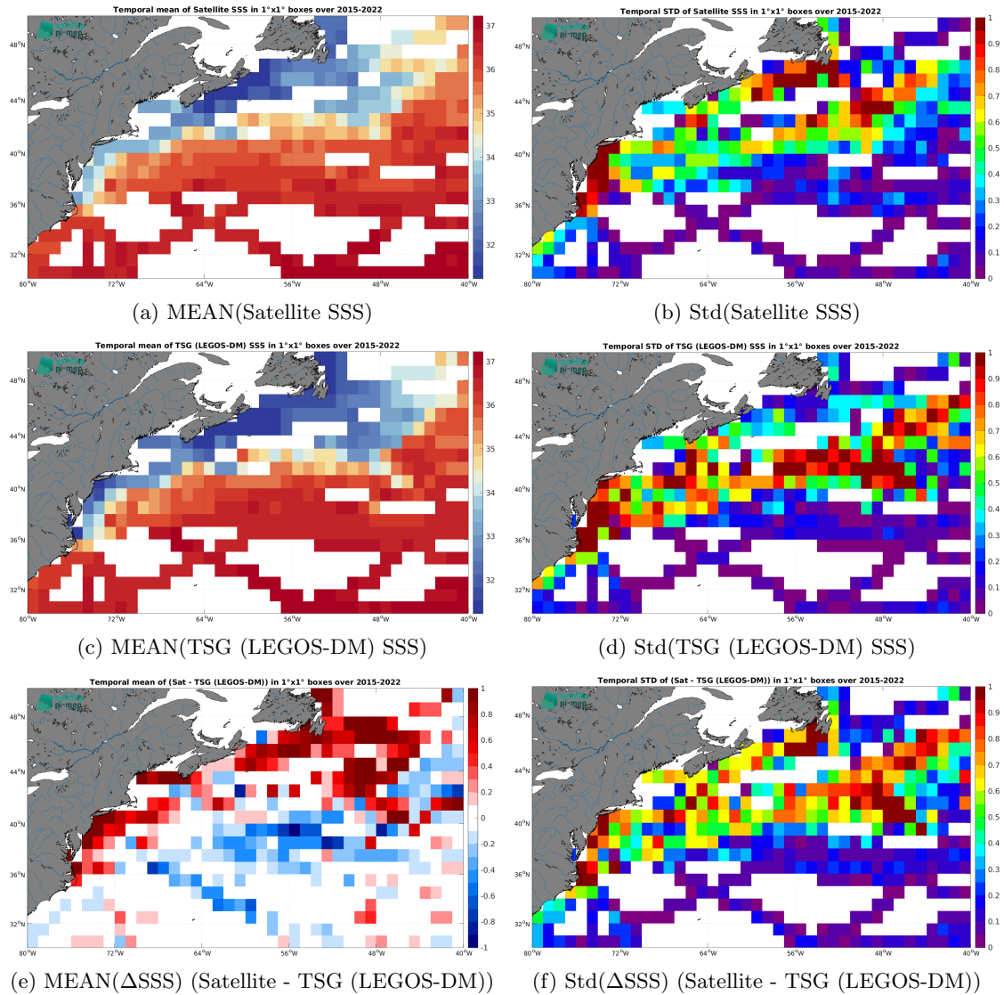
Figure 7: Temporal mean (left) and Std (right) of SSS from SMAP SSS L3 v5.0 - 8-Day running (JPL) (top), TSG (LEGOS-DM) (middle), and of \Delta SSS (Satellite - TSG (LEGOS-DM)). Only match-up pairs are used to generate these maps.
