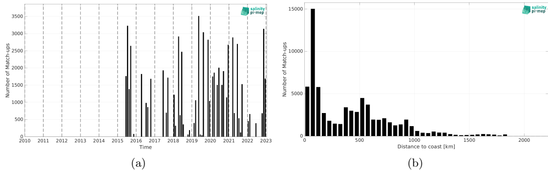
Figure 2: Number of match-ups between TSG (LEGOS-DM) and SMAP SSS L3 v5.0 - 8-Day running (JPL) SSS as a function of time (a) and as function of the distance to coast (b) over the Gulf Stream Pi-MEP region and for the full satellite product period.
