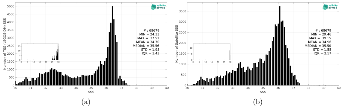
Figure 3: Histograms of SSS from TSG (LEGOS-DM) (a) and SMAP SSS L3 v5.0 - 8-Day running (JPL) (b) considering all match-up pairs per bins of 0.1 over the Gulf Stream Pi-MEP region and for the full satellite product period.
