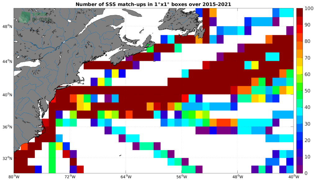
Figure 4: Number of SSS match-ups between TSG (LEGOS-DM) SSS and the SMAP SSS L3 v5.0 - 8-Day running (JPL) SSS product for the Gulf Stream Pi-MEP region over 1^\circ \times 1^\circ boxes and for the full satellite product period.
