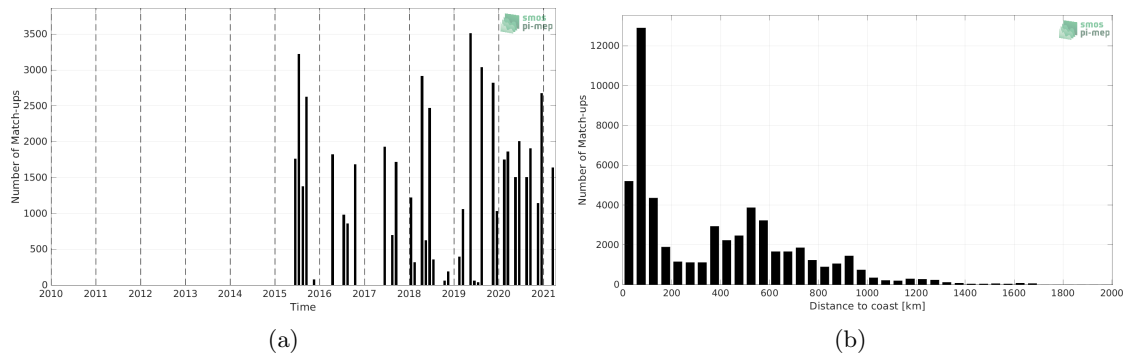
Figure 1: Number of match-ups between TSG (LEGOS-DM) and SMAP SSS L3 v5.0 - 8-Day running (JPL) SSS as a function of time (a) and as function of the distance to coast (b) over the Gulf Stream Pi-MEP region and for the full satellite product period.
