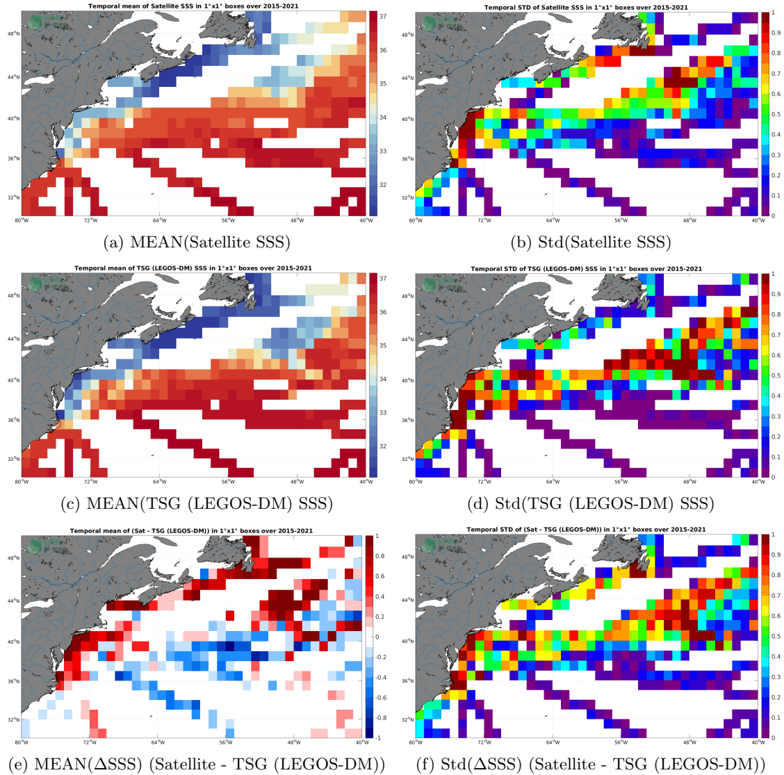
Figure 6: Temporal mean (left) and Std (right) of SSS from SMAP SSS L3 v5.0 - 8-Day running (JPL) (top), TSG (LEGOS-DM) (middle), and of \Delta SSS (Satellite - TSG (LEGOS-DM)). Only match-up pairs are used to generate these maps.
