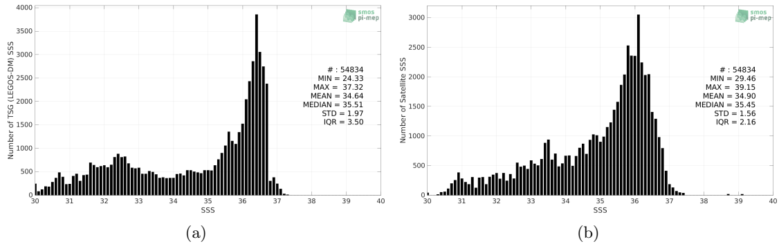
Figure 2: Histograms of SSS from TSG (LEGOS-DM) (a) and SMAP SSS L3 v5.0 - 8-Day running (JPL) (b) considering all match-up pairs per bins of 0.1 over the Gulf Stream Pi-MEP region and for the full satellite product period.
