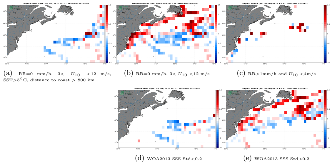
Figure 12: Temporal mean gridded over spatial boxes of size 1^\circ \times 1^\circ of \Delta SSS (SMAP SSS L3 v5.0 - 8-Day running (JPL) - TSG (LEGOS-DM)) for 5 different subdatasets corresponding to:RR=0 mm/h, 3 < U_{10} < 12 m/s, SST >5^\circ C, distance to coast > 800 km (a), RR=0 mm/h, 3 < U_{10} < 12 m/s (b), RR >1 mm/h and U_{10} < 4 m/s (c), WOA2013 SSS Std <0.2 (d), WOA2013 SSS Std >0.2 (e).
