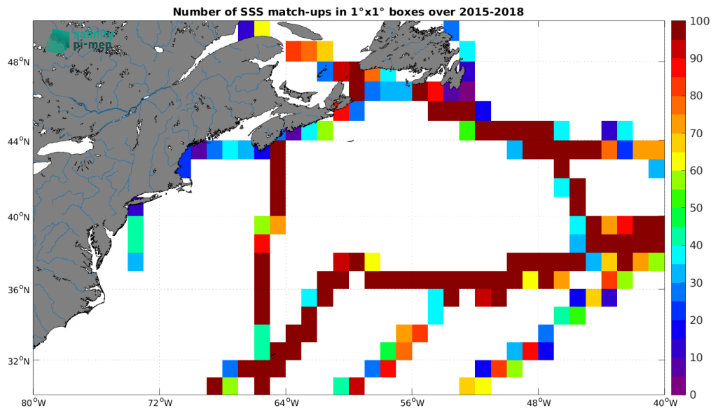
Figure 5: Number of SSS match-ups between TSG (GOSUD-Sailing-ship) SSS and the SMAP SSS L3 v5.0 - 8-Day running (JPL) SSS product for the Gulf Stream Pi-MEP region over 1^\circ \times 1^\circ boxes and for the full satellite product period.
