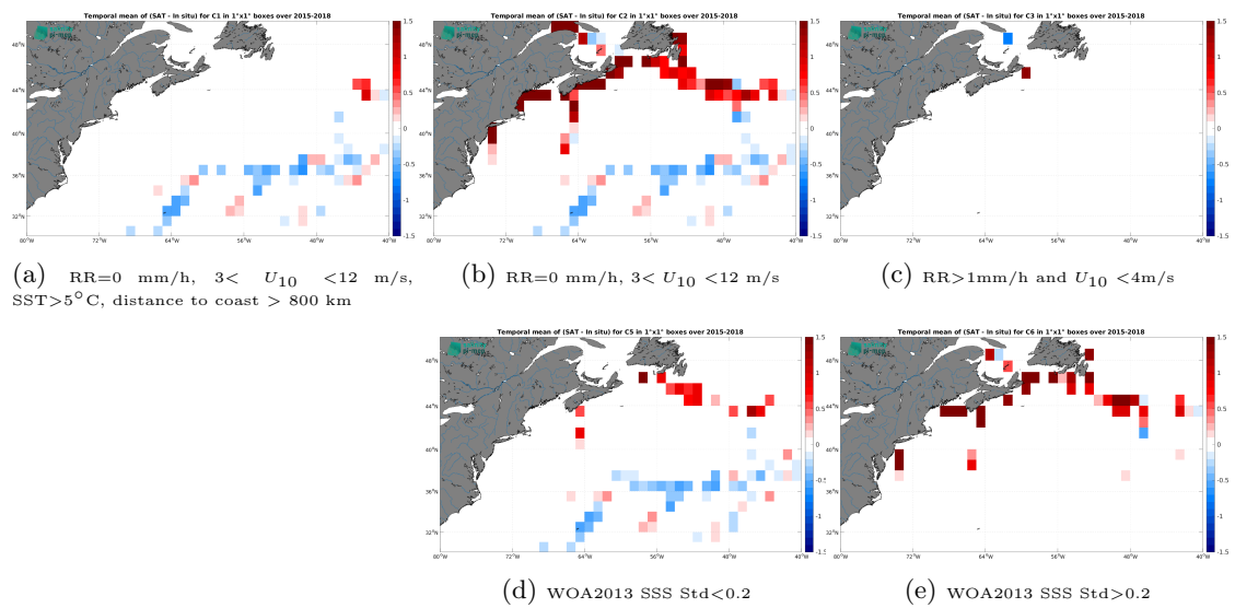
Figure 14: Temporal mean gridded over spatial boxes of size 1^\circ \times 1^\circ of \Delta SSS (SMAP SSS L3 v5.0 - 8-Day running (JPL) - TSG (GOSUD-Sailing-ship)) for 5 different subdatasets corresponding to: RR=0 mm/h, 3 < U_{10} < 12 m/s, SST>5°C, distance to coast > 800 km (a), RR=0 mm/h, 3 < U_{10} < 12 m/s (b), RR>1mm/h and U_{10} < 4 m/s (c), WOA2013 SSS Std<0.2 (d), WOA2013 SSS Std>0.2 (e).
