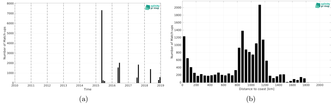
Figure 2: Number of match-ups between TSG (GOSUD-Sailing-ship) and SMAP SSS L3 v5.0 - 8-Day running (JPL) SSS as a function of time (a) and as function of the distance to coast (b) over the Gulf Stream Pi-MEP region and for the full satellite product period.
