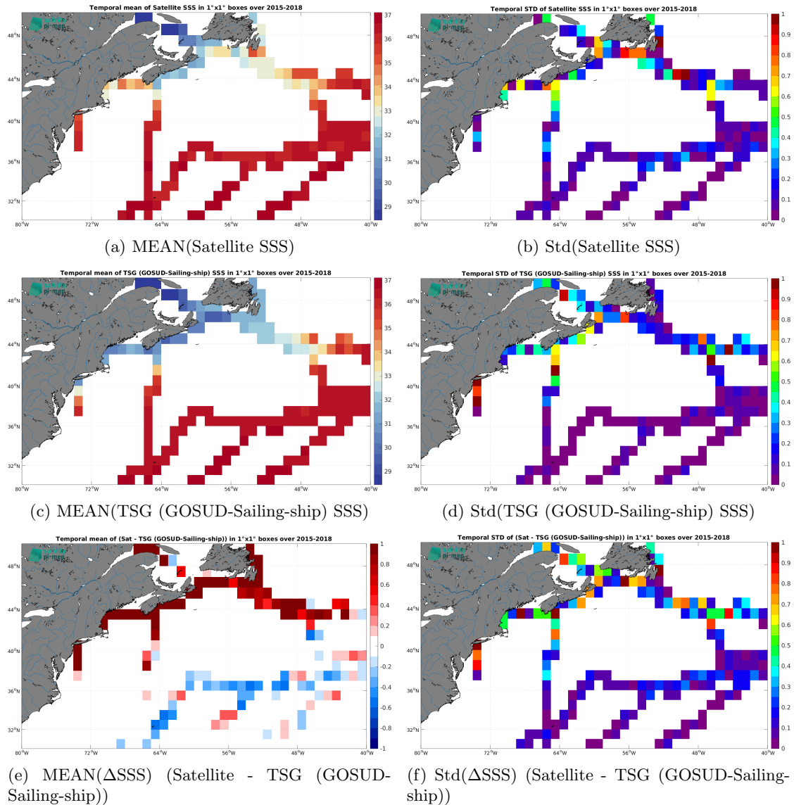
Figure 7: Temporal mean (left) and Std (right) of SSS from SMAP SSS L3 v5.0 - 8-Day running (JPL) (top), TSG (GOSUD-Sailing-ship) (middle), and of \Delta SSS (Satellite - TSG (GOSUD-Sailing-ship)). Only match-up pairs are used to generate these maps.
