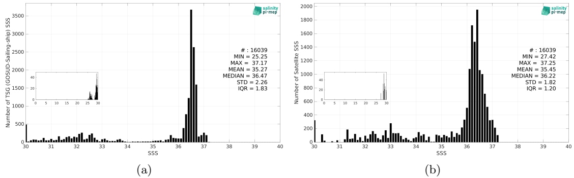
Figure 3: Histograms of SSS from TSG (GOSUD-Sailing-ship) (a) and SMAP SSS L3 v5.0 - 8-Day running (JPL) (b) considering all match-up pairs per bins of 0.1 over the Gulf Stream Pi-MEP region and for the full satellite product period.
