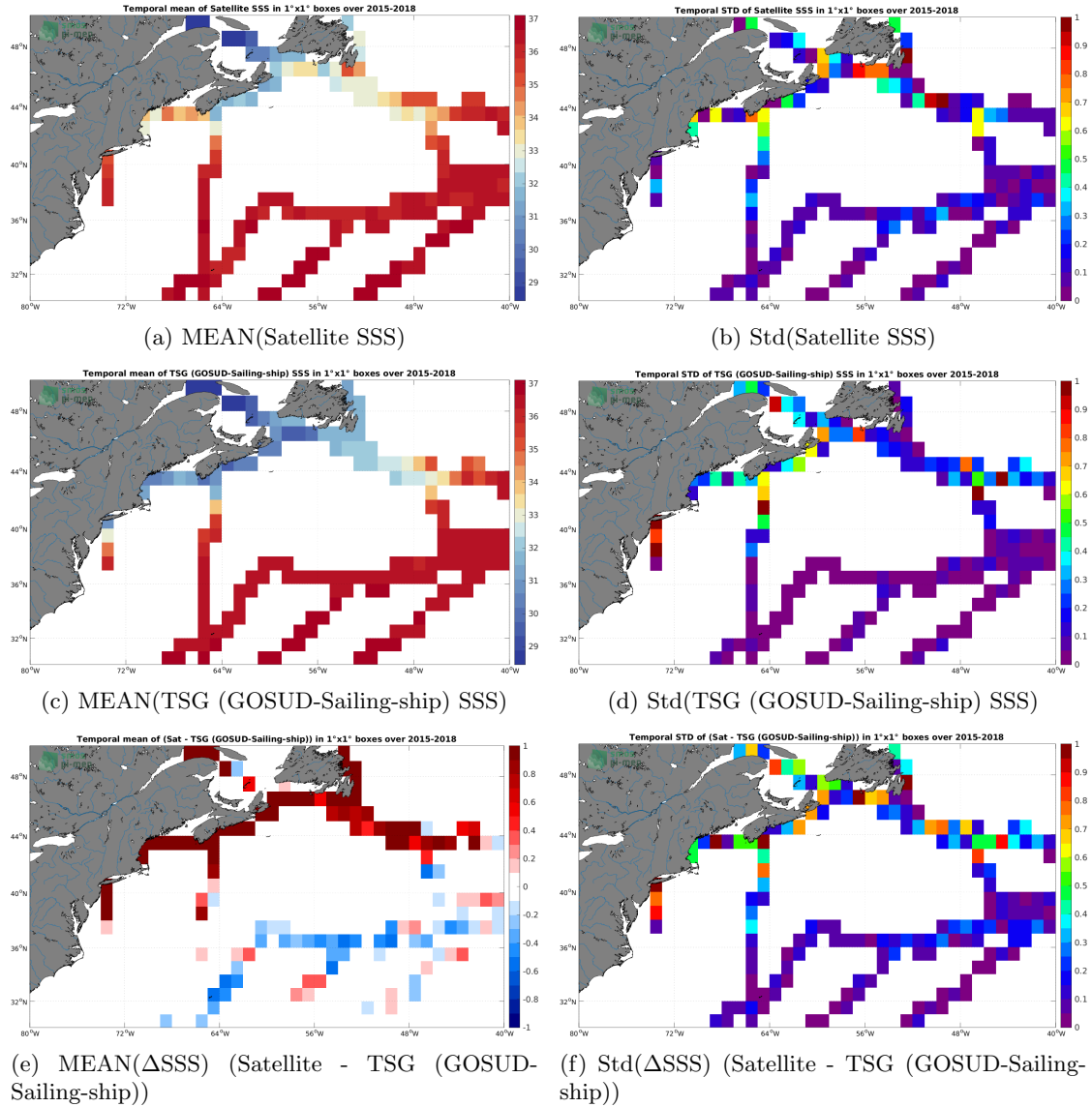
Figure 6: Temporal mean (left) and Std (right) of SSS from SMAP SSS L3 v5.0 - 8-Day running (JPL) (top), TSG (GOSUD-Sailing-ship) (middle), and of \Delta SSS (Satellite - TSG (GOSUD-Sailing-ship)). Only match-up pairs are used to generate these maps.
