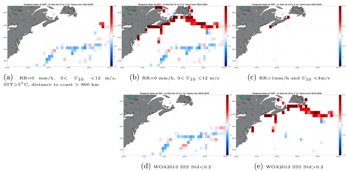
Figure 12: Temporal mean gridded over spatial boxes of size 1^\circ \times 1^\circ of \Delta SSS (SMAP SSS L3 v5.0 - 8-Day running (JPL) - TSG (GOSUD-Sailing-ship)) for 5 different subdatasets corresponding to: RR=0 mm/h, 3 < U_{10} < 12 m/s, SST > 5°C, distance to coast > 800 km (a), RR=0 mm/h, 3 < U_{10} < 12 m/s (b), RR > 1mm/h and U_{10} < 4 m/s (c), WOA2013 SSS Std < 0.2 (d), WOA2013 SSS Std > 0.2 (e).
