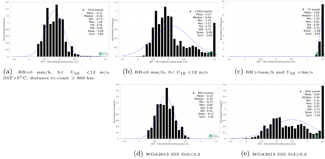
Figure 13: Normalized histogram of \Delta\text{SSS} (SMAP SSS L3 v5.0 - 8-Day running (JPL) - TSG (GOSUD-Sailing-ship)) for 5 different subdatasets corresponding to: RR=0 mm/h, 3 < U_{10} < 12 m/s, SST>5°C, distance to coast > 800 km (a), RR=0 mm/h, 3 < U_{10} < 12 m/s (b), RR>1mm/h and U_{10} < 4 m/s (c), WOA2013 SSS Std<0.2 (d), WOA2013 SSS Std>0.2 (e).
