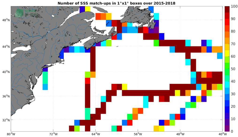
Figure 4: Number of SSS match-ups between TSG (GOSUD-Sailing-ship) SSS and the SMAP SSS L3 v5.0 - 8-Day running (JPL) SSS product for the Gulf Stream Pi-MEP region over 1^\circ \times 1^\circ boxes and for the full satellite product period.
