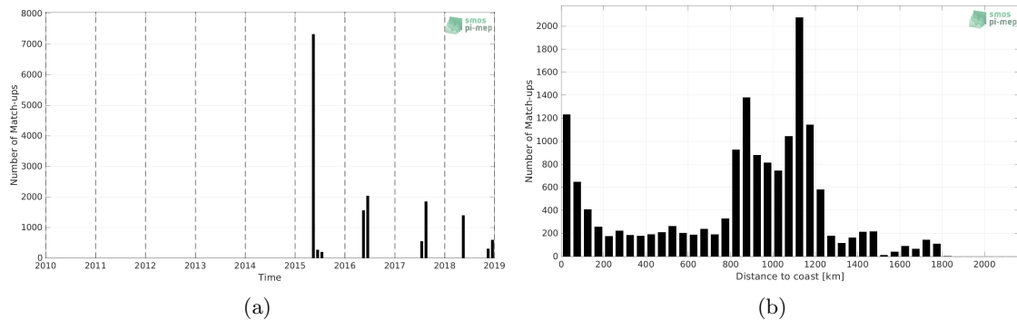
Figure 1: Number of match-ups between TSG (GOSUD-Sailing-ship) and SMAP SSS L3 v5.0 - 8-Day running (JPL) SSS as a function of time (a) and as function of the distance to coast (b) over the Gulf Stream Pi-MEP region and for the full satellite product period.
