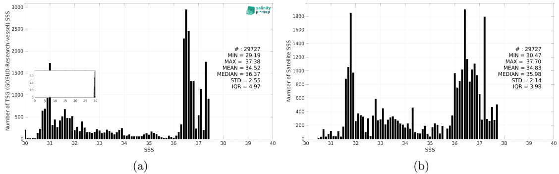
Figure 3: Histograms of SSS from TSG (GOSUD-Research-vessel) (a) and SMAP SSS L3 v5.0 - 8-Day running (JPL) (b) considering all match-up pairs per bins of 0.1 over the Gulf Stream Pi-MEP region and for the full satellite product period.
