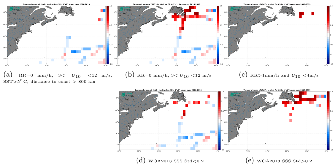
Figure 14: Temporal mean gridded over spatial boxes of size 1^\circ \times 1^\circ of \Delta SSS (SMAP SSS L3 v5.0 - 8-Day running (JPL) - TSG (GOSUD-Research-vessel)) for 5 different subdatasets corresponding to: RR=0 mm/h, 3 < U_{10} < 12 m/s, SST > 5°C, distance to coast > 800 km (a), RR=0 mm/h, 3 < U_{10} < 12 m/s (b), RR > 1mm/h and U_{10} < 4 m/s (c), WOA2013 SSS Std < 0.2 (d), WOA2013 SSS Std > 0.2 (e).
