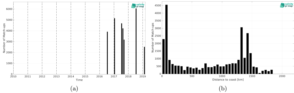
Figure 2: Number of match-ups between TSG (GOSUD-Research-vessel) and SMAP SSS L3 v5.0 - 8-Day running (JPL) SSS as a function of time (a) and as function of the distance to coast (b) over the Gulf Stream Pi-MEP region and for the full satellite product period.
