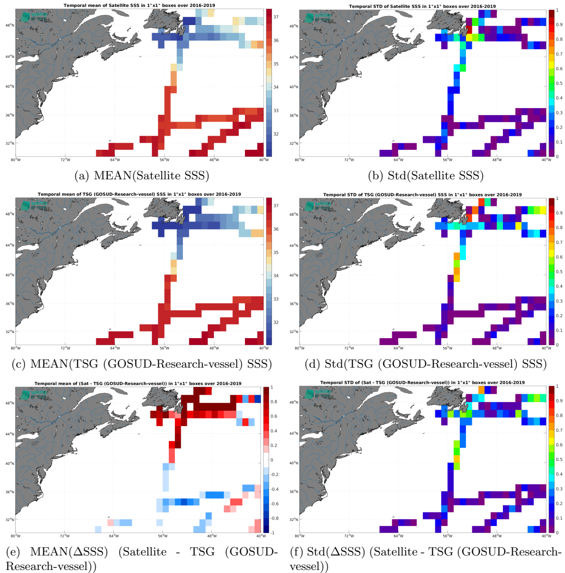
Figure 7: Temporal mean (left) and Std (right) of SSS from SMAP SSS L3 v5.0 - 8-Day running (JPL) (top), TSG (GOSUD-Research-vessel) (middle), and of \Delta SSS (Satellite - TSG (GOSUD-Research-vessel)). Only match-up pairs are used to generate these maps.
