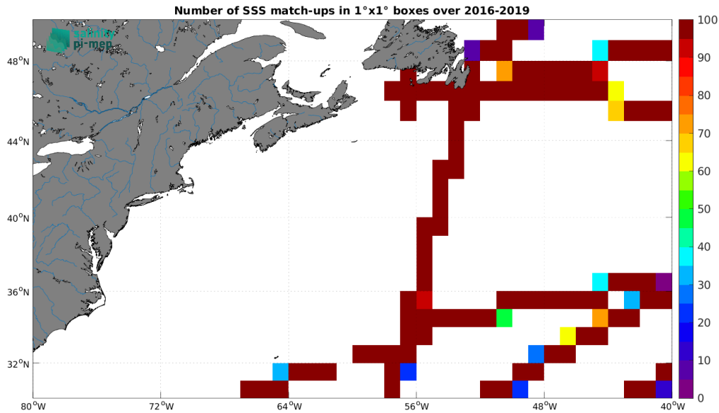
Figure 5: Number of SSS match-ups between TSG (GOSUD-Research-vessel) SSS and the SMAP SSS L3 v5.0 - 8-Day running (JPL) SSS product for the Gulf Stream Pi-MEP region over 1^\circ \times 1^\circ boxes and for the full satellite product period.
