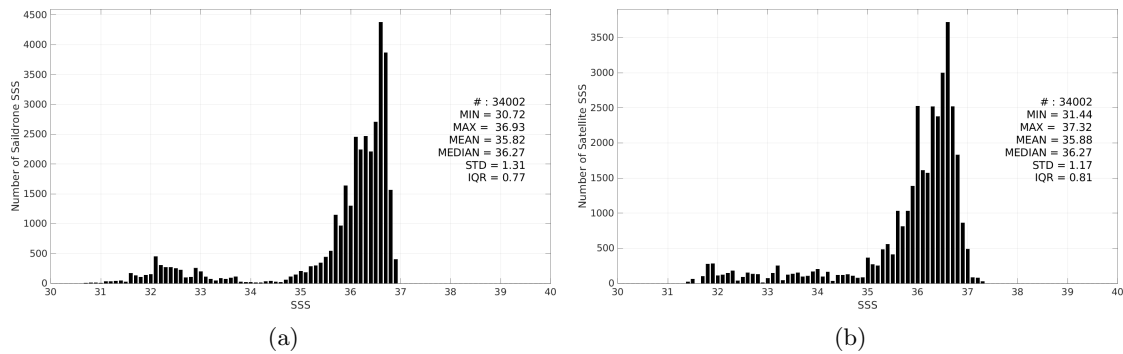
Figure 3: Histograms of SSS from Sairdrone (a) and SMAP SSS L3 v5.0 - 8-Day running (JPL) (b) considering all match-up pairs per bins of 0.1 over the Gulf Stream Pi-MEP region and for the full satellite product period.
