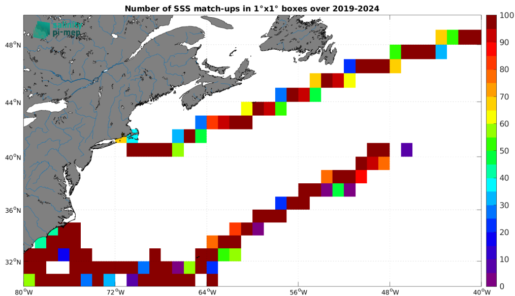
Figure 5: Number of SSS match-ups between Saildrone SSS and the SMAP SSS L3 v5.0 - 8-Day running (JPL) SSS product for the Gulf Stream Pi-MEP region over 1^\circ \times 1^\circ boxes and for the full satellite product period.
