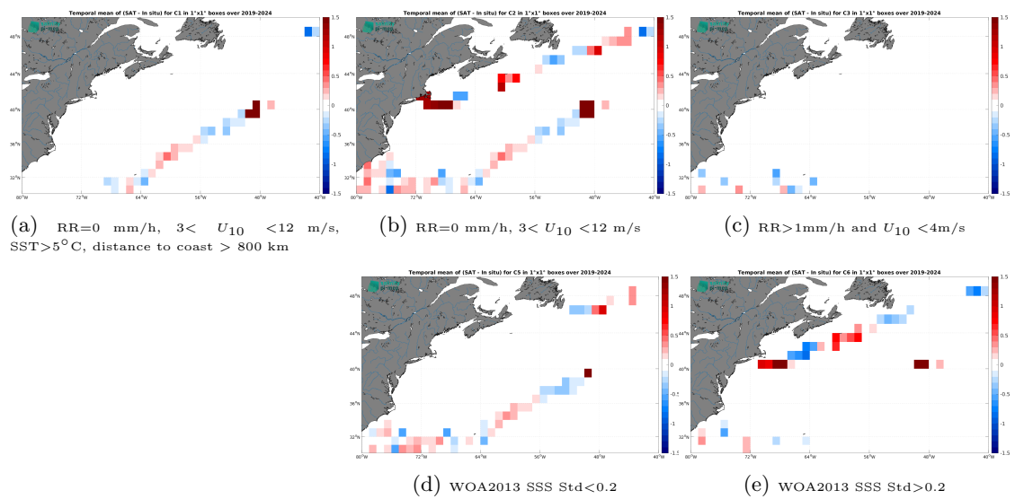
Figure 14: Temporal mean gridded over spatial boxes of size 1^\circ \times 1^\circ of \Delta SSS (SMAP SSS L3 v5.0 - 8-Day running (JPL) - Sairdrone) for 5 different subdatasets corresponding to: RR=0 mm/h, 3 < U_{10} < 12 m/s, SST > 5°C, distance to coast > 800 km (a), RR=0 mm/h, 3 < U_{10} < 12 m/s (b), RR > 1mm/h and U_{10} < 4 m/s (c), WOA2013 SSS Std < 0.2 (d), WOA2013 SSS Std > 0.2 (e).
