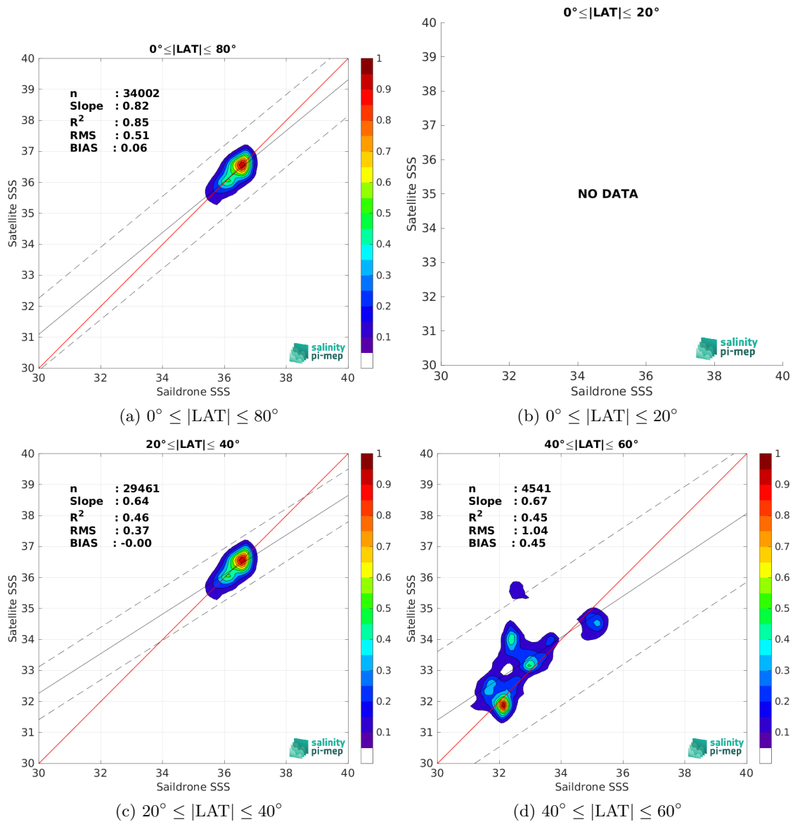
Figure 10: Contour maps of the concentration of SMAP SSS L3 v5.0 - 8-Day running (JPL) SSS (y-axis) versus Saildrone SSS (x-axis) at match-up pairs for different latitude bands. For each plot, the red line shows x=y . The black thin and dashed lines indicate a linear fit through the data cloud and the \pm 95\% confidence levels, respectively. The number match-up pairs n , the slope and R^2 coefficient of the linear fit, the root mean square (RMS) and the mean bias between satellite and in situ data are indicated for each latitude band in each plots.
