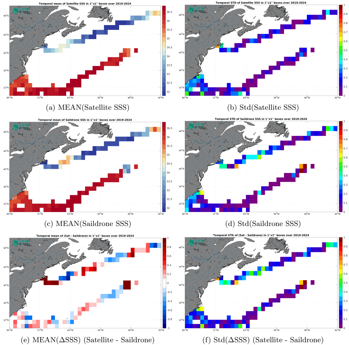
Figure 7: Temporal mean (left) and Std (right) of SSS from SMAP SSS L3 v5.0 - 8-Day running (JPL) (top), Saildrone (middle), and of \Delta SSS (Satellite - Saildrone). Only match-up pairs are used to generate these maps.
