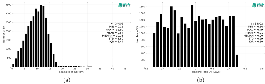
Figure 6: Histograms of the spatial (a) and temporal (b) lags between the location/time of the Sairdronne measurement and the date of the corresponding SMAP SSS L3 v5.0 - 8-Day running (JPL) SSS pixel.
