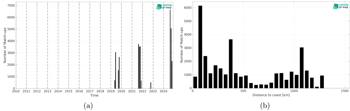
Figure 2: Number of match-ups between Sairdrone and SMAP SSS L3 v5.0 - 8-Day running (JPL) SSS as a function of time (a) and as function of the distance to coast (b) over the Gulf Stream Pi-MEP region and for the full satellite product period.
