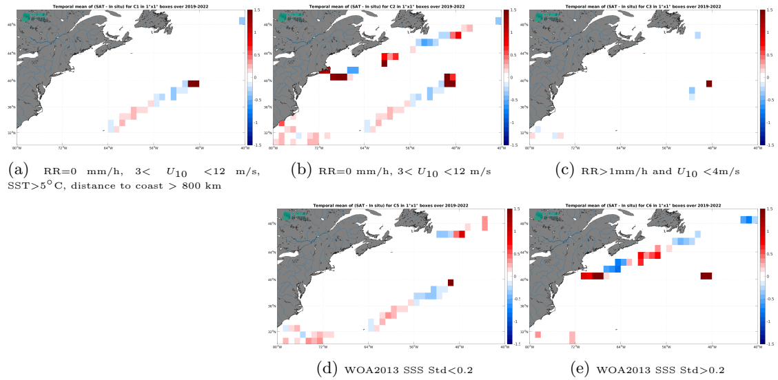
Figure 12: Temporal mean gridded over spatial boxes of size 1^\circ \times 1^\circ of \Delta SSS (SMAP SSS L3 v5.0 - 8-Day running (JPL) - Sairdrone) for 5 different subdatasets corresponding to:RR=0 mm/h, 3 < U_{10} < 12 m/s, SST >5^\circ C, distance to coast > 800 km (a), RR=0 mm/h, 3 < U_{10} < 12 m/s (b), RR >1 mm/h and U_{10} < 4 m/s (c), WOA2013 SSS Std <0.2 (d), WOA2013 SSS Std >0.2 (e).
