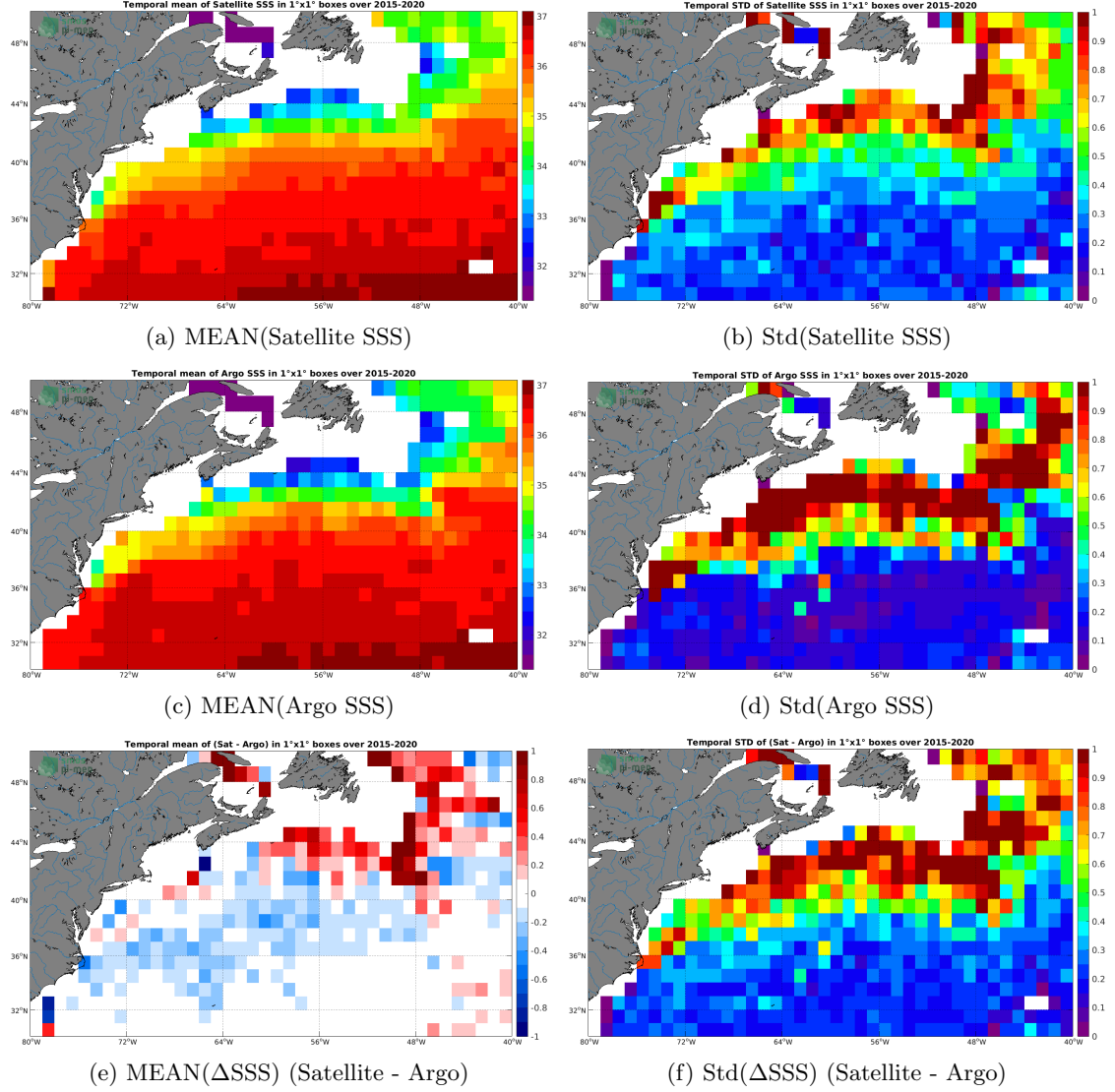
Figure 6: Temporal mean (left) and Std (right) of SSS from SMAP SSS L3 v5.0 - 8-Day running (JPL) (top), Argo (middle), and of \Delta\text{SSS} (Satellite - Argo). Only match-up pairs are used to generate these maps.
