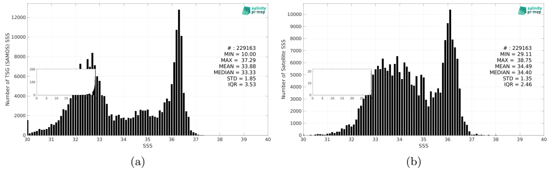
Figure 3: Histograms of SSS from TSG (SAMOS) (a) and SMAP SSS L3 v5.0 - Monthly (JPL) (b) considering all match-up pairs per bins of 0.1 over the Gulf Stream Pi-MEP region and for the full satellite product period.
