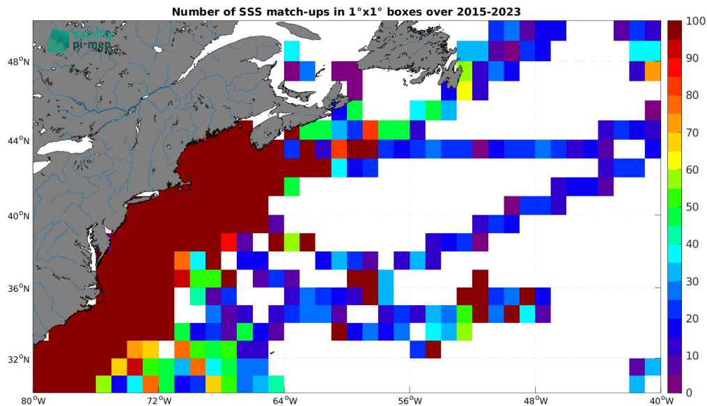
Figure 5: Number of SSS match-ups between TSG (SAMOS) SSS and the SMAP SSS L3 v5.0 - Monthly (JPL) SSS product for the Gulf Stream Pi-MEP region over 1^\circ \times 1^\circ boxes and for the full satellite product period.
