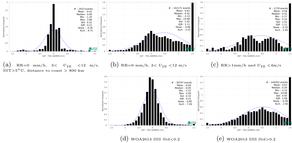
Figure 15: Normalized histogram of \Delta\text{SSS} (SMAP SSS L3 v5.0 - Monthly (JPL) - TSG (SAMOS)) for 5 different subdatasets corresponding to: RR=0 mm/h, 3 < U_{10} < 12 m/s, SST>5°C, distance to coast > 800 km (a), RR=0 mm/h, 3 < U_{10} < 12 m/s (b), RR>1mm/h and U_{10} < 4 m/s (c), WOA2013 SSS Std<0.2 (d), WOA2013 SSS Std>0.2 (e).
