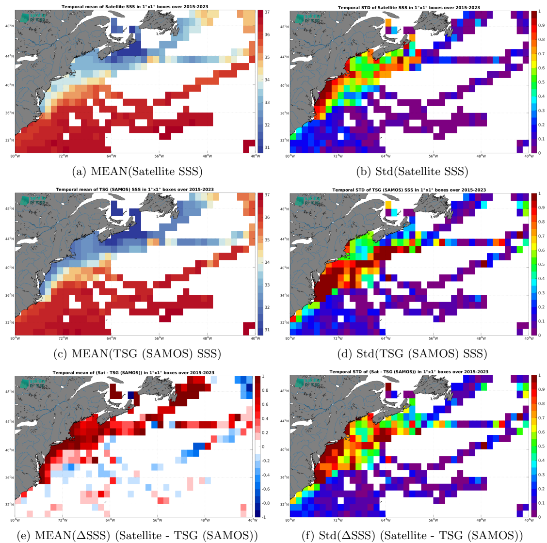
Figure 7: Temporal mean (left) and Std (right) of SSS from SMAP SSS L3 v5.0 - Monthly (JPL) (top), TSG (SAMOS) (middle), and of \Delta SSS (Satellite - TSG (SAMOS)). Only match-up pairs are used to generate these maps.
