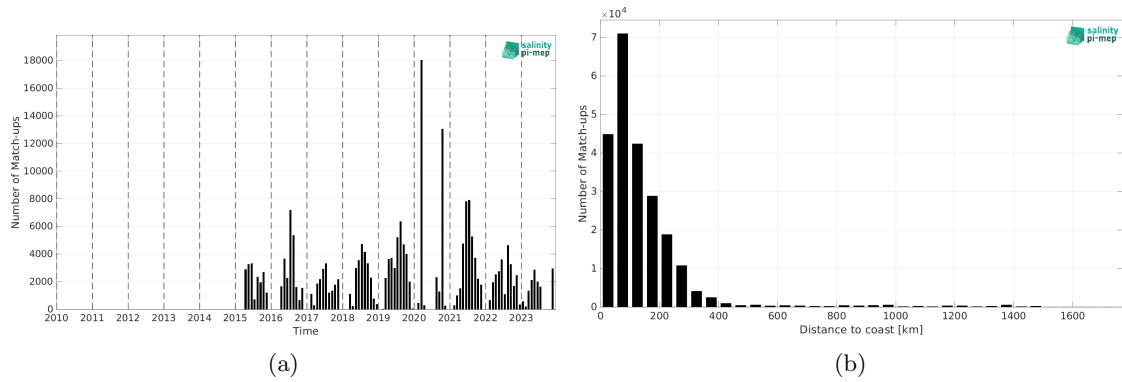
Figure 2: Number of match-ups between TSG (SAMOS) and SMAP SSS L3 v5.0 - Monthly (JPL) SSS as a function of time (a) and as function of the distance to coast (b) over the Gulf Stream Pi-MEP region and for the full satellite product period.
