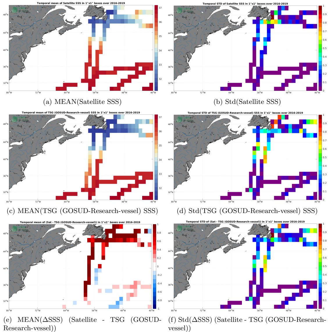
Figure 6: Temporal mean (left) and Std (right) of SSS from SMAP SSS L3 v5.0 - Monthly (JPL) (top), TSG (GOSUD-Research-vessel) (middle), and of \Delta SSS (Satellite - TSG (GOSUD-Research-vessel)). Only match-up pairs are used to generate these maps.
