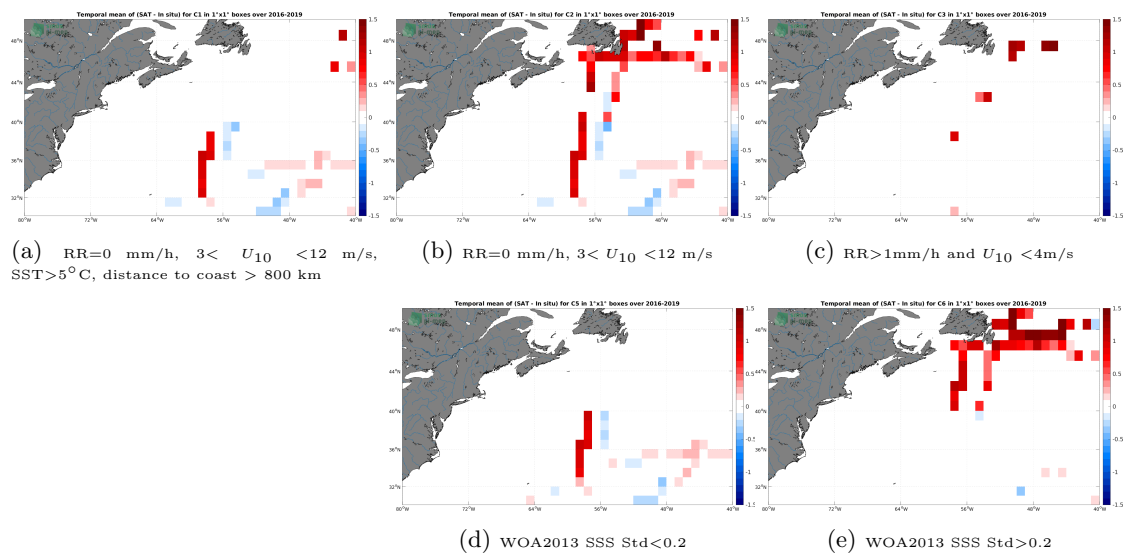
Figure 12: Temporal mean gridded over spatial boxes of size 1^\circ \times 1^\circ of \Delta SSS (SMAP SSS L3 v5.0 - Monthly (JPL) - TSG (GOSUD-Research-vessel)) for 5 different subdatasets corresponding to:RR=0 mm/h, 3 < U_{10} < 12 m/s, SST>5°C, distance to coast > 800 km (a), RR=0 mm/h, 3 < U_{10} < 12 m/s (b), RR>1mm/h and U_{10} < 4 m/s (c), WOA2013 SSS Std<0.2 (d), WOA2013 SSS Std>0.2 (e).
