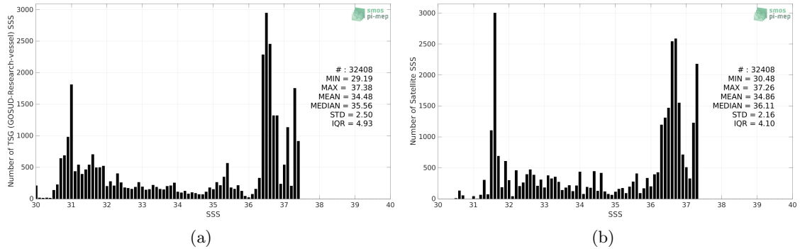
Figure 2: Histograms of SSS from TSG (GOSUD-Research-vessel) (a) and SMAP SSS L3 v5.0 - Monthly (JPL) (b) considering all match-up pairs per bins of 0.1 over the Gulf Stream Pi-MEP region and for the full satellite product period.
