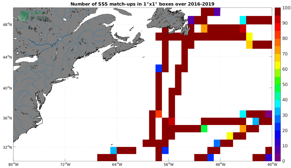
Figure 4: Number of SSS match-ups between TSG (GOSUD-Research-vessel) SSS and the SMAP SSS L3 v5.0 - Monthly (JPL) SSS product for the Gulf Stream Pi-MEP region over 1^\circ \times 1^\circ boxes and for the full satellite product period.
