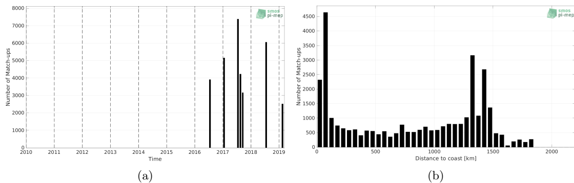
Figure 1: Number of match-ups between TSG (GOSUD-Research-vessel) and SMAP SSS L3 v5.0 - Monthly (JPL) SSS as a function of time (a) and as function of the distance to coast (b) over the Gulf Stream Pi-MEP region and for the full satellite product period.
