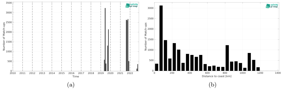
Figure 2: Number of match-ups between Sairdron and SMAP SSS L3 v5.0 - Monthly (JPL) SSS as a function of time (a) and as function of the distance to coast (b) over the Gulf Stream Pi-MEP region and for the full satellite product period.
