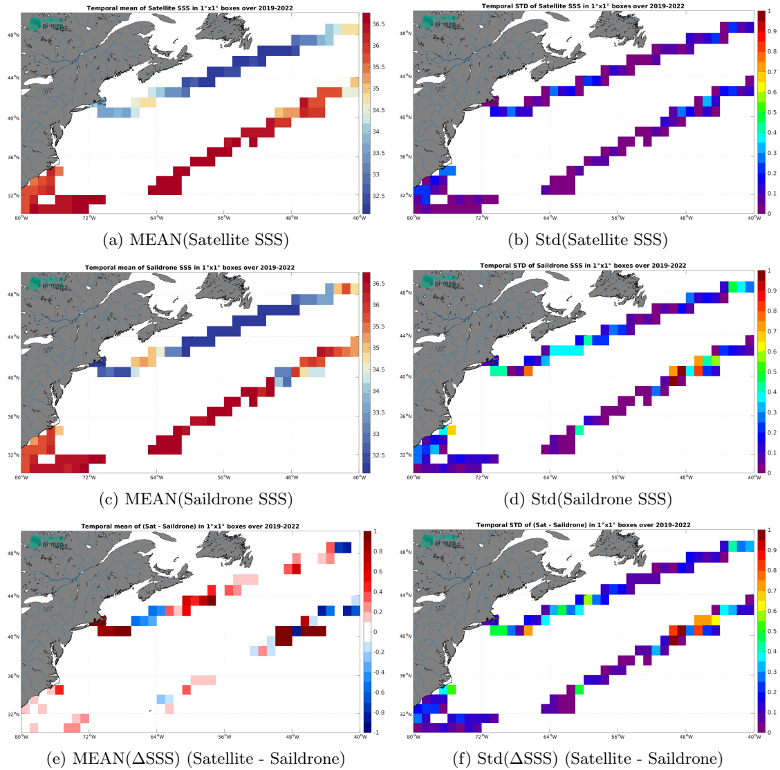
Figure 7: Temporal mean (left) and Std (right) of SSS from SMAP SSS L3 v5.0 - Monthly (JPL) (top), Saildrone (middle), and of \Delta SSS (Satellite - Saildrone). Only match-up pairs are used to generate these maps.
