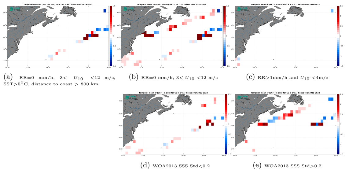
Figure 14: Temporal mean gridded over spatial boxes of size 1^\circ \times 1^\circ of \Delta SSS (SMAP SSS L3 v5.0 - Monthly (JPL) - Sairdrone) for 5 different subdatasets corresponding to:RR=0 mm/h, 3 < U_{10} < 12 m/s, SST>5°C, distance to coast > 800 km (a), RR=0 mm/h, 3 < U_{10} < 12 m/s (b), RR>1mm/h and U_{10} < 4 m/s (c), WOA2013 SSS Std<0.2 (d), WOA2013 SSS Std>0.2 (e).
