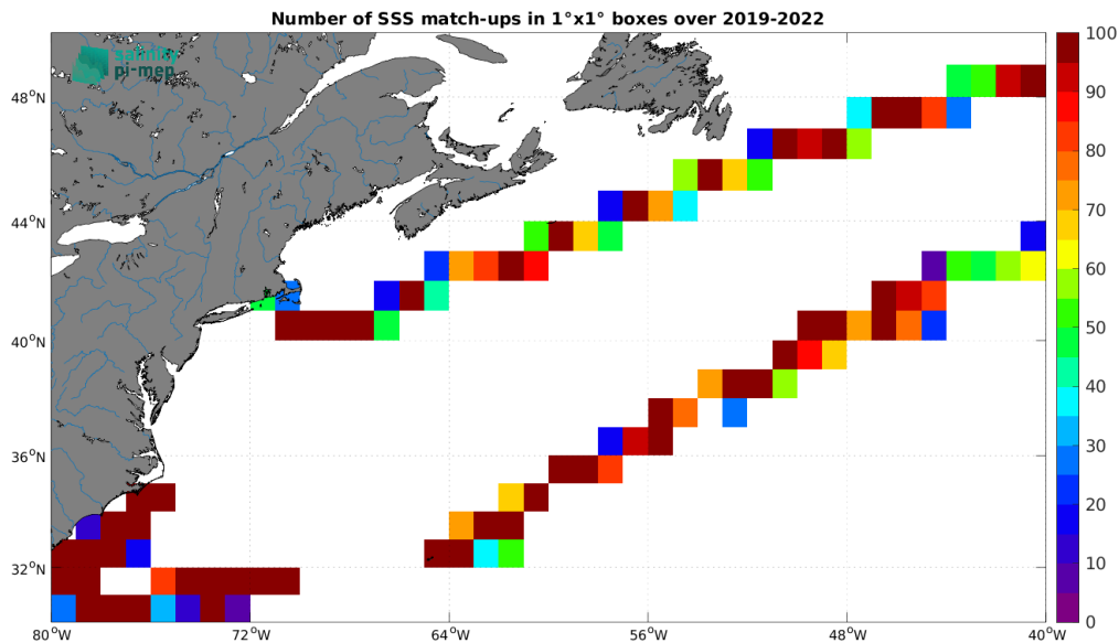
Figure 5: Number of SSS match-ups between Saildrone SSS and the SMAP SSS L3 v5.0 - Monthly (JPL) SSS product for the Gulf Stream Pi-MEP region over 1^\circ \times 1^\circ boxes and for the full satellite product period.
