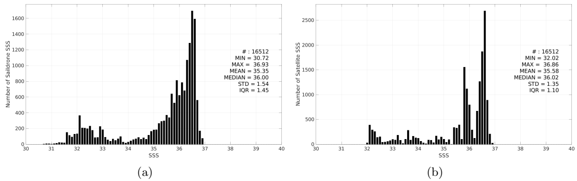
Figure 3: Histograms of SSS from Saildrone (a) and SMAP SSS L3 v5.0 - Monthly (JPL) (b) considering all match-up pairs per bins of 0.1 over the Gulf Stream Pi-MEP region and for the full satellite product period.
