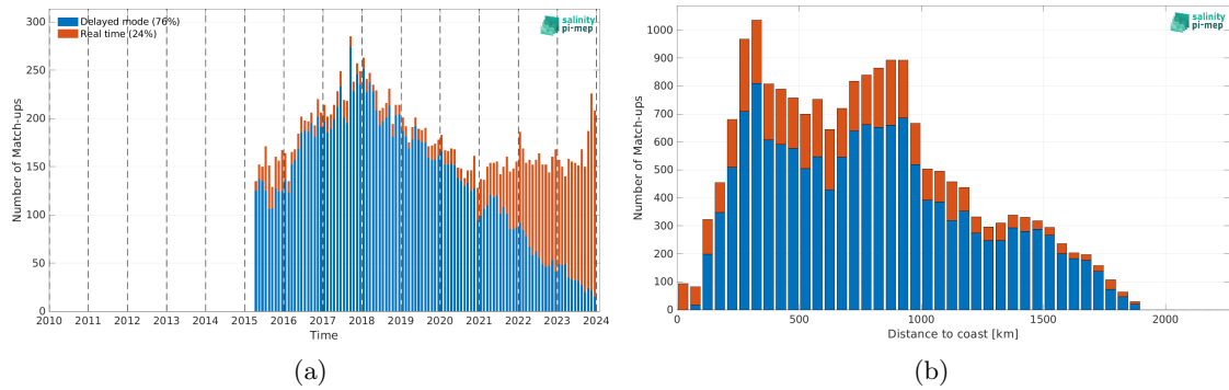
Figure 2: Number of match-ups between Argo and SMAP SSS L3 v5.0 - Monthly (JPL) SSS as a function of time (a) and as function of the distance to coast (b) over the Gulf Stream Pi-MEP region and for the full satellite product period.
