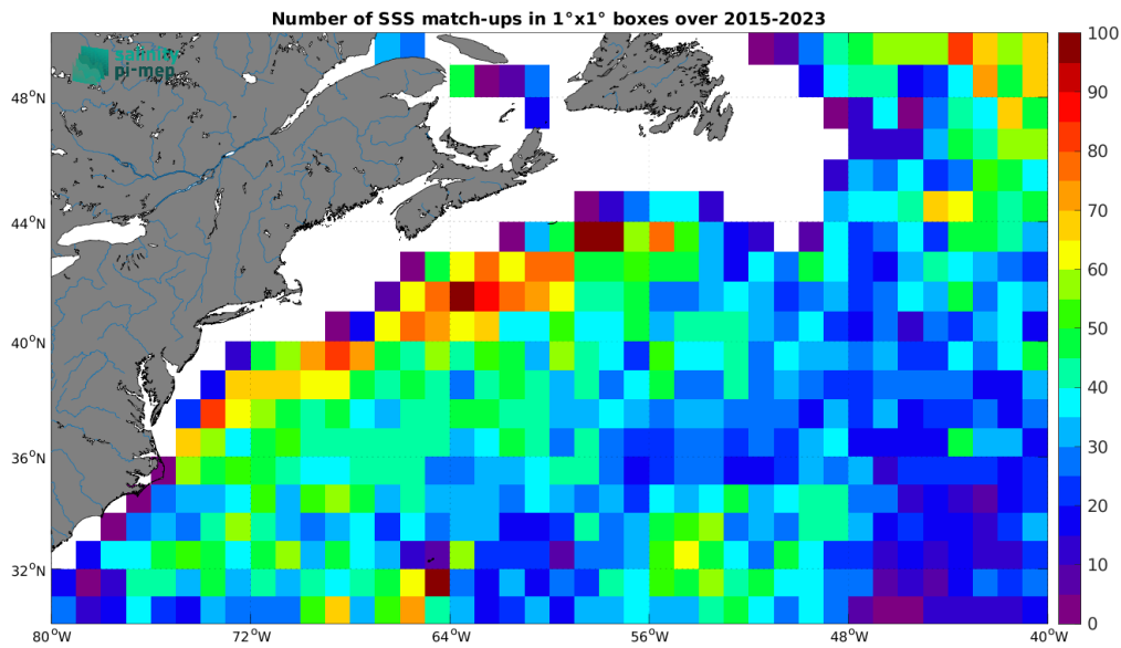
Figure 5: Number of SSS match-ups between Argo SSS and the SMAP SSS L3 v5.0 - Monthly (JPL) SSS product for the Gulf Stream Pi-MEP region over 1^\circ \times 1^\circ boxes and for the full satellite product period.
