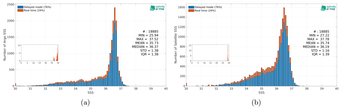
Figure 3: Histograms of SSS from Argo (a) and SMAP SSS L3 v5.0 - Monthly (JPL) (b) considering all match-up pairs per bins of 0.1 over the Gulf Stream Pi-MEP region and for the full satellite product period.
