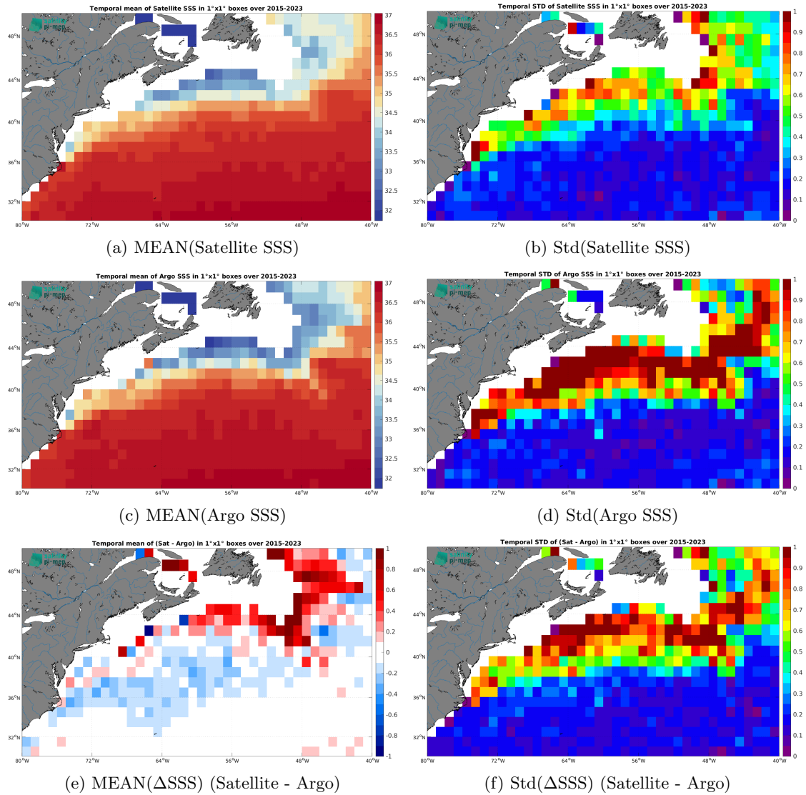
Figure 7: Temporal mean (left) and Std (right) of SSS from SMAP SSS L3 v5.0 - Monthly (JPL) (top), Argo (middle), and of \Delta SSS (Satellite - Argo). Only match-up pairs are used to generate these maps.
