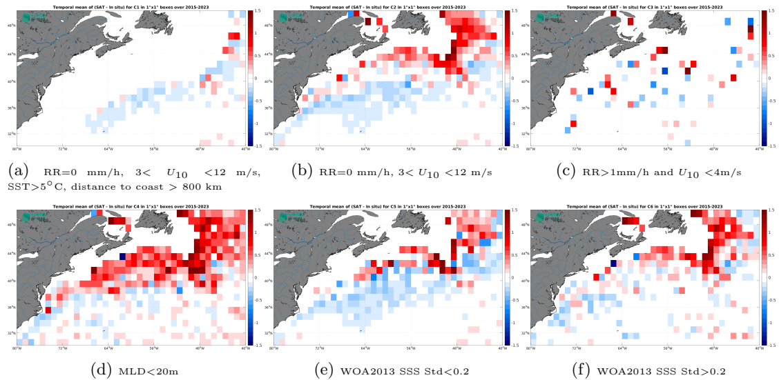
Figure 14: Temporal mean gridded over spatial boxes of size 1^\circ \times 1^\circ of \Delta SSS (SMAP SSS L3 v5.0 - Monthly (JPL) - Argo) for 6 different subdatasets corresponding to:RR=0 mm/h, 3 < U_{10} < 12 m/s, SST >5^\circ C, distance to coast > 800 km (a), RR=0 mm/h, 3 < U_{10} < 12 m/s (b), RR >1 mm/h and U_{10} < 4 m/s (c),MLD <20 m (d),WOA2013 SSS Std <0.2 (e),WOA2013 SSS Std >0.2 (f).
