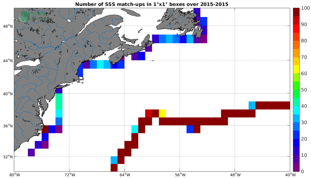
Figure 4: Number of SSS match-ups between TSG-GOSUD-Sailing-ship SSS and the SMAP-L3-JPL-V4-8DAY-RUNNING-60KM SSS product for the Gulf Stream Pi-MEP region over 1^\circ \times 1^\circ boxes and for the full satellite product period.
