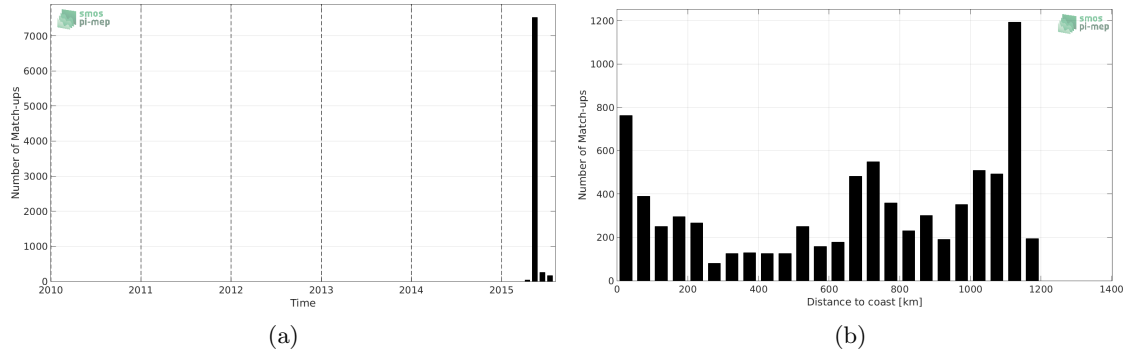
Figure 1: Number of match-ups between TSG-GOSUD-Sailing-ship and SMAP-L3-JPL-V4-8DAY-RUNNING-60KM SSS as a function of time (a) and as function of the distance to coast (b) over the Gulf Stream Pi-MEP region and for the full satellite product period.
