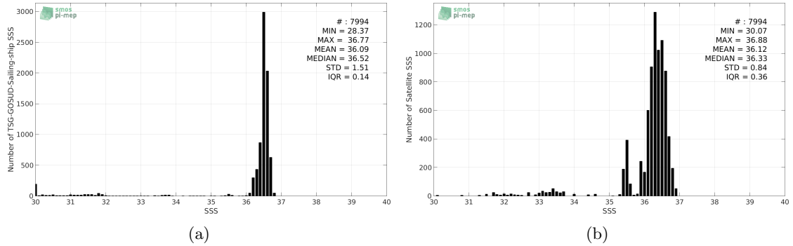
Figure 2: Histograms of SSS from TSG-GOSUD-Sailing-ship (a) and SMAP-L3-JPL-V4-8DAY-RUNNING-60KM (b) considering all match-up pairs per bins of 0.1 over the Gulf Stream Pi-MEP region and for the full satellite product period.
