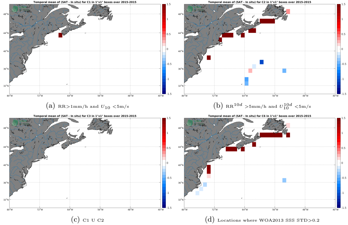
Figure 12: Temporal mean gridded over spatial boxes of size 1^\circ \times 1^\circ of \Delta SSS (SMAP-L3-JPL-V4-8DAY-RUNNING-60KM - TSG-GOSUD-Sailing-ship) for 4 different subdatasets corresponding to: RR > 1\text{mm/h} and U_{10} < 5\text{m/s} (a), RR^{10d} > 5\text{mm/h} and U_{10}^{10d} < 5\text{m/s} (b), C1 U C2 (c), Locations where WOA2013 SSS STD > 0.2 (d).
