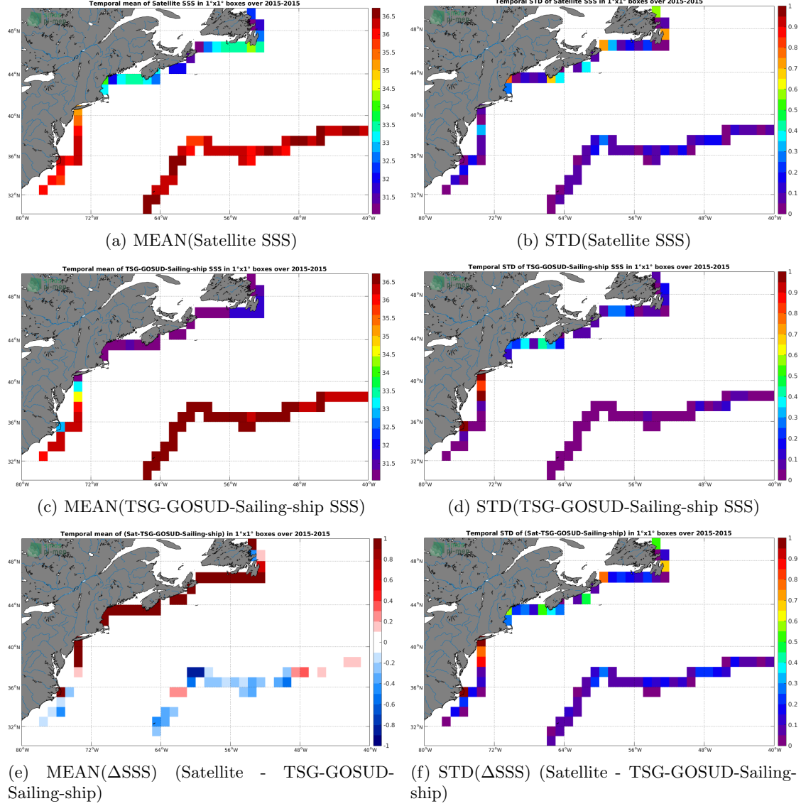
Figure 6: Temporal mean (left) and STD (right) of SSS from SMAP-L3-JPL-V4-8DAY-RUNNING-60KM (top), TSG-GOSUD-Sailing-ship (middle), and of \Delta SSS (Satellite - TSG-GOSUD-Sailing-ship). Only match-up pairs are used to generate these maps.
