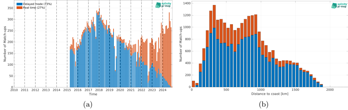
Figure 2: Number of match-ups between Argo and SMAP SSS L2-AVERAGED v6 (RSS) SSS as a function of time (a) and as function of the distance to coast (b) over the Gulf Stream Pi-MEP region and for the full satellite product period.
