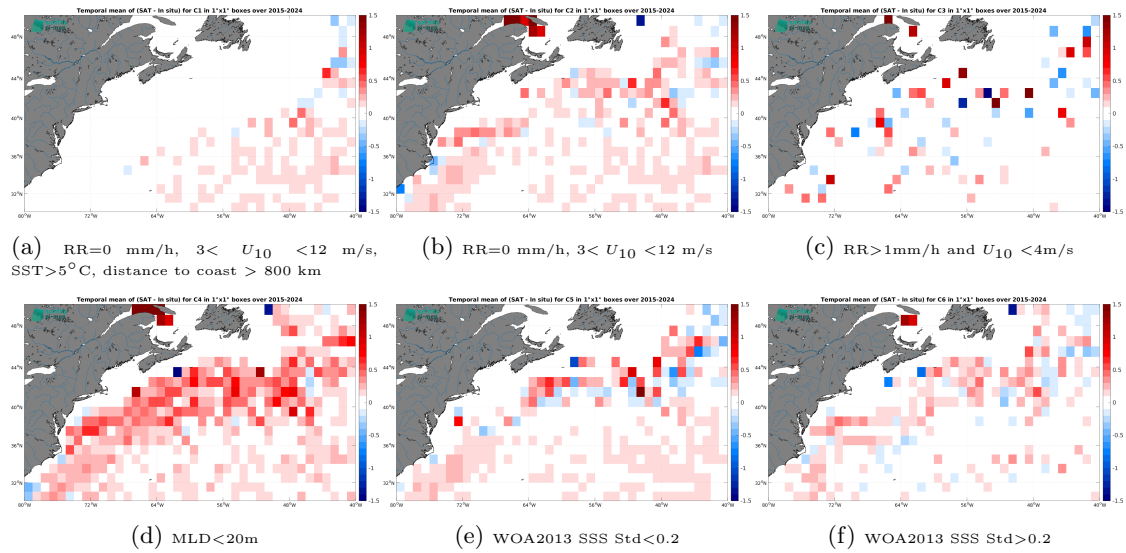
Figure 14: Temporal mean gridded over spatial boxes of size 1^\circ \times 1^\circ of \Delta SSS (SMAP SSS L2-AVERAGED v6 (RSS) - Argo) for 6 different subdatasets corresponding to:RR=0 mm/h, 3 < U_{10} < 12 m/s, SST >5^\circ C, distance to coast > 800 km (a), RR=0 mm/h, 3 < U_{10} < 12 m/s (b), RR >1 mm/h and U_{10} < 4 m/s (c),MLD <20 m (d),WOA2013 SSS Std <0.2 (e),WOA2013 SSS Std >0.2 (f).
