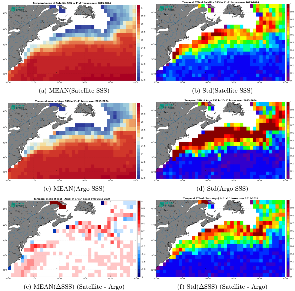
Figure 7: Temporal mean (left) and Std (right) of SSS from SMAP SSS L2-AVERAGED v6 (RSS) (top), Argo (middle), and of \Delta SSS (Satellite - Argo). Only match-up pairs are used to generate these maps.
