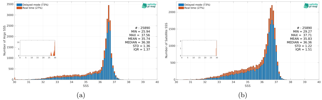
Figure 3: Histograms of SSS from Argo (a) and SMAP SSS L2-AVERAGED v6 (RSS) (b) considering all match-up pairs per bins of 0.1 over the Gulf Stream Pi-MEP region and for the full satellite product period.
