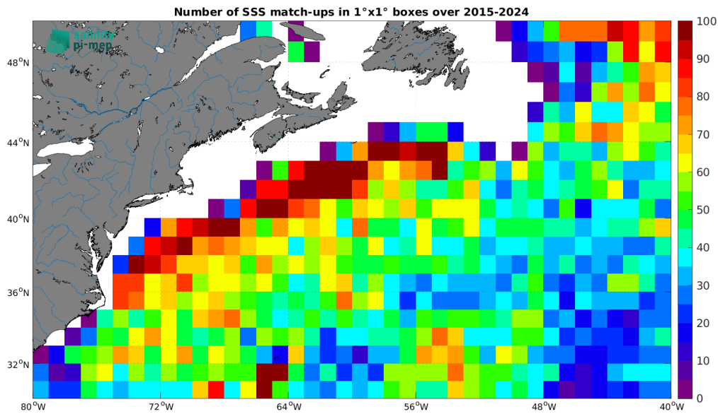
Figure 5: Number of SSS match-ups between Argo SSS and the SMAP SSS L2-AVERAGED v6 (RSS) SSS product for the Gulf Stream Pi-MEP region over 1^\circ \times 1^\circ boxes and for the full satellite product period.
