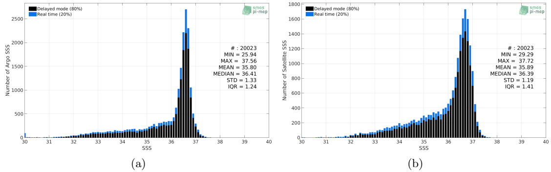
Figure 2: Histograms of SSS from Argo (a) and SMAP SSS L2-AVERAGED v5 (RSS) (b) considering all match-up pairs per bins of 0.1 over the Gulf Stream Pi-MEP region and for the full satellite product period.
