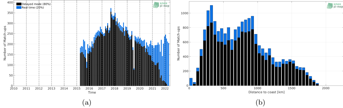
Figure 1: Number of match-ups between Argo and SMAP SSS L2-AVERAGED v5 (RSS) SSS as a function of time (a) and as function of the distance to coast (b) over the Gulf Stream Pi-MEP region and for the full satellite product period.
