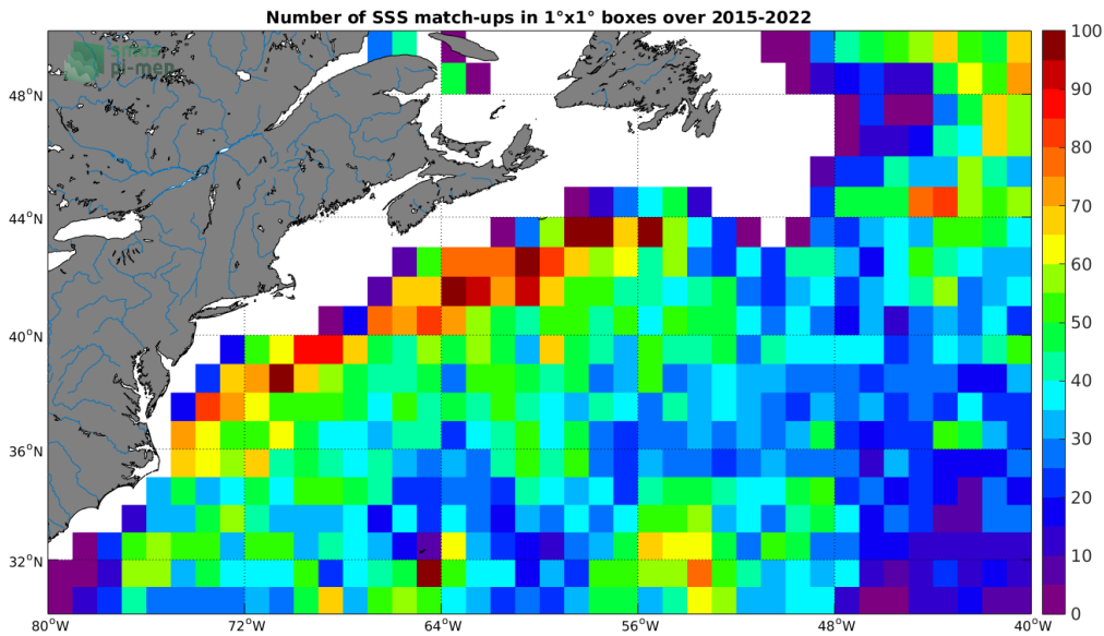
Figure 4: Number of SSS match-ups between Argo SSS and the SMAP SSS L2-AVERAGED v5 (RSS) SSS product for the Gulf Stream Pi-MEP region over 1^\circ \times 1^\circ boxes and for the full satellite product period.
