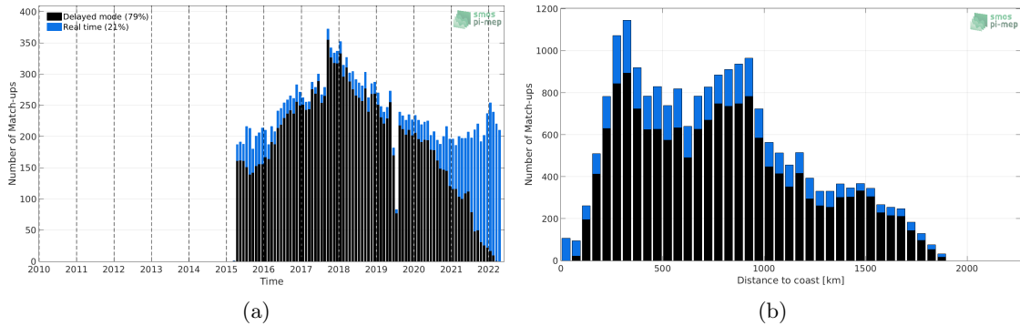
Figure 1: Number of match-ups between Argo and SMAP SSS L2-AVERAGED v5.0 (JPL) SSS as a function of time (a) and as function of the distance to coast (b) over the Gulf Stream Pi-MEP region and for the full satellite product period.
