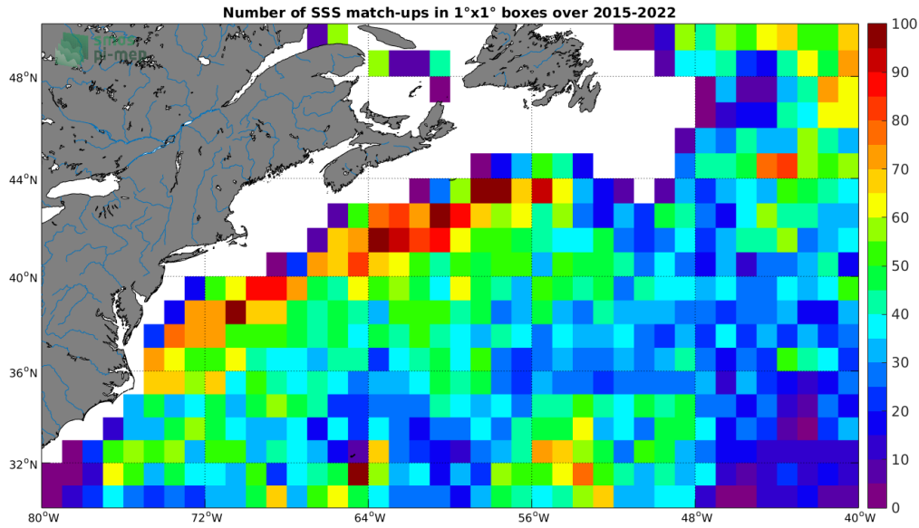
Figure 4: Number of SSS match-ups between Argo SSS and the SMAP SSS L2-AVERAGED v5.0 (JPL) SSS product for the Gulf Stream Pi-MEP region over 1^\circ \times 1^\circ boxes and for the full satellite product period.
