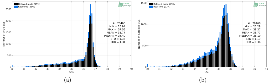
Figure 2: Histograms of SSS from Argo (a) and SMAP SSS L2-AVERAGED v5.0 (JPL) (b) considering all match-up pairs per bins of 0.1 over the Gulf Stream Pi-MEP region and for the full satellite product period.
