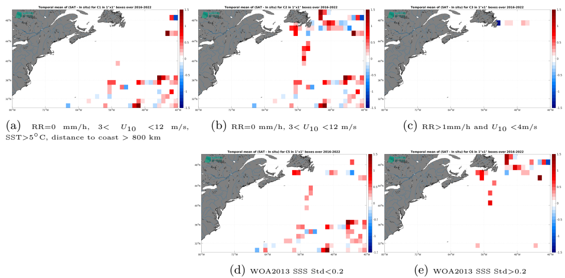
Figure 14: Temporal mean gridded over spatial boxes of size 1^\circ \times 1^\circ of \Delta SSS (SMAP SSS L2 v6 (RSS) - TSG (GOSUD-Research-vessel)) for 5 different subdatasets corresponding to:RR=0 mm/h, 3 < U_{10} < 12 m/s, SST > 5°C, distance to coast > 800 km (a), RR=0 mm/h, 3 < U_{10} < 12 m/s (b), RR > 1mm/h and U_{10} < 4 m/s (c), WOA2013 SSS Std < 0.2 (d), WOA2013 SSS Std > 0.2 (e).
