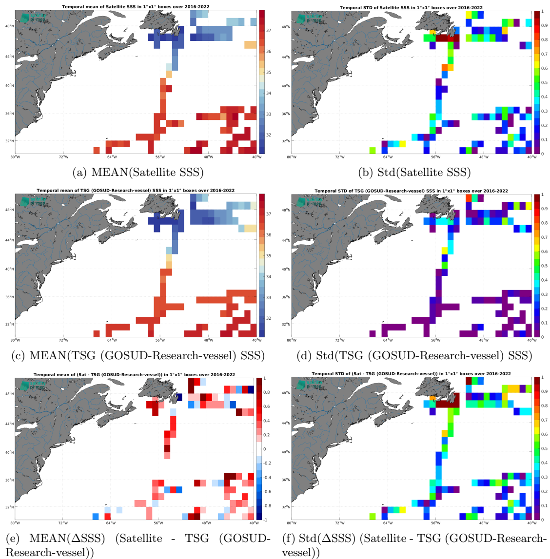
Figure 7: Temporal mean (left) and Std (right) of SSS from SMAP SSS L2 v6 (RSS) (top), TSG (GOSUD-Research-vessel) (middle), and of \Delta SSS (Satellite - TSG (GOSUD-Research-vessel)). Only match-up pairs are used to generate these maps.
