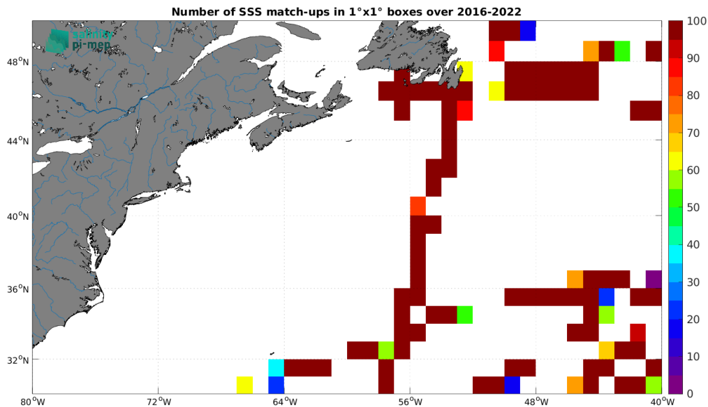
Figure 5: Number of SSS match-ups between TSG (GOSUD-Research-vessel) SSS and the SMAP SSS L2 v6 (RSS) SSS product for the Gulf Stream Pi-MEP region over 1^\circ \times 1^\circ boxes and for the full satellite product period.
