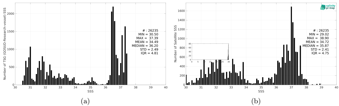
Figure 3: Histograms of SSS from TSG (GOSUD-Research-vessel) (a) and SMAP SSS L2 v6 (RSS) (b) considering all match-up pairs per bins of 0.1 over the Gulf Stream Pi-MEP region and for the full satellite product period.
