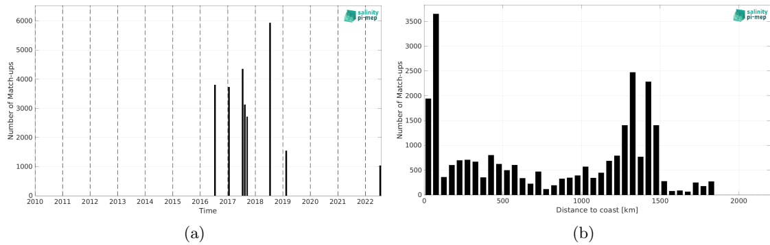
Figure 2: Number of match-ups between TSG (GOSUD-Research-vessel) and SMAP SSS L2 v6 (RSS) SSS as a function of time (a) and as function of the distance to coast (b) over the Gulf Stream Pi-MEP region and for the full satellite product period.
