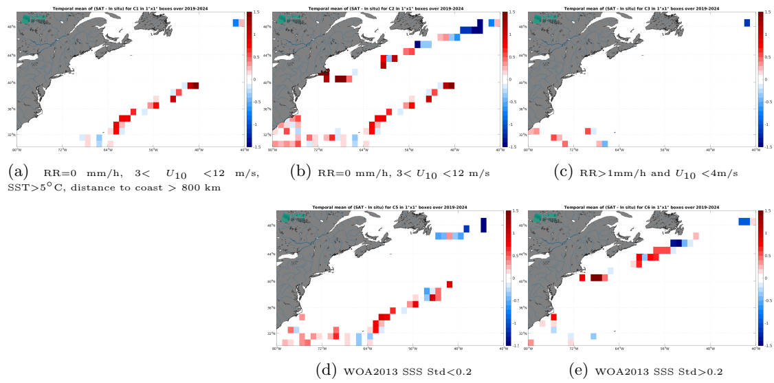
Figure 14: Temporal mean gridded over spatial boxes of size 1^\circ \times 1^\circ of \Delta SSS (SMAP SSS L2 v6 (RSS) - Saifdrone) for 5 different subdatasets corresponding to: RR=0 mm/h, 3 < U_{10} < 12 m/s, SST > 5°C, distance to coast > 800 km (a), RR=0 mm/h, 3 < U_{10} < 12 m/s (b), RR > 1mm/h and U_{10} < 4 m/s (c), WOA2013 SSS Std < 0.2 (d), WOA2013 SSS Std > 0.2 (e).
