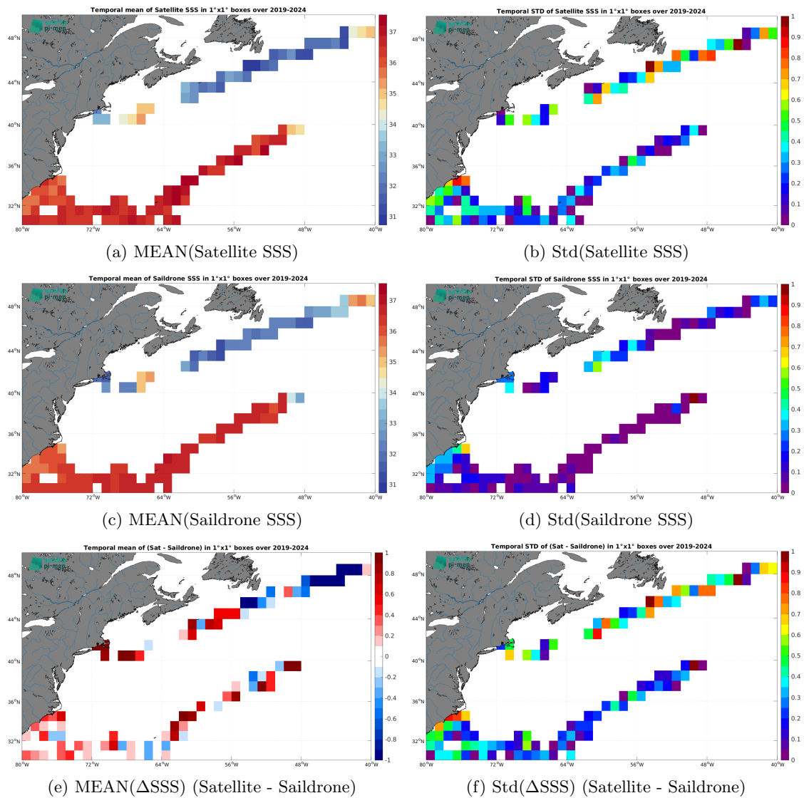
Figure 7: Temporal mean (left) and Std (right) of SSS from SMAP SSS L2 v6 (RSS) (top), Saildrone (middle), and of \Delta SSS (Satellite - Saildrone). Only match-up pairs are used to generate these maps.
