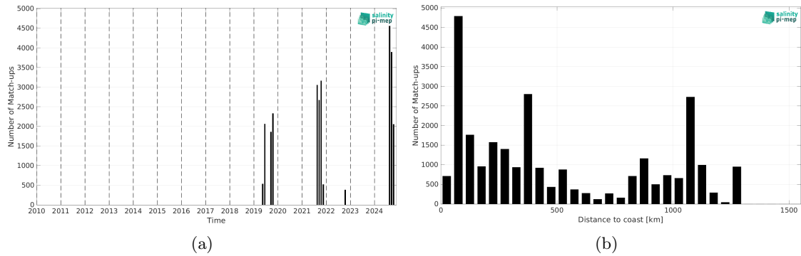
Figure 2: Number of match-ups between Saildrone and SMAP SSS L2 v6 (RSS) SSS as a function of time (a) and as function of the distance to coast (b) over the Gulf Stream Pi-MEP region and for the full satellite product period.
