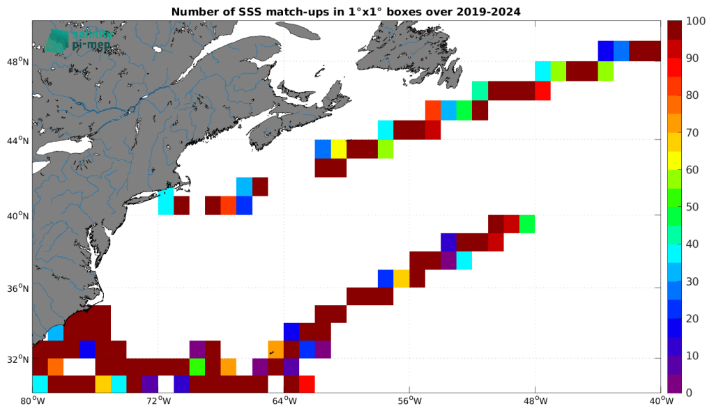
Figure 5: Number of SSS match-ups between Saildrone SSS and the SMAP SSS L2 v6 (RSS) SSS product for the Gulf Stream Pi-MEP region over 1^\circ \times 1^\circ boxes and for the full satellite product period.
