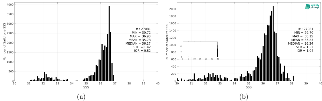
Figure 3: Histograms of SSS from Saildrone (a) and SMAP SSS L2 v6 (RSS) (b) considering all match-up pairs per bins of 0.1 over the Gulf Stream Pi-MEP region and for the full satellite product period.
