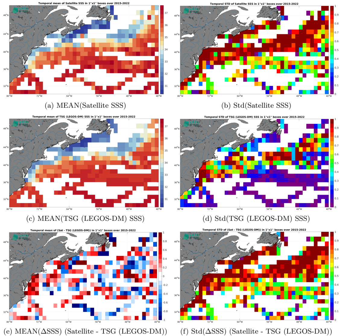
Figure 7: Temporal mean (left) and Std (right) of SSS from SMAP SSS L2 v6 - 40 km (RSS) (top), TSG (LEGOS-DM) (middle), and of \Delta SSS (Satellite - TSG (LEGOS-DM)). Only match-up pairs are used to generate these maps.
