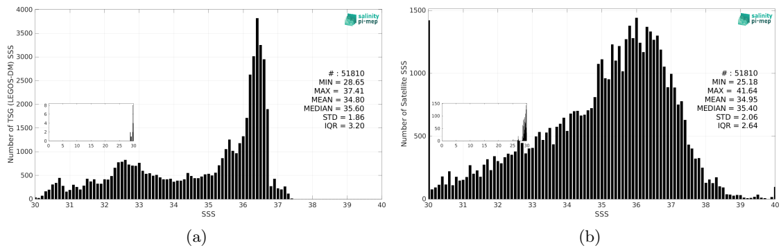
Figure 3: Histograms of SSS from TSG (LEGOS-DM) (a) and SMAP SSS L2 v6 - 40 km (RSS) (b) considering all match-up pairs per bins of 0.1 over the Gulf Stream Pi-MEP region and for the full satellite product period.
