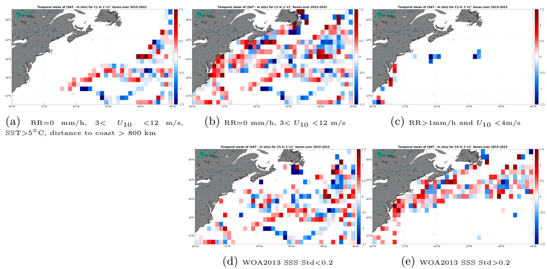
Figure 14: Temporal mean gridded over spatial boxes of size 1^\circ \times 1^\circ of \Delta SSS (SMAP SSS L2 v6 - 40 km (RSS) - TSG (LEGOS-DM)) for 5 different subdatasets corresponding to: RR=0 mm/h, 3 < U_{10} < 12 m/s, SST > 5°C, distance to coast > 800 km (a), RR=0 mm/h, 3 < U_{10} < 12 m/s (b), RR > 1mm/h and U_{10} < 4 m/s (c), WOA2013 SSS Std < 0.2 (d), WOA2013 SSS Std > 0.2 (e).
