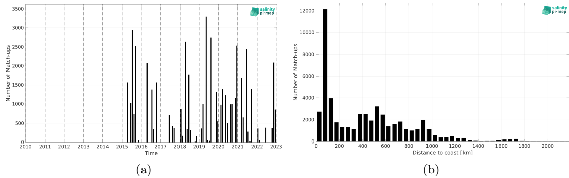
Figure 2: Number of match-ups between TSG (LEGOS-DM) and SMAP SSS L2 v6 - 40 km (RSS) SSS as a function of time (a) and as function of the distance to coast (b) over the Gulf Stream Pi-MEP region and for the full satellite product period.
