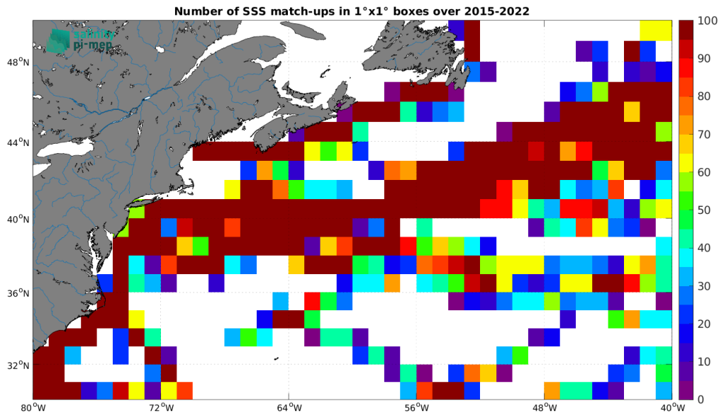
Figure 5: Number of SSS match-ups between TSG (LEGOS-DM) SSS and the SMAP SSS L2 v6 - 40 km (RSS) SSS product for the Gulf Stream Pi-MEP region over 1^\circ \times 1^\circ boxes and for the full satellite product period.
