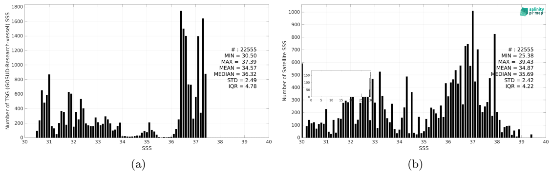
Figure 3: Histograms of SSS from TSG (GOSUD-Research-vessel) (a) and SMAP SSS L2 v6 - 40 km (RSS) (b) considering all match-up pairs per bins of 0.1 over the Gulf Stream Pi-MEP region and for the full satellite product period.
