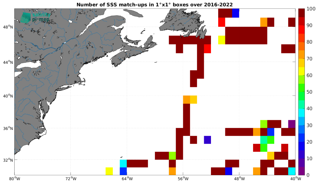
Figure 5: Number of SSS match-ups between TSG (GOSUD-Research-vessel) SSS and the SMAP SSS L2 v6 - 40 km (RSS) SSS product for the Gulf Stream Pi-MEP region over 1^\circ \times 1^\circ boxes and for the full satellite product period.
