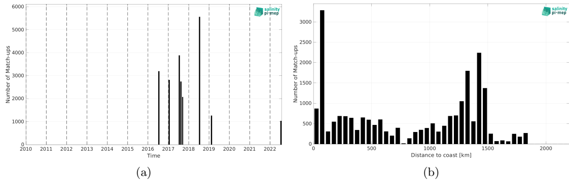
Figure 2: Number of match-ups between TSG (GOSUD-Research-vessel) and SMAP SSS L2 v6 - 40 km (RSS) SSS as a function of time (a) and as function of the distance to coast (b) over the Gulf Stream Pi-MEP region and for the full satellite product period.
