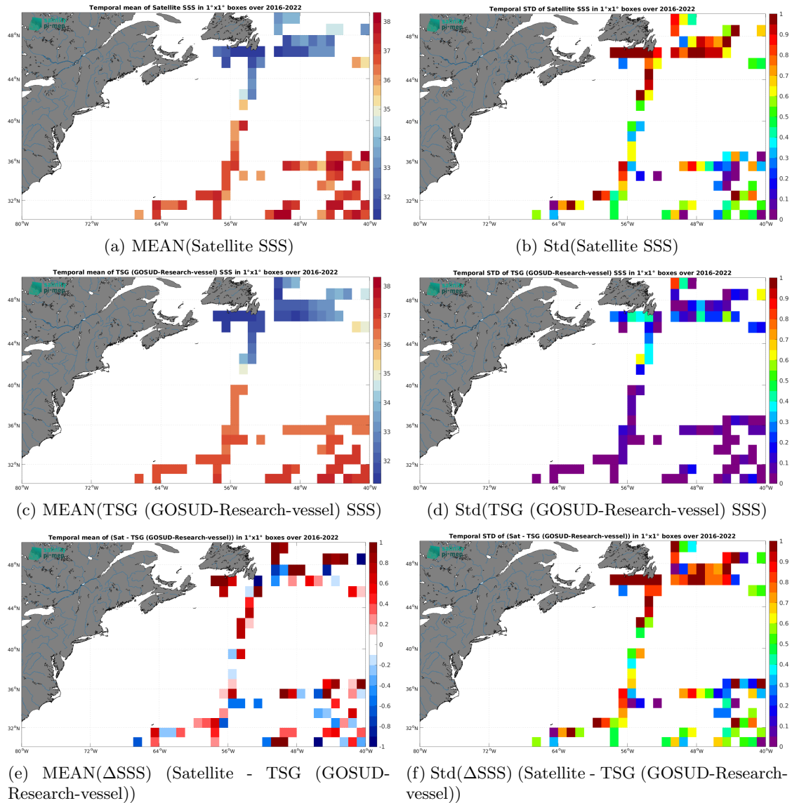
Figure 7: Temporal mean (left) and Std (right) of SSS from SMAP SSS L2 v6 - 40 km (RSS) (top), TSG (GOSUD-Research-vessel) (middle), and of \Delta SSS (Satellite - TSG (GOSUD-Research-vessel)). Only match-up pairs are used to generate these maps.
