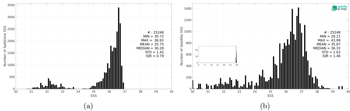
Figure 3: Histograms of SSS from Sairdrone (a) and SMAP SSS L2 v6 - 40 km (RSS) (b) considering all match-up pairs per bins of 0.1 over the Gulf Stream Pi-MEP region and for the full satellite product period.
