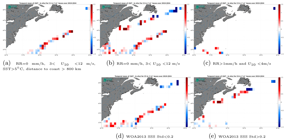
Figure 14: Temporal mean gridded over spatial boxes of size 1^\circ \times 1^\circ of \Delta SSS (SMAP SSS L2 v6 - 40 km (RSS) - Sairdrone) for 5 different subdatasets corresponding to:RR=0 mm/h, 3 < U_{10} < 12 m/s, SST>5°C, distance to coast > 800 km (a), RR=0 mm/h, 3 < U_{10} < 12 m/s (b), RR>1mm/h and U_{10} < 4 m/s (c), WOA2013 SSS Std<0.2 (d), WOA2013 SSS Std>0.2 (e).
