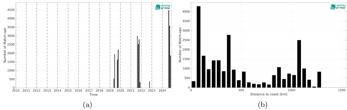
Figure 2: Number of match-ups between Sairdrone and SMAP SSS L2 v6 - 40 km (RSS) SSS as a function of time (a) and as function of the distance to coast (b) over the Gulf Stream Pi-MEP region and for the full satellite product period.
