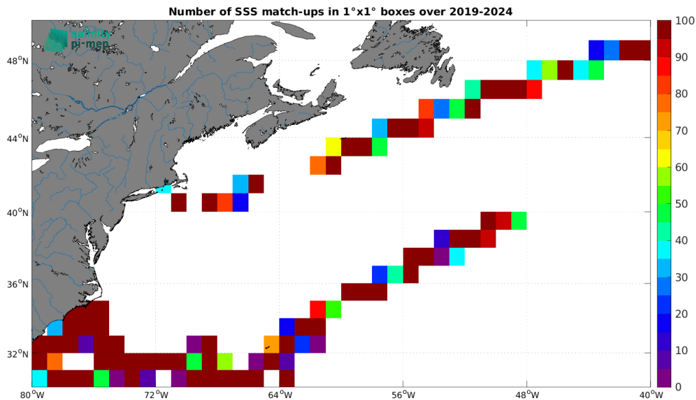
Figure 5: Number of SSS match-ups between Saildrone SSS and the SMAP SSS L2 v6 - 40 km (RSS) SSS product for the Gulf Stream Pi-MEP region over 1^\circ \times 1^\circ boxes and for the full satellite product period.
