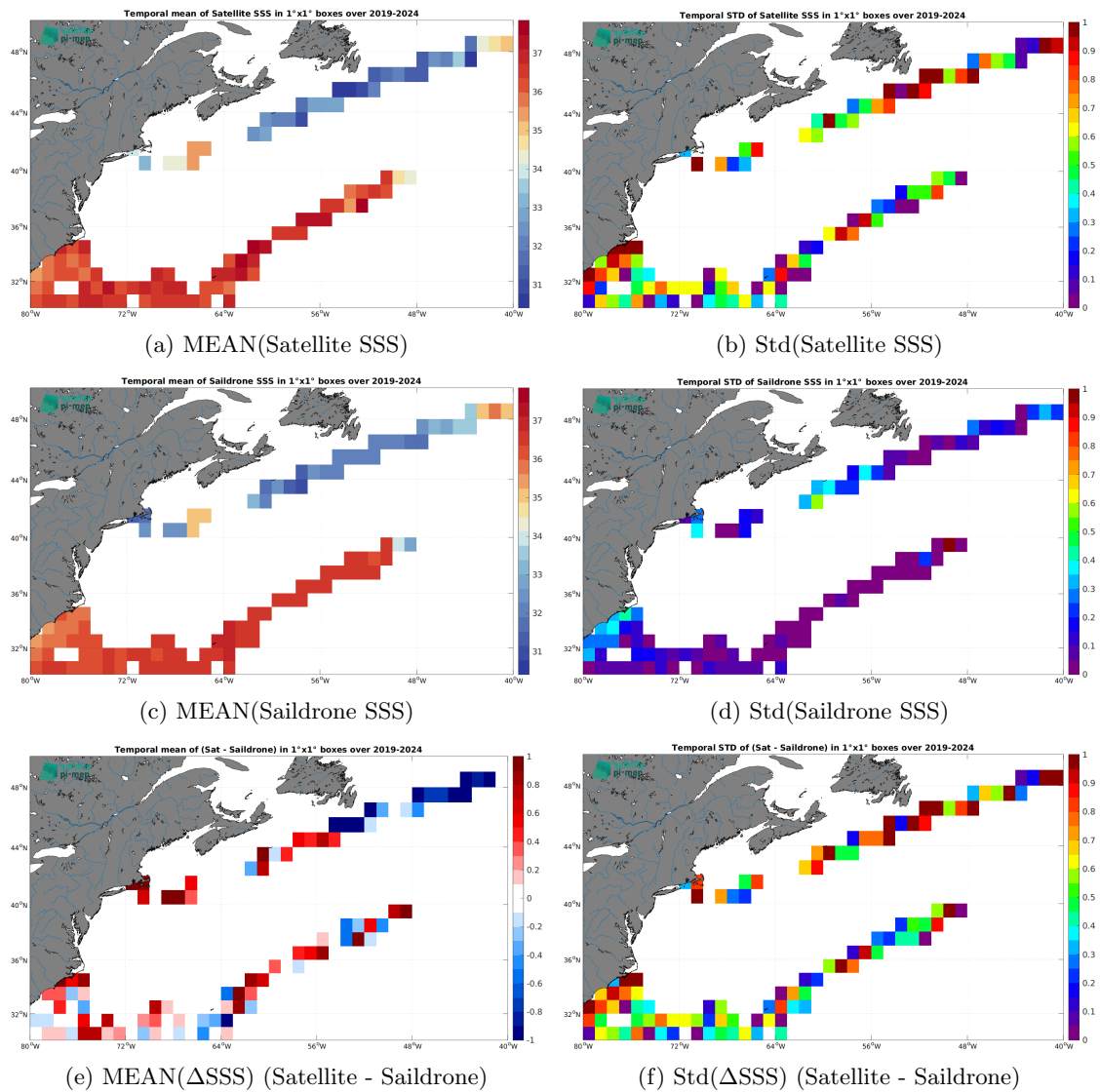
Figure 7: Temporal mean (left) and Std (right) of SSS from SMAP SSS L2 v6 - 40 km (RSS) (top), Saildrone (middle), and of \Delta SSS (Satellite - Saildrone). Only match-up pairs are used to generate these maps.
