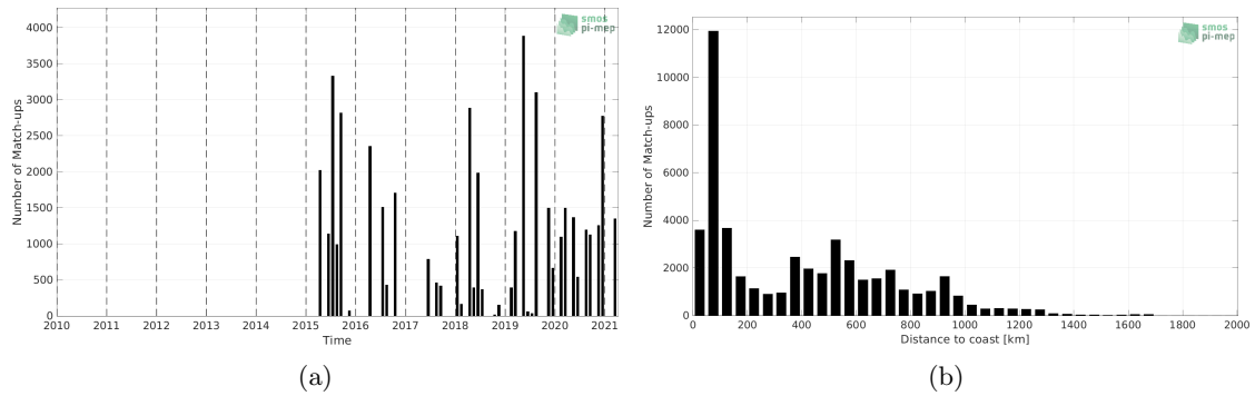
Figure 1: Number of match-ups between TSG (LEGOS-DM) and SMAP SSS L2 v5 (RSS) SSS as a function of time (a) and as function of the distance to coast (b) over the Gulf Stream Pi-MEP region and for the full satellite product period.
