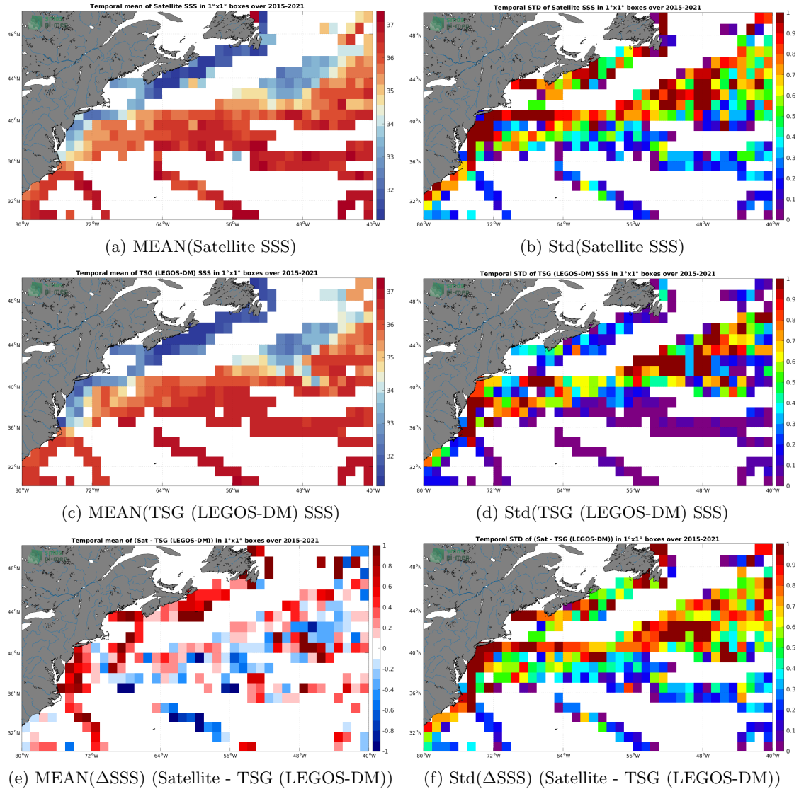
Figure 6: Temporal mean (left) and Std (right) of SSS from SMAP SSS L2 v5 (RSS) (top), TSG (LEGOS-DM) (middle), and of \Delta SSS (Satellite - TSG (LEGOS-DM)). Only match-up pairs are used to generate these maps.
