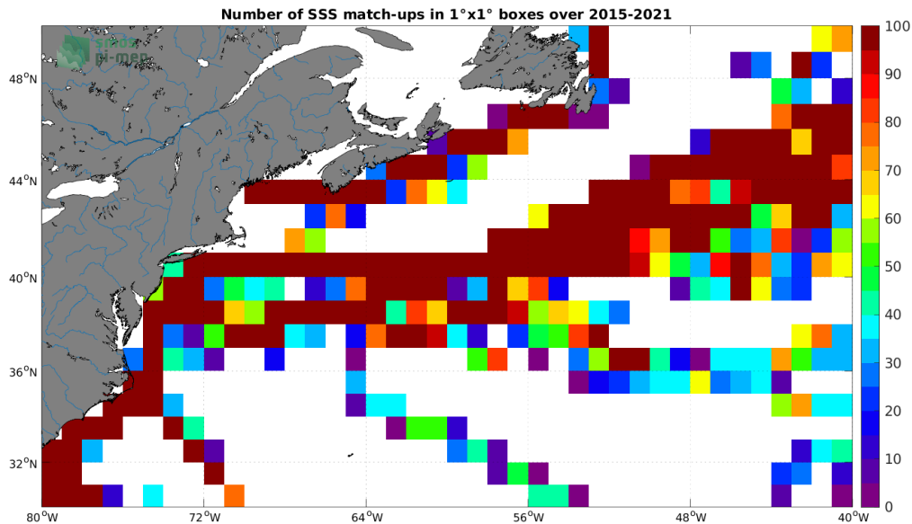
Figure 4: Number of SSS match-ups between TSG (LEGOS-DM) SSS and the SMAP SSS L2 v5 (RSS) SSS product for the Gulf Stream Pi-MEP region over 1^\circ \times 1^\circ boxes and for the full satellite product period.
