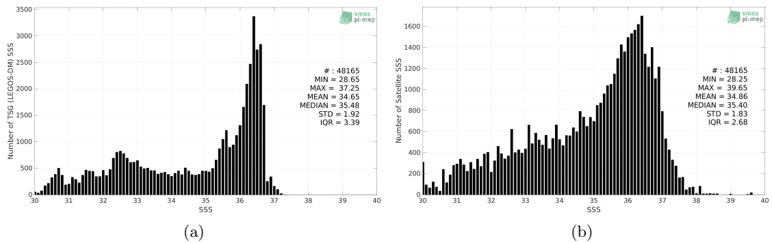
Figure 2: Histograms of SSS from TSG (LEGOS-DM) (a) and SMAP SSS L2 v5 (RSS) (b) considering all match-up pairs per bins of 0.1 over the Gulf Stream Pi-MEP region and for the full satellite product period.
