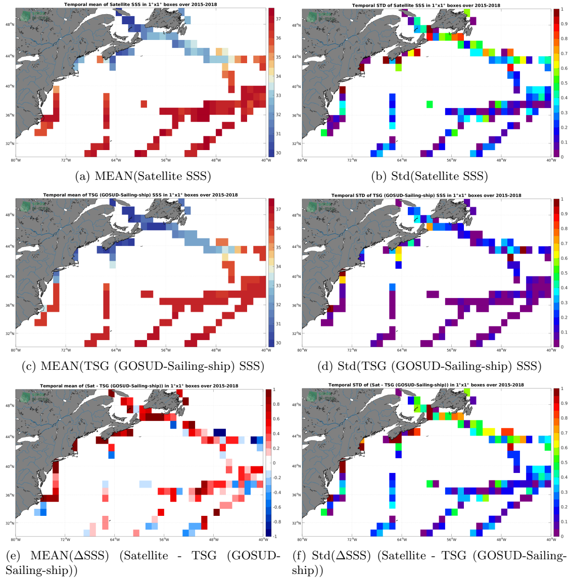
Figure 6: Temporal mean (left) and Std (right) of SSS from SMAP SSS L2 v5 (RSS) (top), TSG (GOSUD-Sailing-ship) (middle), and of \Delta SSS (Satellite - TSG (GOSUD-Sailing-ship)). Only match-up pairs are used to generate these maps.
