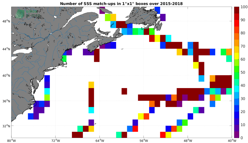
Figure 4: Number of SSS match-ups between TSG (GOSUD-Sailing-ship) SSS and the SMAP SSS L2 v5 (RSS) SSS product for the Gulf Stream Pi-MEP region over 1^\circ \times 1^\circ boxes and for the full satellite product period.
