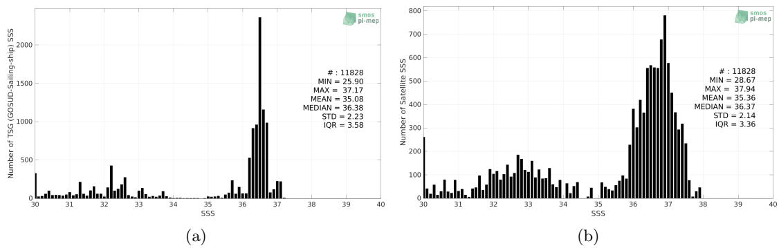
Figure 2: Histograms of SSS from TSG (GOSUD-Sailing-ship) (a) and SMAP SSS L2 v5 (RSS) (b) considering all match-up pairs per bins of 0.1 over the Gulf Stream Pi-MEP region and for the full satellite product period.
