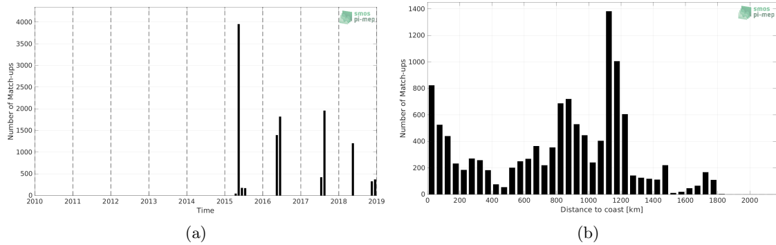
Figure 1: Number of match-ups between TSG (GOSUD-Sailing-ship) and SMAP SSS L2 v5 (RSS) SSS as a function of time (a) and as function of the distance to coast (b) over the Gulf Stream Pi-MEP region and for the full satellite product period.
