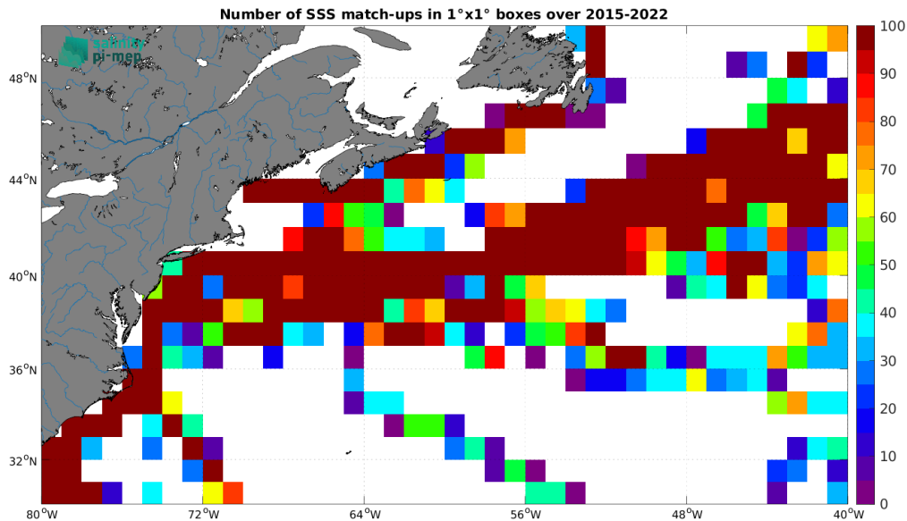
Figure 5: Number of SSS match-ups between TSG (LEGOS-DM) SSS and the SMAP SSS L2 v5.3 (RSS) SSS product for the Gulf Stream Pi-MEP region over 1^\circ \times 1^\circ boxes and for the full satellite product period.
