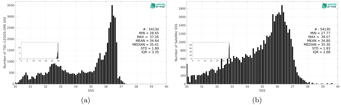
Figure 3: Histograms of SSS from TSG (LEGOS-DM) (a) and SMAP SSS L2 v5.3 (RSS) (b) considering all match-up pairs per bins of 0.1 over the Gulf Stream Pi-MEP region and for the full satellite product period.
