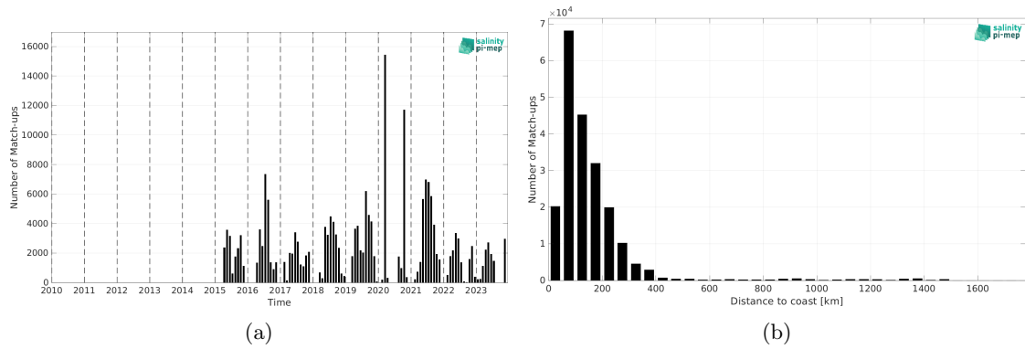
Figure 2: Number of match-ups between TSG (SAMOS) and SMAP SSS L2 v5.3 - 40 km (RSS) SSS as a function of time (a) and as function of the distance to coast (b) over the Gulf Stream Pi-MEP region and for the full satellite product period.
