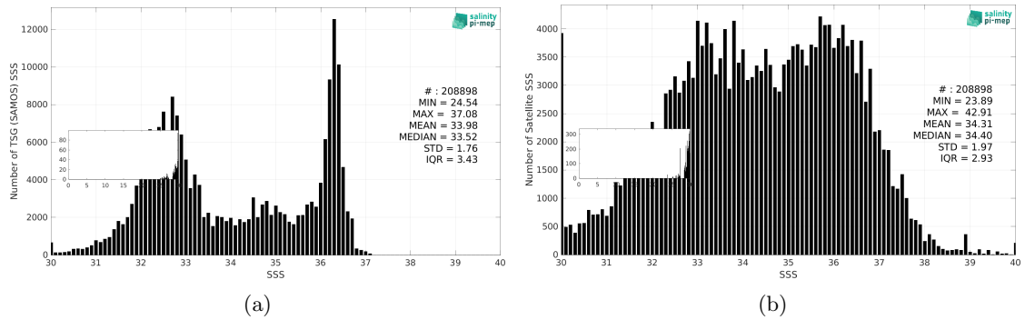
Figure 3: Histograms of SSS from TSG (SAMOS) (a) and SMAP SSS L2 v5.3 - 40 km (RSS) (b) considering all match-up pairs per bins of 0.1 over the Gulf Stream Pi-MEP region and for the full satellite product period.
