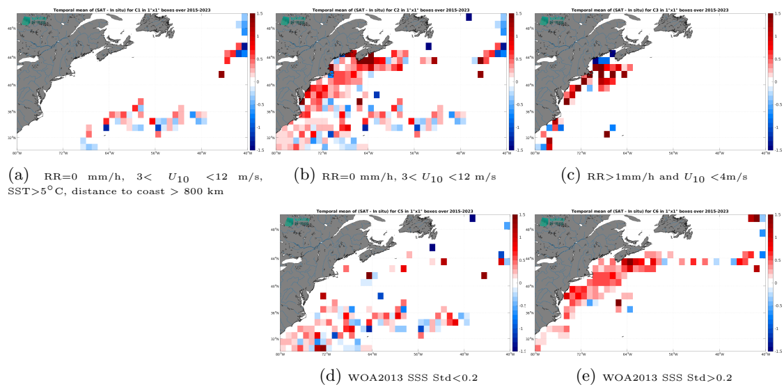
Figure 14: Temporal mean gridded over spatial boxes of size 1^\circ \times 1^\circ of \Delta SSS (SMAP SSS L2 v5.3 - 40 km (RSS) - TSG (SAMOS)) for 5 different subdatasets corresponding to:RR=0 mm/h, 3 < U_{10} < 12 m/s, SST>5°C, distance to coast > 800 km (a), RR=0 mm/h, 3 < U_{10} < 12 m/s (b), RR>1mm/h and U_{10} < 4 m/s (c), WOA2013 SSS Std<0.2 (d), WOA2013 SSS Std>0.2 (e).
