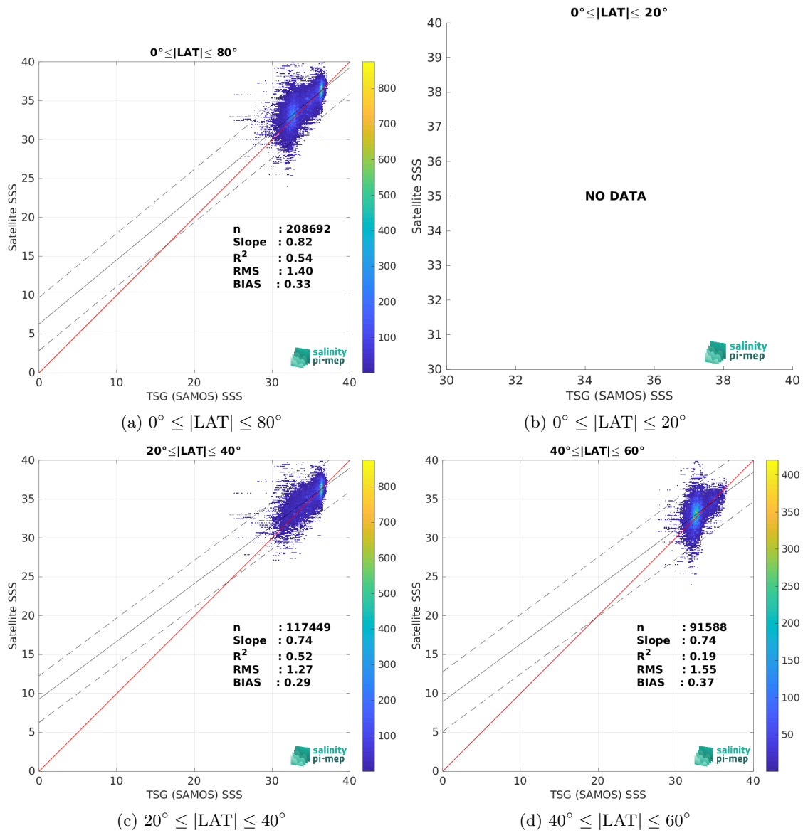
Figure 10: Contour maps of the concentration of SMAP SSS L2 v5.3 - 40 km (RSS) SSS (y-axis) versus TSG (SAMOS) SSS (x-axis) at match-up pairs for different latitude bands. For each plot, the red line shows x=y . The black thin and dashed lines indicate a linear fit through the data cloud and the \pm 95\% confidence levels, respectively. The number match-up pairs n , the slope and R^2 coefficient of the linear fit, the root mean square (RMS) and the mean bias between satellite and in situ data are indicated for each latitude band in each plots.
