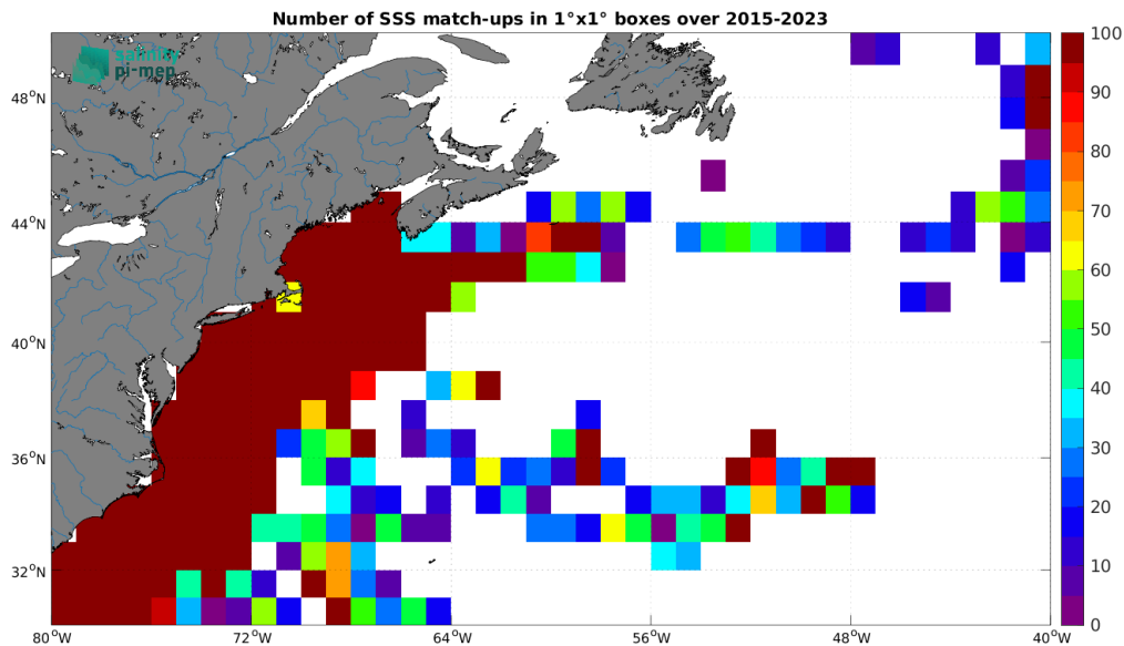
Figure 5: Number of SSS match-ups between TSG (SAMOS) SSS and the SMAP SSS L2 v5.3 - 40 km (RSS) SSS product for the Gulf Stream Pi-MEP region over 1^\circ \times 1^\circ boxes and for the full satellite product period.
