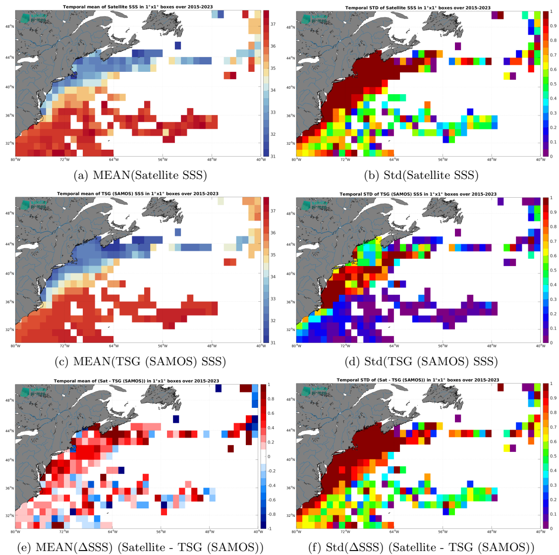
Figure 7: Temporal mean (left) and Std (right) of SSS from SMAP SSS L2 v5.3 - 40 km (RSS) (top), TSG (SAMOS) (middle), and of \Delta SSS (Satellite - TSG (SAMOS)). Only match-up pairs are used to generate these maps.
