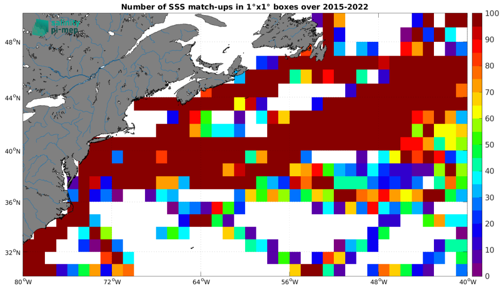
Figure 5: Number of SSS match-ups between TSG (LEGOS-DM) SSS and the SMAP SSS L2 v5.0 (JPL) SSS product for the Gulf Stream Pi-MEP region over 1^\circ \times 1^\circ boxes and for the full satellite product period.
