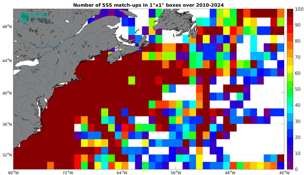
Figure 5: Number of SSS match-ups between TSG (SAMOS) SSS and the ISAS SSS product for the Gulf Stream Pi-MEP region over 1^\circ \times 1^\circ boxes and for the full satellite product period.
