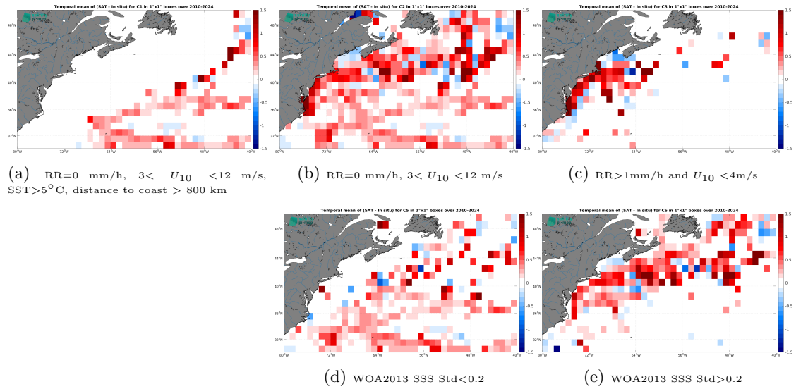
Figure 14: Temporal mean gridded over spatial boxes of size 1^\circ \times 1^\circ of \Delta SSS (ISAS - TSG (SAMOS)) for 5 different subdatasets corresponding to:RR=0 mm/h, 3 < U_{10} < 12 m/s, SST >5^\circ C, distance to coast > 800 km (a), RR=0 mm/h, 3 < U_{10} < 12 m/s (b), RR >1 mm/h and U_{10} < 4 m/s (c), WOA2013 SSS Std <0.2 (d), WOA2013 SSS Std >0.2 (e).
