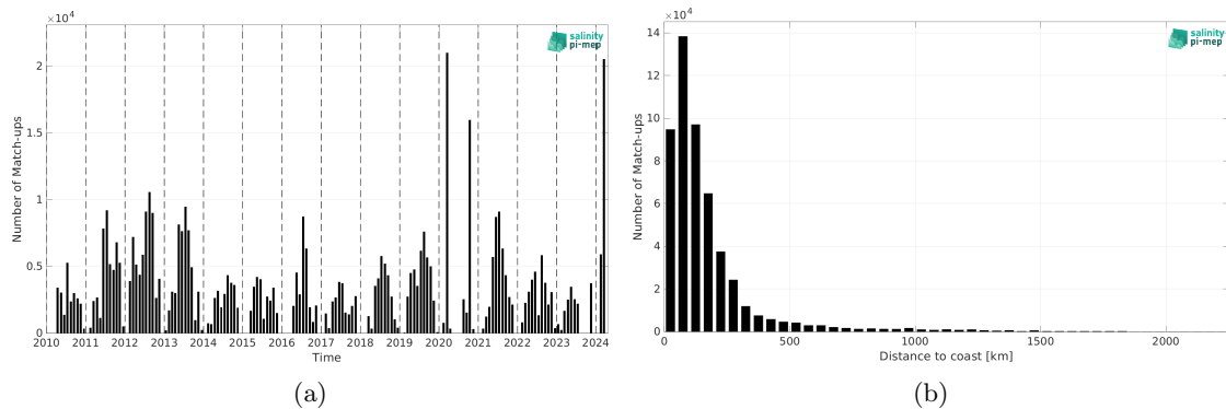
Figure 2: Number of match-ups between TSG (SAMOS) and ISAS SSS as a function of time (a) and as function of the distance to coast (b) over the Gulf Stream Pi-MEP region and for the full satellite product period.
