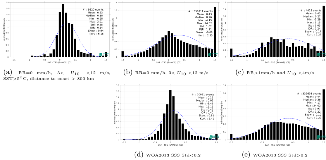
Figure 15: Normalized histogram of \Delta\text{SSS} (ISAS - TSG (SAMOS)) for 5 different subdatasets corresponding to: RR=0 mm/h, 3 < U_{10} < 12 m/s, SST>5°C, distance to coast > 800 km (a), RR=0 mm/h, 3 < U_{10} < 12 m/s (b), RR>1mm/h and U_{10} < 4 m/s (c), WOA2013 SSS Std<0.2 (d), WOA2013 SSS Std>0.2 (e).
