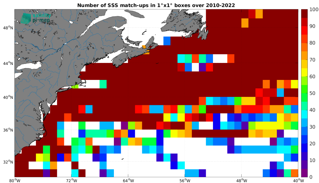
Figure 5: Number of SSS match-ups between TSG (LEGOS-DM) SSS and the ISAS SSS product for the Gulf Stream Pi-MEP region over 1^\circ \times 1^\circ boxes and for the full satellite product period.
