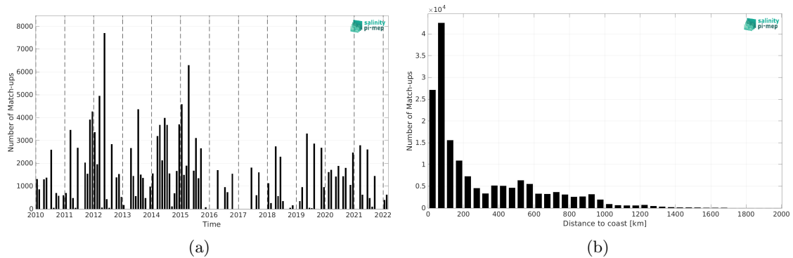
Figure 2: Number of match-ups between TSG (LEGOS-DM) and ISAS SSS as a function of time (a) and as function of the distance to coast (b) over the Gulf Stream Pi-MEP region and for the full satellite product period.
