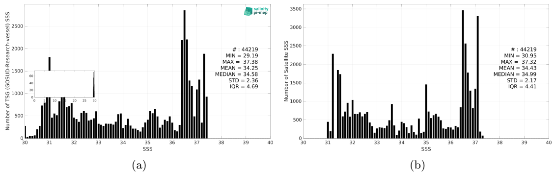
Figure 3: Histograms of SSS from TSG (GOSUD-Research-vessel) (a) and ISAS v7 - Monthly (Ifremer-LOPS-CMEMS) (b) considering all match-up pairs per bins of 0.1 over the Gulf Stream Pi-MEP region and for the full satellite product period.
