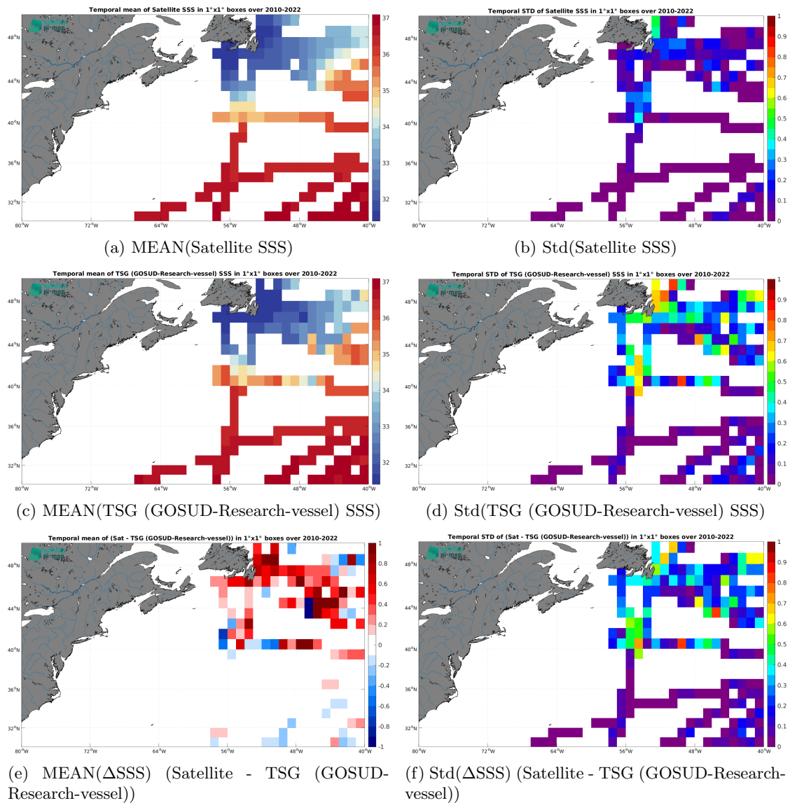
Figure 7: Temporal mean (left) and Std (right) of SSS from ISAS v7 - Monthly (Ifremer-LOPS-CMEMS) (top), TSG (GOSUD-Research-vessel) (middle), and of \Delta SSS (Satellite - TSG (GOSUD-Research-vessel)). Only match-up pairs are used to generate these maps.
