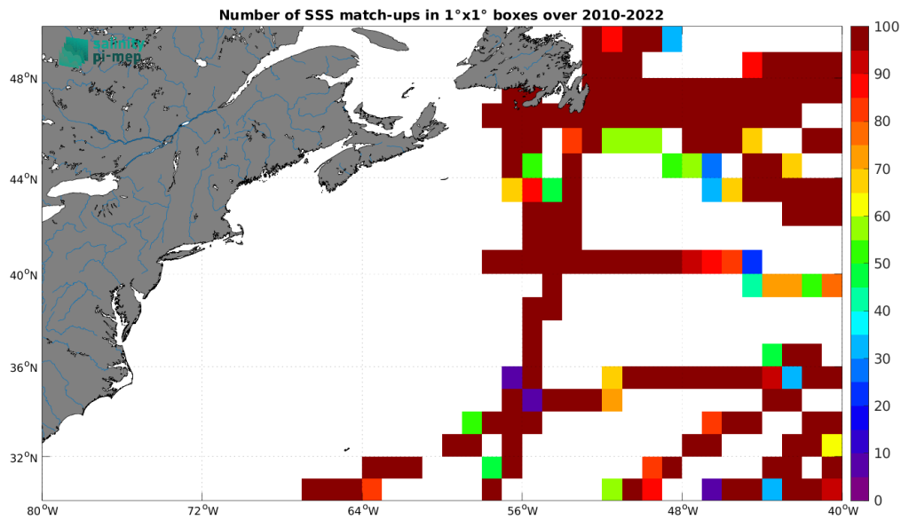
Figure 5: Number of SSS match-ups between TSG (GOSUD-Research-vessel) SSS and the ISAS v7 - Monthly (Ifremer-LOPS-CMEMS) SSS product for the Gulf Stream Pi-MEP region over 1^\circ \times 1^\circ boxes and for the full satellite product period.
