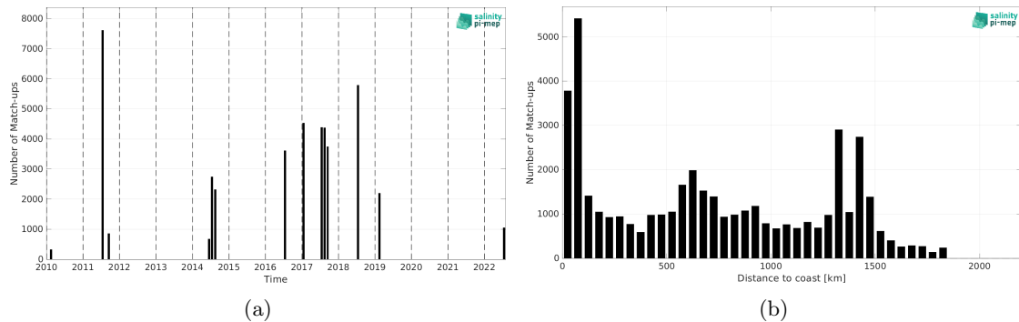
Figure 2: Number of match-ups between TSG (GOSUD-Research-vessel) and ISAS v7 - Monthly (Ifremer-LOPS-CMEMS) SSS as a function of time (a) and as function of the distance to coast (b) over the Gulf Stream Pi-MEP region and for the full satellite product period.
