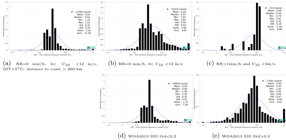
Figure 15: Normalized histogram of \Delta\text{SSS} (ISAS v7 - Monthly (Ifremer-LOPS-CMEMS) - TSG (GOSUD-Research-vessel)) for 5 different subdatasets corresponding to: RR=0 mm/h, 3 < U_{10} < 12 m/s, SST > 5^\circ\text{C} , distance to coast > 800 km (a), RR=0 mm/h, 3 < U_{10} < 12 m/s (b), RR > 1 mm/h and U_{10} < 4 m/s (c), WOA2013 SSS Std < 0.2 (d), WOA2013 SSS Std > 0.2 (e).
