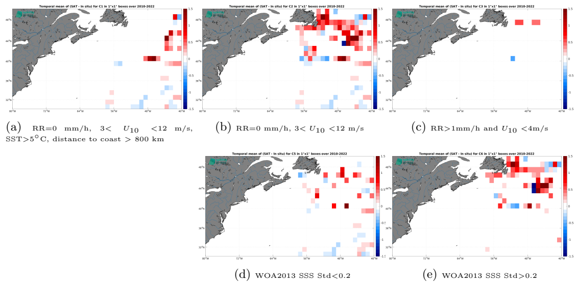
Figure 14: Temporal mean gridded over spatial boxes of size 1^\circ \times 1^\circ of \Delta SSS (ISAS v7 - Monthly (Ifremer-LOPS-CMEMS) - TSG (GOSUD-Research-vessel)) for 5 different subdatasets corresponding to:RR=0 mm/h, 3 < U_{10} < 12 m/s, SST>5°C, distance to coast > 800 km (a), RR=0 mm/h, 3 < U_{10} < 12 m/s (b), RR>1mm/h and U_{10} < 4 m/s (c), WOA2013 SSS Std<0.2 (d), WOA2013 SSS Std>0.2 (e).
