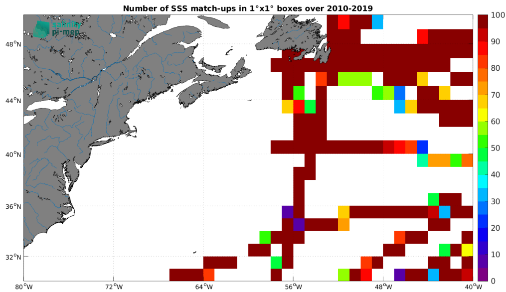
Figure 5: Number of SSS match-ups between TSG (GOSUD-Research-vessel) SSS and the ISAS SSS product for the Gulf Stream Pi-MEP region over 1^\circ \times 1^\circ boxes and for the full satellite product period.
