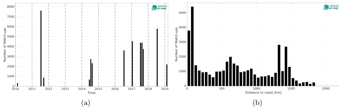
Figure 2: Number of match-ups between TSG (GOSUD-Research-vessel) and ISAS SSS as a function of time (a) and as function of the distance to coast (b) over the Gulf Stream Pi-MEP region and for the full satellite product period.
