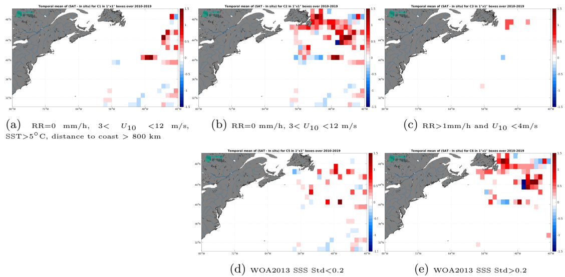
Figure 14: Temporal mean gridded over spatial boxes of size 1^\circ \times 1^\circ of \Delta SSS (ISAS - TSG (GOSUD-Research-vessel)) for 5 different subdatasets corresponding to:RR=0 mm/h, 3 < U_{10} < 12 m/s, SST > 5°C, distance to coast > 800 km (a), RR=0 mm/h, 3 < U_{10} < 12 m/s (b), RR > 1mm/h and U_{10} < 4 m/s (c), WOA2013 SSS Std < 0.2 (d), WOA2013 SSS Std > 0.2 (e).
