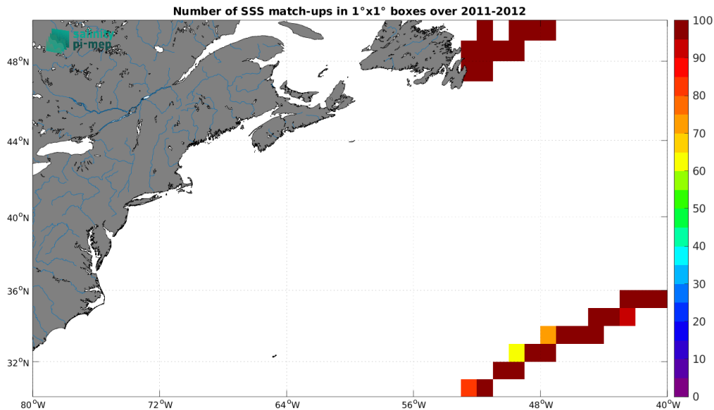
Figure 5: Number of SSS match-ups between TSG (CSIC-UTM) SSS and the ISAS SSS product for the Gulf Stream Pi-MEP region over 1^\circ \times 1^\circ boxes and for the full satellite product period.
