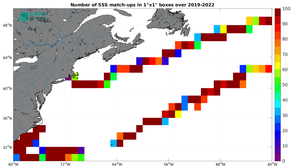
Figure 5: Number of SSS match-ups between Saildrone SSS and the ISAS SSS product for the Gulf Stream Pi-MEP region over 1^\circ \times 1^\circ boxes and for the full satellite product period.
