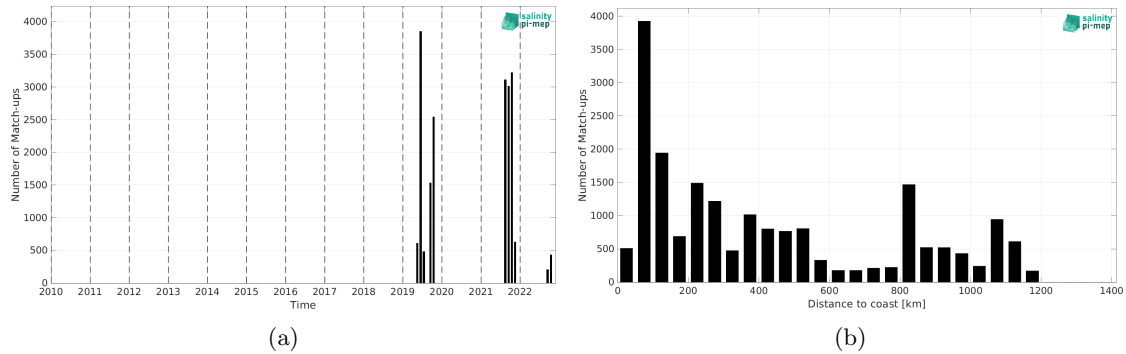
Figure 2: Number of match-ups between Sairdrone and ISAS SSS as a function of time (a) and as function of the distance to coast (b) over the Gulf Stream Pi-MEP region and for the full satellite product period.
