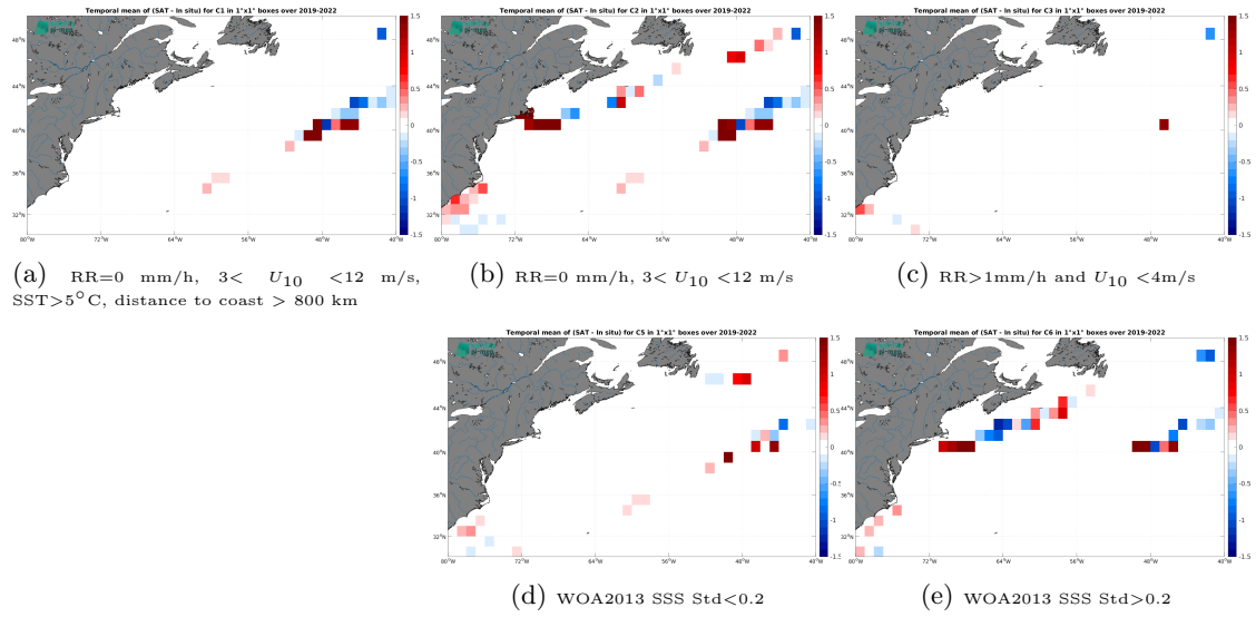
Figure 14: Temporal mean gridded over spatial boxes of size 1^\circ \times 1^\circ of \Delta SSS (ISAS - Saildrone) for 5 different subdatasets corresponding to:RR=0 mm/h, 3 < U_{10} < 12 m/s, SST > 5^\circ\text{C} , distance to coast > 800 km (a), RR=0 mm/h, 3 < U_{10} < 12 m/s (b), RR > 1 mm/h and U_{10} < 4 m/s (c), WOA2013 SSS Std < 0.2 (d), WOA2013 SSS Std > 0.2 (e).
