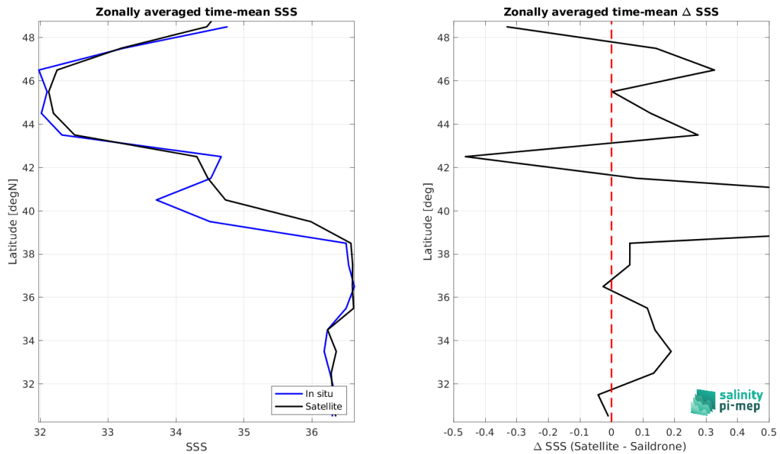
Figure 9: Left panel: Zonal mean SSS from ISAS satellite product (black) and from Sairdron (blue). Right panel: Zonal mean of \Delta SSS (Satellite - Sairdron) for all the collected Pi-MEP match-up pairs estimated over the full satellite product period.
