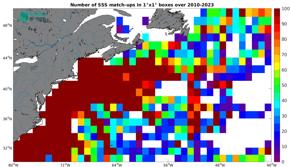
Figure 5: Number of SSS match-ups between TSG (SAMOS) SSS and the CCI SSS L4 Merged-OI v5.5 - 7-day running (ESA) SSS product for the Gulf Stream Pi-MEP region over 1^\circ \times 1^\circ boxes and for the full satellite product period.
