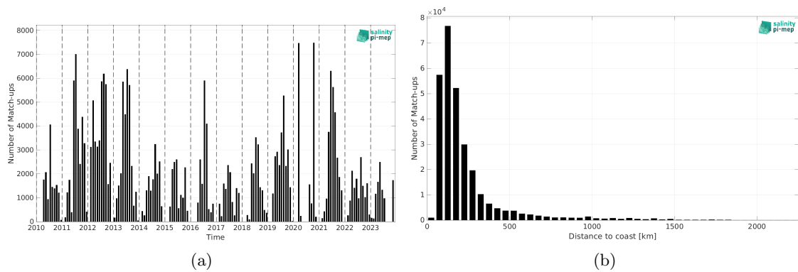
Figure 2: Number of match-ups between TSG (SAMOS) and CCI SSS L4 Merged-OI v5.5 - 7-day running (ESA) SSS as a function of time (a) and as function of the distance to coast (b) over the Gulf Stream Pi-MEP region and for the full satellite product period.
