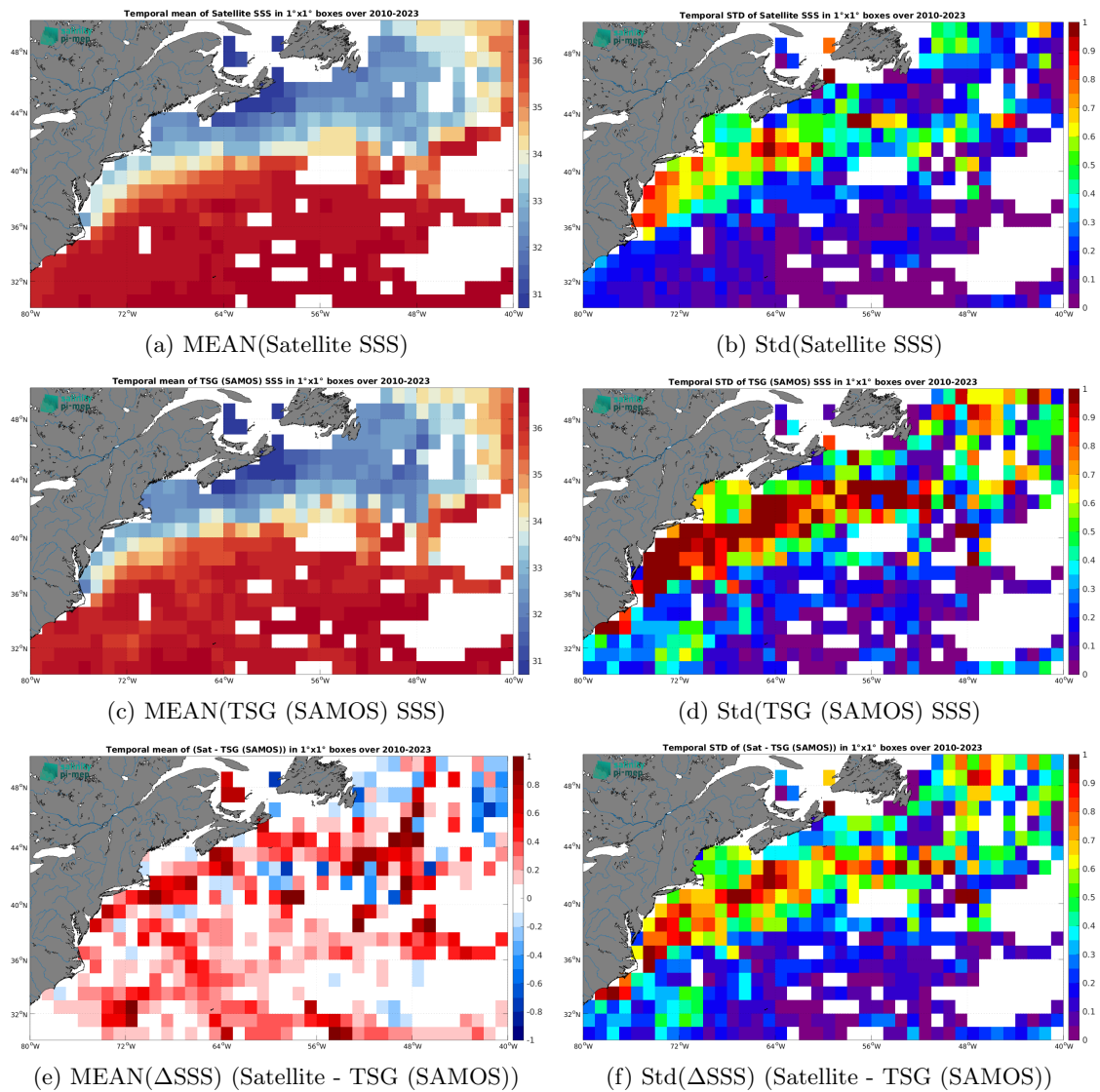
Figure 7: Temporal mean (left) and Std (right) of SSS from CCI SSS L4 Merged-OI v5.5 - 7-day running (ESA) (top), TSG (SAMOS) (middle), and of \Delta SSS (Satellite - TSG (SAMOS)). Only match-up pairs are used to generate these maps.
