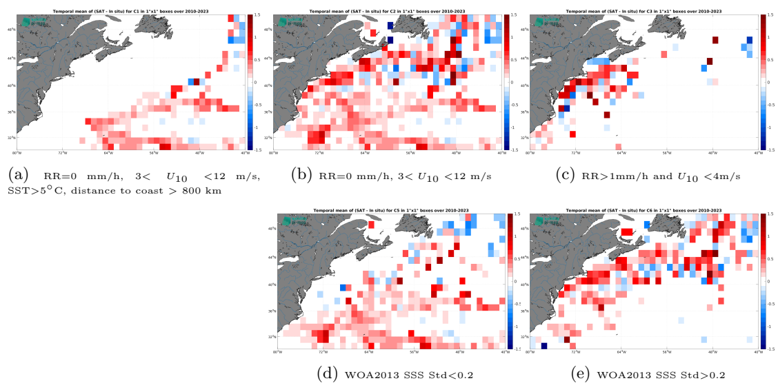
Figure 14: Temporal mean gridded over spatial boxes of size 1^\circ \times 1^\circ of \Delta\text{SSS} (CCI SSS L4 Merged-OI v5.5 - 7-day running (ESA) - TSG (SAMOS)) for 5 different subdatasets corresponding to:RR=0 mm/h, 3 < U_{10} < 12 m/s, SST >5^\circ\text{C} , distance to coast > 800 km (a), RR=0 mm/h, 3 < U_{10} < 12 m/s (b), RR >1 mm/h and U_{10} < 4 m/s (c), WOA2013 SSS Std <0.2 (d), WOA2013 SSS Std >0.2 (e).
