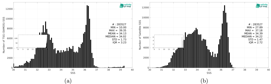
Figure 3: Histograms of SSS from TSG (SAMOS) (a) and CCI SSS L4 Merged-OI v5.5 - 7-day running (ESA) (b) considering all match-up pairs per bins of 0.1 over the Gulf Stream Pi-MEP region and for the full satellite product period.
