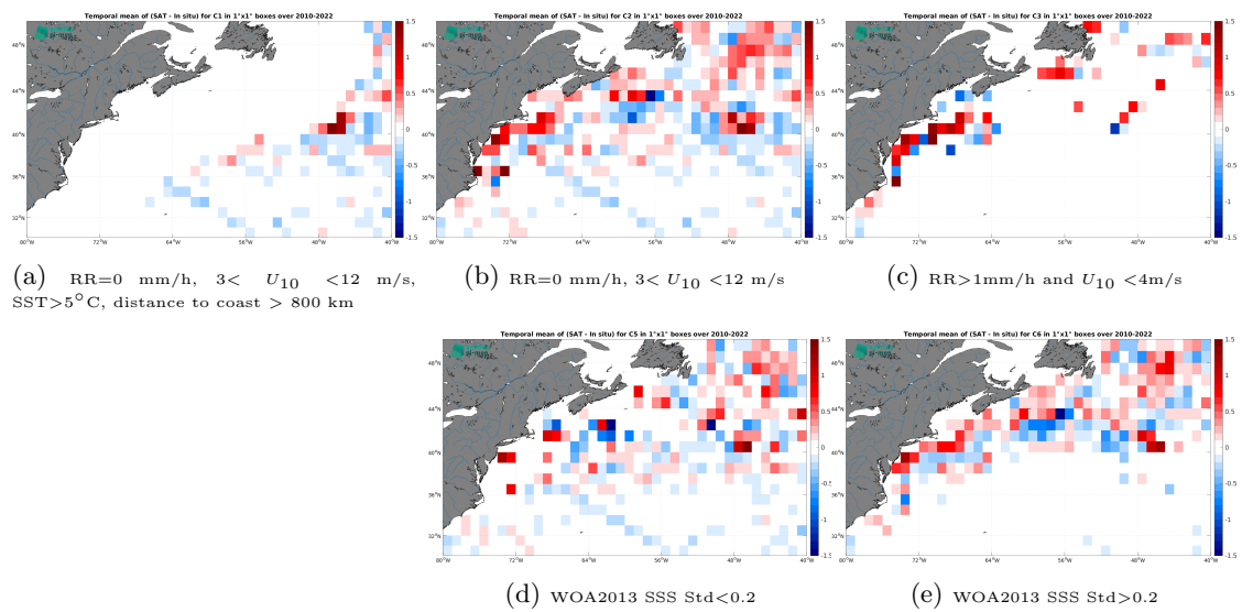
Figure 14: Temporal mean gridded over spatial boxes of size 1^\circ \times 1^\circ of \Delta SSS (CCI SSS L4 Merged-OI v5.5 - 7-day running (ESA) - TSG (LEGOS-DM)) for 5 different subdatasets corresponding to:RR=0 mm/h, 3 < U_{10} < 12 m/s, SST >5^\circ C, distance to coast > 800 km (a), RR=0 mm/h, 3 < U_{10} < 12 m/s (b), RR >1 mm/h and U_{10} < 4 m/s (c), WOA2013 SSS Std <0.2 (d), WOA2013 SSS Std >0.2 (e).
