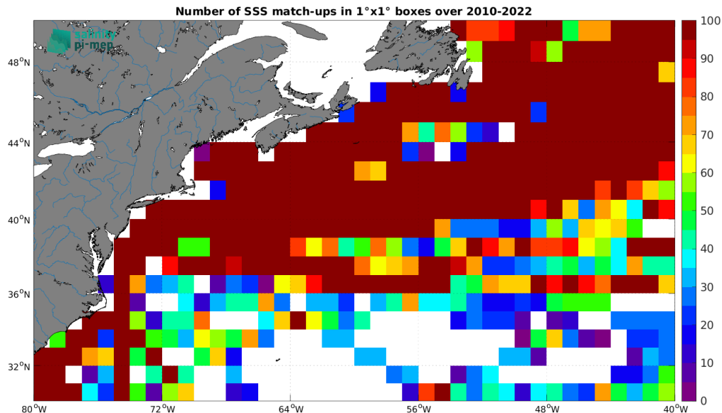
Figure 5: Number of SSS match-ups between TSG (LEGOS-DM) SSS and the CCI SSS L4 Merged-OI v5.5 - 7-day running (ESA) SSS product for the Gulf Stream Pi-MEP region over 1^\circ \times 1^\circ boxes and for the full satellite product period.
