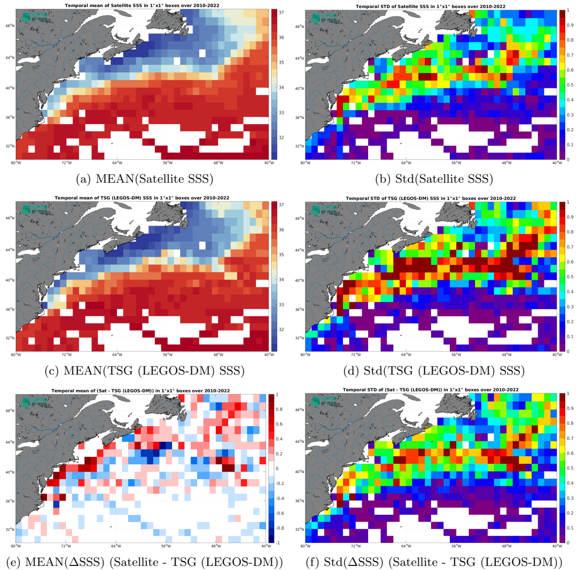
Figure 7: Temporal mean (left) and Std (right) of SSS from CCI SSS L4 Merged-OI v5.5 - 7-day running (ESA) (top), TSG (LEGOS-DM) (middle), and of \Delta SSS (Satellite - TSG (LEGOS-DM)). Only match-up pairs are used to generate these maps.
