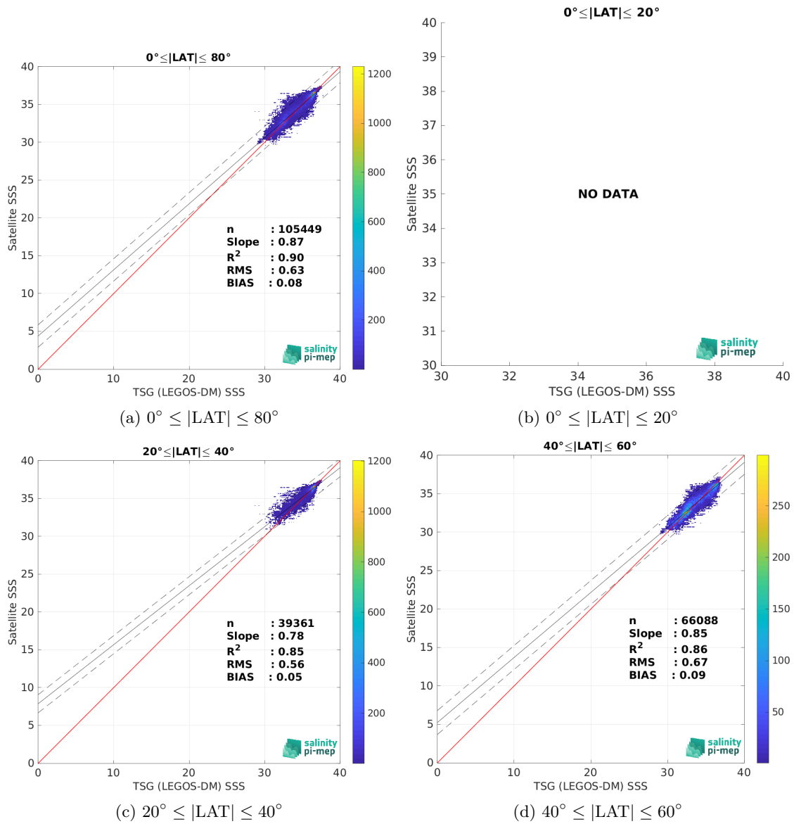
Figure 10: Contour maps of the concentration of CCI SSS L4 Merged-OI v5.5 - 7-day running (ESA) SSS (y-axis) versus TSG (LEGOS-DM) SSS (x-axis) at match-up pairs for different latitude bands. For each plot, the red line shows x=y . The black thin and dashed lines indicate a linear fit through the data cloud and the \pm 95\% confidence levels, respectively. The number match-up pairs n , the slope and R^2 coefficient of the linear fit, the root mean square (RMS) and the mean bias between satellite and in situ data are indicated for each latitude band in each plots.
