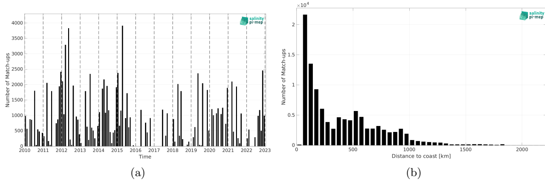
Figure 2: Number of match-ups between TSG (LEGOS-DM) and CCI SSS L4 Merged-OI v5.5 - 7-day running (ESA) SSS as a function of time (a) and as function of the distance to coast (b) over the Gulf Stream Pi-MEP region and for the full satellite product period.
