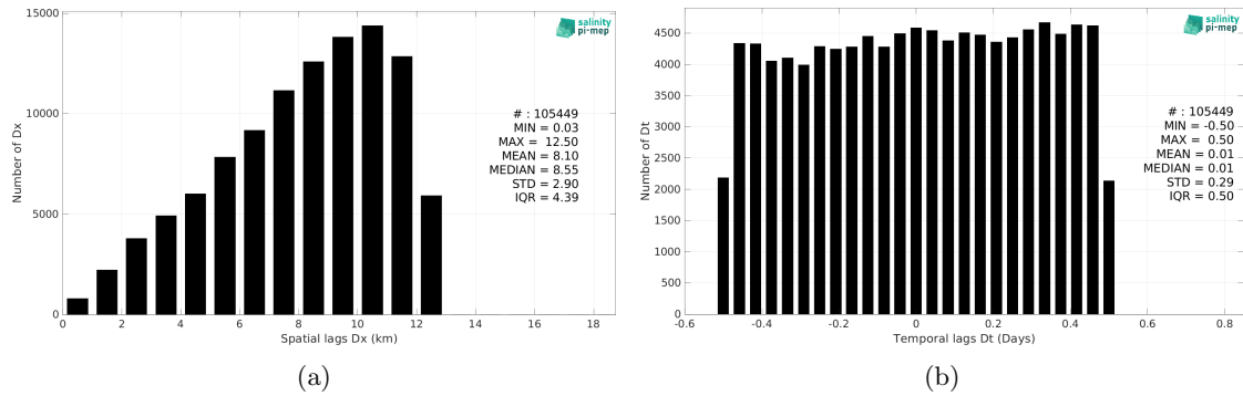
Figure 6: Histograms of the spatial (a) and temporal (b) lags between the location/time of the TSG (LEGOS-DM) measurement and the date of the corresponding CCI SSS L4 Merged-OI v5.5 - 7-day running (ESA) SSS pixel.
