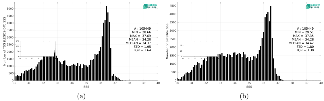
Figure 3: Histograms of SSS from TSG (LEGOS-DM) (a) and CCI SSS L4 Merged-OI v5.5 - 7-day running (ESA) (b) considering all match-up pairs per bins of 0.1 over the Gulf Stream Pi-MEP region and for the full satellite product period.
