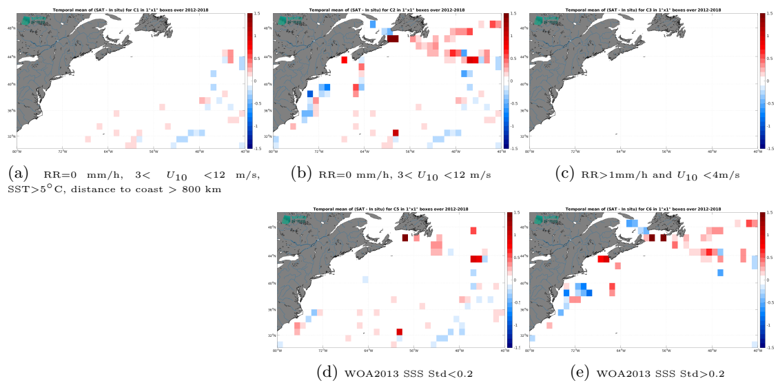
Figure 14: Temporal mean gridded over spatial boxes of size 1^\circ \times 1^\circ of \Delta SSS (CCI SSS L4 Merged-OI v5.5 - 7-day running (ESA) - TSG (GOSUD-Sailing-ship)) for 5 different subdatasets corresponding to: RR=0 mm/h, 3 < U_{10} < 12 m/s, SST>5°C, distance to coast > 800 km (a), RR=0 mm/h, 3 < U_{10} < 12 m/s (b), RR>1mm/h and U_{10} < 4 m/s (c), WOA2013 SSS Std<0.2 (d), WOA2013 SSS Std>0.2 (e).
