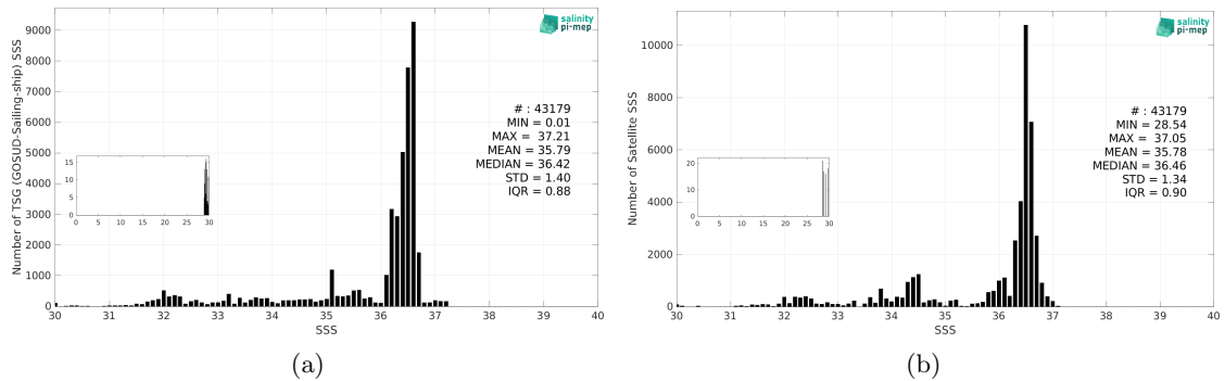
Figure 3: Histograms of SSS from TSG (GOSUD-Sailing-ship) (a) and CCI SSS L4 Merged-OI v5.5 - 7-day running (ESA) (b) considering all match-up pairs per bins of 0.1 over the Gulf Stream Pi-MEP region and for the full satellite product period.
