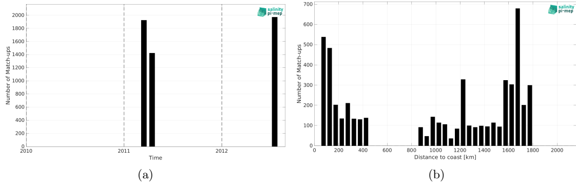
Figure 2: Number of match-ups between TSG (CSIC-UTM) and CCI SSS L4 Merged-OI v5.5 - 7-day running (ESA) SSS as a function of time (a) and as function of the distance to coast (b) over the Gulf Stream Pi-MEP region and for the full satellite product period.
