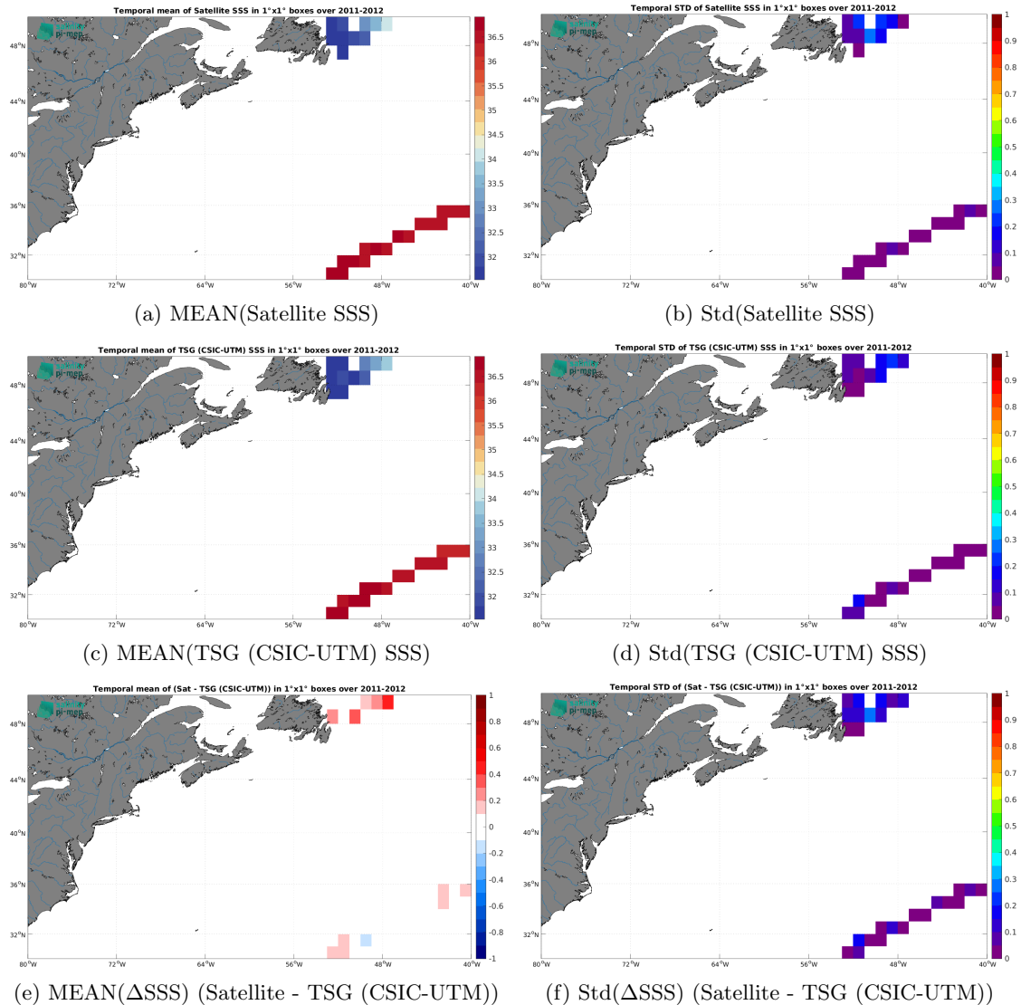
Figure 7: Temporal mean (left) and Std (right) of SSS from CCI SSS L4 Merged-OI v5.5 - 7-day running (ESA) (top), TSG (CSIC-UTM) (middle), and of \Delta SSS (Satellite - TSG (CSIC-UTM)). Only match-up pairs are used to generate these maps.
