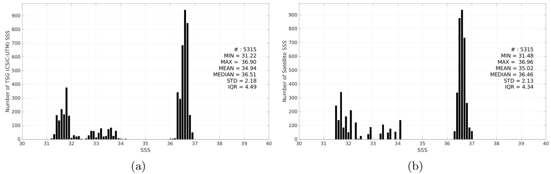
Figure 3: Histograms of SSS from TSG (CSIC-UTM) (a) and CCI SSS L4 Merged-OI v5.5 - 7-day running (ESA) (b) considering all match-up pairs per bins of 0.1 over the Gulf Stream Pi-MEP region and for the full satellite product period.
