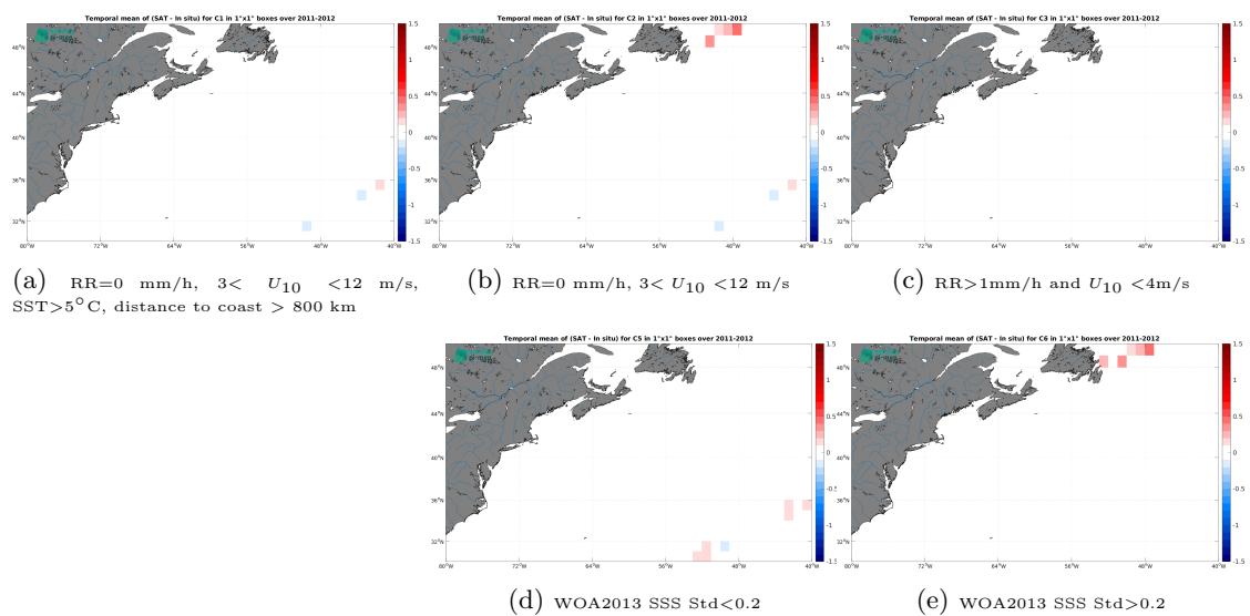
Figure 14: Temporal mean gridded over spatial boxes of size 1^\circ \times 1^\circ of \Delta SSS (CCI SSS L4 Merged-OI v5.5 - 7-day running (ESA) - TSG (CSIC-UTM)) for 5 different subdatasets corresponding to:RR=0 mm/h, 3 < U_{10} < 12 m/s, SST >5^\circ C, distance to coast > 800 km (a), RR=0 mm/h, 3 < U_{10} < 12 m/s (b), RR >1 mm/h and U_{10} < 4 m/s (c), WOA2013 SSS Std <0.2 (d), WOA2013 SSS Std >0.2 (e).
