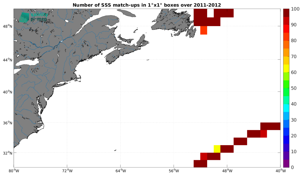
Figure 5: Number of SSS match-ups between TSG (CSIC-UTM) SSS and the CCI SSS L4 Merged-OI v5.5 - 7-day running (ESA) SSS product for the Gulf Stream Pi-MEP region over 1^\circ \times 1^\circ boxes and for the full satellite product period.
