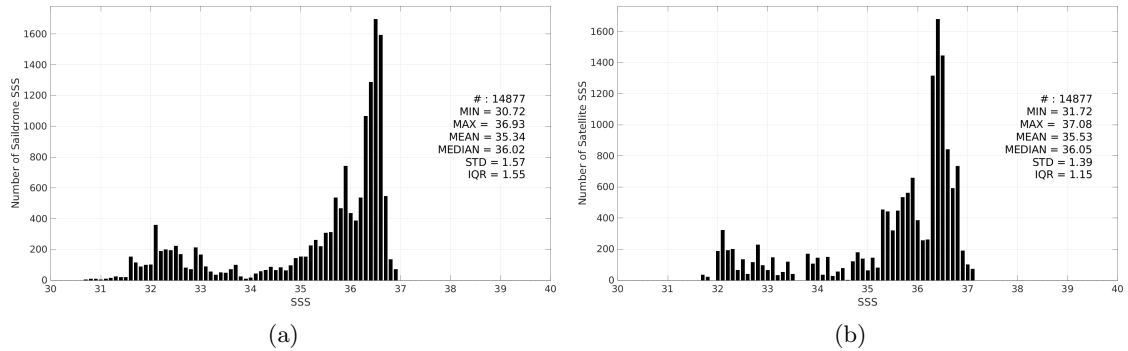
Figure 3: Histograms of SSS from Saildrone (a) and CCI SSS L4 Merged-OI v5.5 - 7-day running (ESA) (b) considering all match-up pairs per bins of 0.1 over the Gulf Stream Pi-MEP region and for the full satellite product period.
