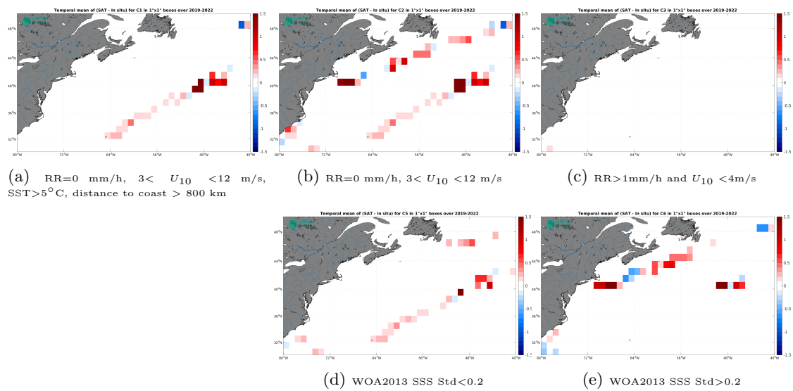
Figure 14: Temporal mean gridded over spatial boxes of size 1^\circ \times 1^\circ of \Delta SSS (CCI SSS L4 Merged-OI v5.5 - 7-day running (ESA) - Saildrone) for 5 different subdatasets corresponding to:RR=0 mm/h, 3 < U_{10} < 12 m/s, SST >5^\circ\text{C} , distance to coast > 800 km (a), RR=0 mm/h, 3 < U_{10} < 12 m/s (b), RR >1 mm/h and U_{10} < 4 m/s (c), WOA2013 SSS Std <0.2 (d), WOA2013 SSS Std >0.2 (e).
