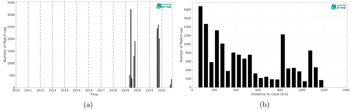
Figure 2: Number of match-ups between Saildrone and CCI SSS L4 Merged-OI v5.5 - 7-day running (ESA) SSS as a function of time (a) and as function of the distance to coast (b) over the Gulf Stream Pi-MEP region and for the full satellite product period.
