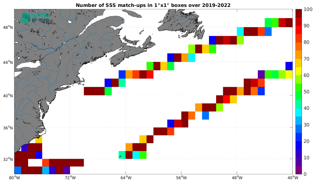
Figure 5: Number of SSS match-ups between Saildrone SSS and the CCI SSS L4 Merged-OI v5.5 - 7-day running (ESA) SSS product for the Gulf Stream Pi-MEP region over 1^\circ \times 1^\circ boxes and for the full satellite product period.
