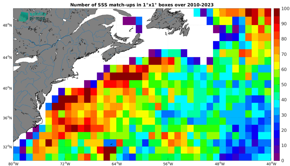
Figure 5: Number of SSS match-ups between Argo SSS and the CCI SSS L4 Merged-OI v5.5 - 7-day running (ESA) SSS product for the Gulf Stream Pi-MEP region over 1^\circ \times 1^\circ boxes and for the full satellite product period.
