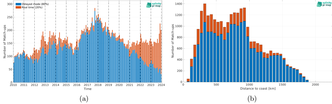
Figure 2: Number of match-ups between Argo and CCI SSS L4 Merged-OI v5.5 - 7-day running (ESA) SSS as a function of time (a) and as function of the distance to coast (b) over the Gulf Stream Pi-MEP region and for the full satellite product period.
