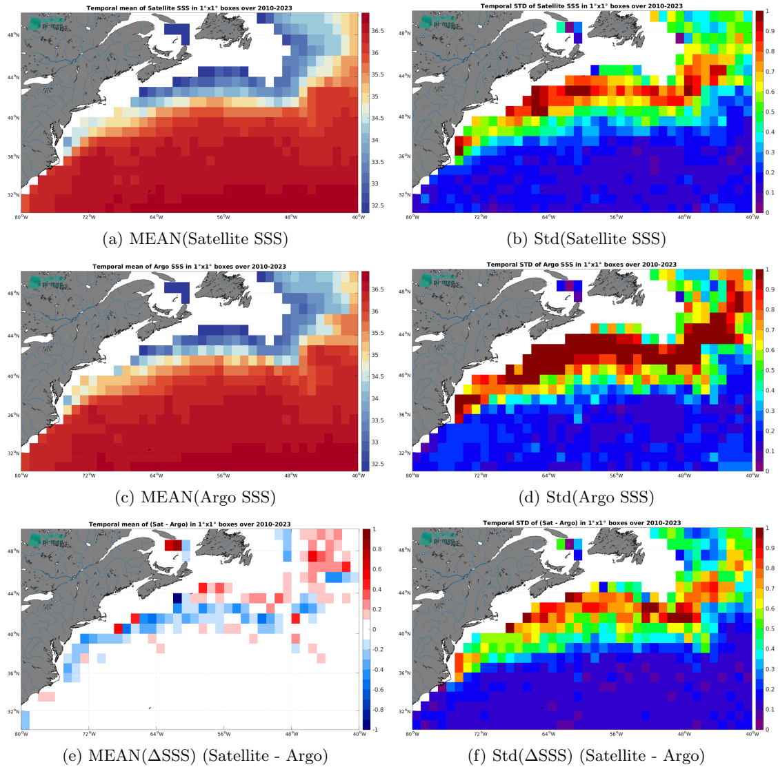
Figure 7: Temporal mean (left) and Std (right) of SSS from CCI SSS L4 Merged-OI v5.5 - 7-day running (ESA) (top), Argo (middle), and of \Delta SSS (Satellite - Argo). Only match-up pairs are used to generate these maps.
