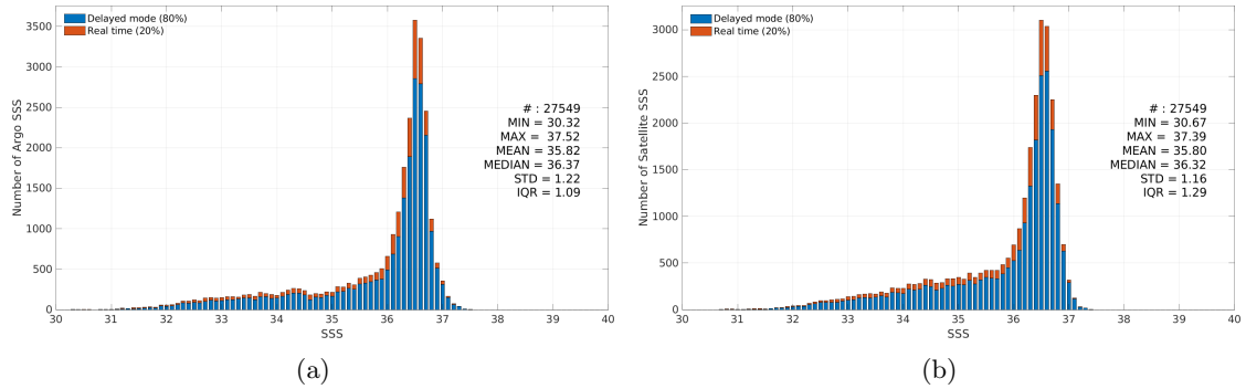
Figure 3: Histograms of SSS from Argo (a) and CCI SSS L4 Merged-OI v5.5 - 7-day running (ESA) (b) considering all match-up pairs per bins of 0.1 over the Gulf Stream Pi-MEP region and for the full satellite product period.
