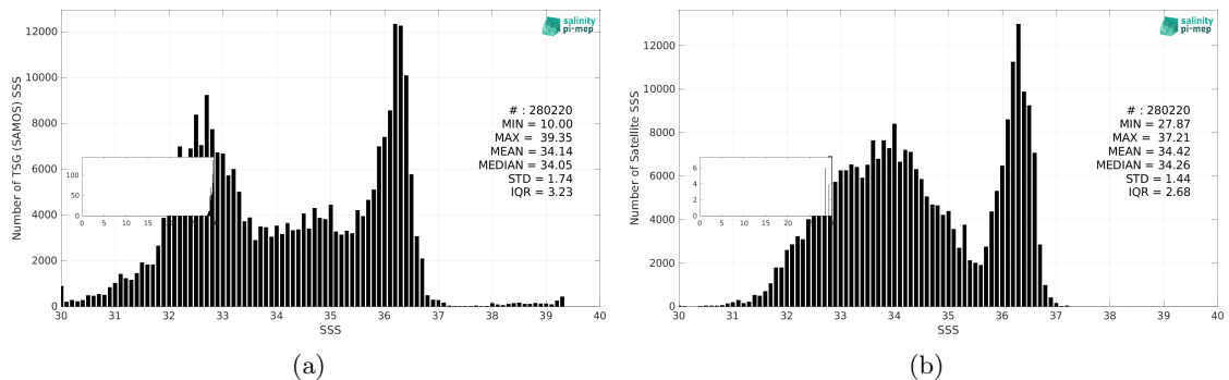
Figure 3: Histograms of SSS from TSG (SAMOS) (a) and CCI SSS L4 Merged-OI v5.5 - 30-day running (ESA) (b) considering all match-up pairs per bins of 0.1 over the Gulf Stream Pi-MEP region and for the full satellite product period.
