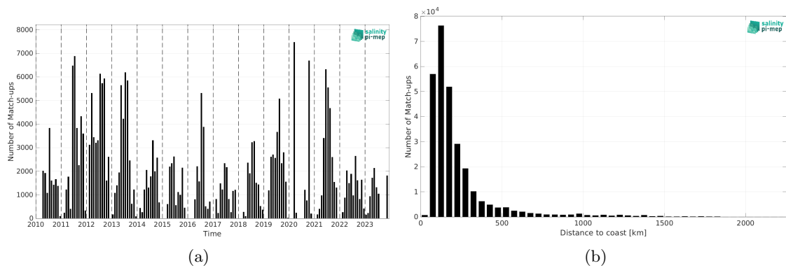
Figure 2: Number of match-ups between TSG (SAMOS) and CCI SSS L4 Merged-OI v5.5 - 30-day running (ESA) SSS as a function of time (a) and as function of the distance to coast (b) over the Gulf Stream Pi-MEP region and for the full satellite product period.
