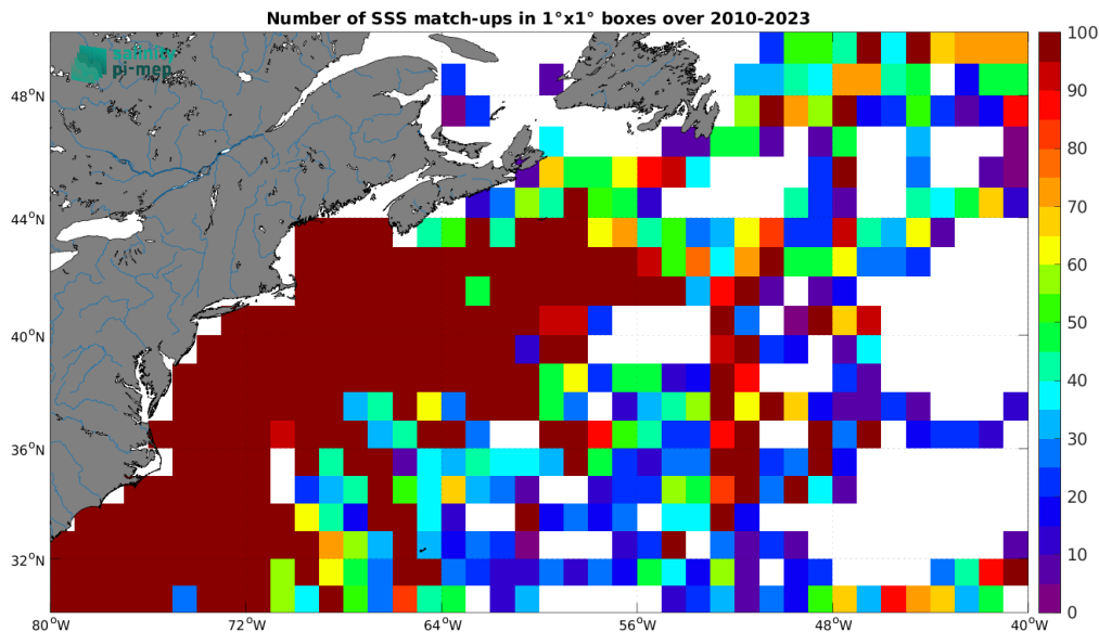
Figure 5: Number of SSS match-ups between TSG (SAMOS) SSS and the CCI SSS L4 Merged-OI v5.5 - 30-day running (ESA) SSS product for the Gulf Stream Pi-MEP region over 1^\circ \times 1^\circ boxes and for the full satellite product period.
