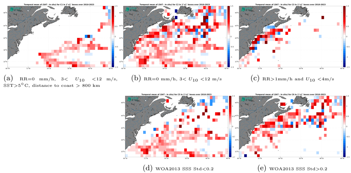
Figure 14: Temporal mean gridded over spatial boxes of size 1^\circ \times 1^\circ of \Delta\text{SSS} (CCI SSS L4 Merged-OI v5.5 - 30-day running (ESA) - TSG (SAMOS)) for 5 different subdatasets corresponding to:RR=0 mm/h, 3 < U_{10} < 12 m/s, SST >5^\circ\text{C} , distance to coast > 800 km (a), RR=0 mm/h, 3 < U_{10} < 12 m/s (b), RR >1 mm/h and U_{10} < 4 m/s (c), WOA2013 SSS Std <0.2 (d), WOA2013 SSS Std >0.2 (e).
