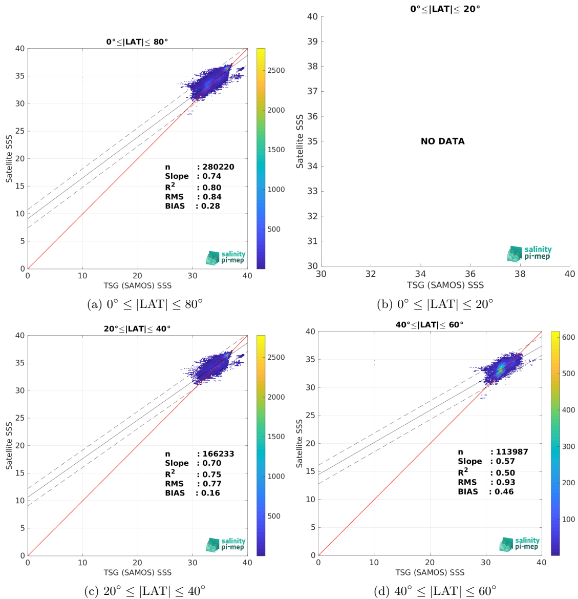
Figure 10: Contour maps of the concentration of CCI SSS L4 Merged-OI v5.5 - 30-day running (ESA) SSS (y-axis) versus TSG (SAMOS) SSS (x-axis) at match-up pairs for different latitude bands. For each plot, the red line shows x=y . The black thin and dashed lines indicate a linear fit through the data cloud and the \pm 95\% confidence levels, respectively. The number match-up pairs n , the slope and R^2 coefficient of the linear fit, the root mean square (RMS) and the mean bias between satellite and in situ data are indicated for each latitude band in each plots.
