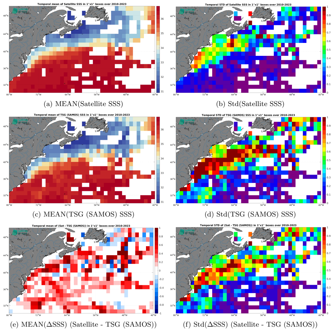
Figure 7: Temporal mean (left) and Std (right) of SSS from CCI SSS L4 Merged-OI v5.5 - 30-day running (ESA) (top), TSG (SAMOS) (middle), and of \Delta SSS (Satellite - TSG (SAMOS)). Only match-up pairs are used to generate these maps.
