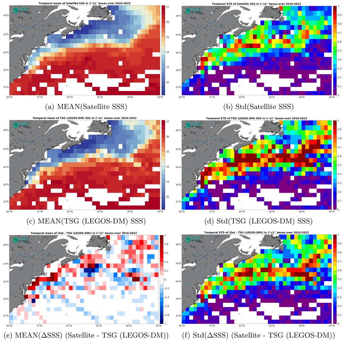
Figure 7: Temporal mean (left) and Std (right) of SSS from CCI SSS L4 Merged-OI v5.5 - 30-day running (ESA) (top), TSG (LEGOS-DM) (middle), and of \Delta SSS (Satellite - TSG (LEGOS-DM)). Only match-up pairs are used to generate these maps.
