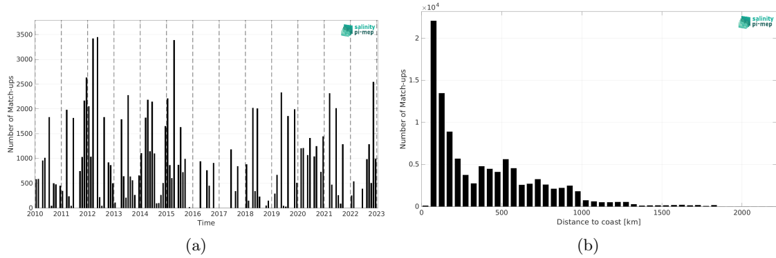
Figure 2: Number of match-ups between TSG (LEGOS-DM) and CCI SSS L4 Merged-OI v5.5 - 30-day running (ESA) SSS as a function of time (a) and as function of the distance to coast (b) over the Gulf Stream Pi-MEP region and for the full satellite product period.
