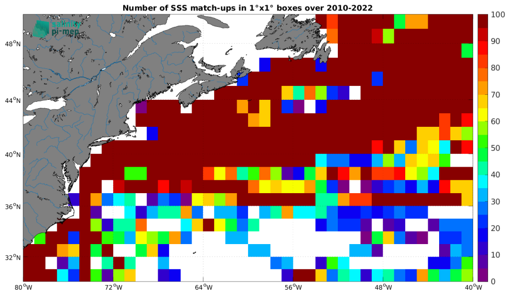
Figure 5: Number of SSS match-ups between TSG (LEGOS-DM) SSS and the CCI SSS L4 Merged-OI v5.5 - 30-day running (ESA) SSS product for the Gulf Stream Pi-MEP region over 1^\circ \times 1^\circ boxes and for the full satellite product period.
