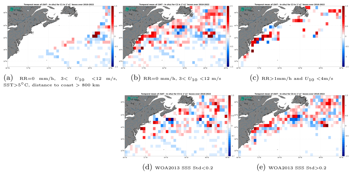
Figure 14: Temporal mean gridded over spatial boxes of size 1^\circ \times 1^\circ of \Delta\text{SSS} (CCI SSS L4 Merged-OI v5.5 - 30-day running (ESA) - TSG (LEGOS-DM)) for 5 different subdatasets corresponding to:RR=0 mm/h, 3 < U_{10} < 12 m/s, SST > 5^\circ\text{C} , distance to coast > 800 km (a), RR=0 mm/h, 3 < U_{10} < 12 m/s (b), RR > 1 mm/h and U_{10} < 4 m/s (c), WOA2013 SSS Std < 0.2 (d), WOA2013 SSS Std > 0.2 (e).
