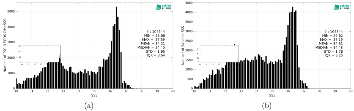
Figure 3: Histograms of SSS from TSG (LEGOS-DM) (a) and CCI SSS L4 Merged-OI v5.5 - 30-day running (ESA) (b) considering all match-up pairs per bins of 0.1 over the Gulf Stream Pi-MEP region and for the full satellite product period.
