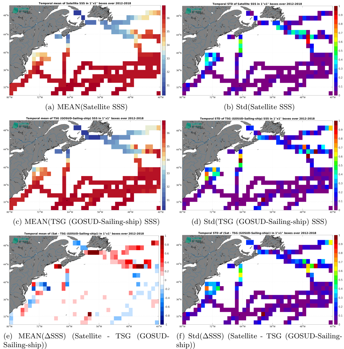
Figure 7: Temporal mean (left) and Std (right) of SSS from CCI SSS L4 Merged-OI v5.5 - 30-day running (ESA) (top), TSG (GOSUD-Sailing-ship) (middle), and of \Delta SSS (Satellite - TSG (GOSUD-Sailing-ship)). Only match-up pairs are used to generate these maps.
