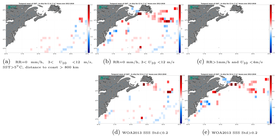
Figure 14: Temporal mean gridded over spatial boxes of size 1^\circ \times 1^\circ of \Delta SSS (CCI SSS L4 Merged-OI v5.5 - 30-day running (ESA) - TSG (GOSUD-Sailing-ship)) for 5 different subdatasets corresponding to:RR=0 mm/h, 3 < U_{10} < 12 m/s, SST >5^\circ\text{C} , distance to coast > 800 km (a), RR=0 mm/h, 3 < U_{10} < 12 m/s (b), RR >1 mm/h and U_{10} < 4 m/s (c), WOA2013 SSS Std <0.2 (d), WOA2013 SSS Std >0.2 (e).
