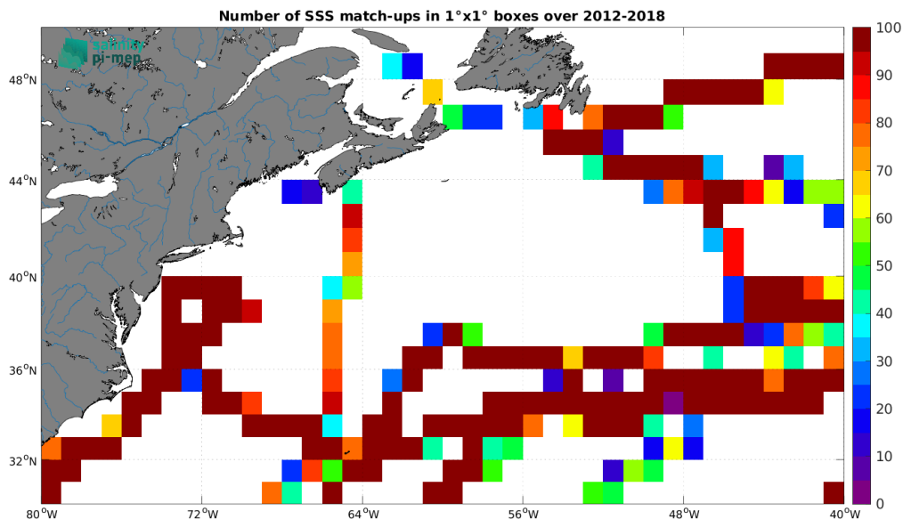
Figure 5: Number of SSS match-ups between TSG (GOSUD-Sailing-ship) SSS and the CCI SSS L4 Merged-OI v5.5 - 30-day running (ESA) SSS product for the Gulf Stream Pi-MEP region over 1^\circ \times 1^\circ boxes and for the full satellite product period.
