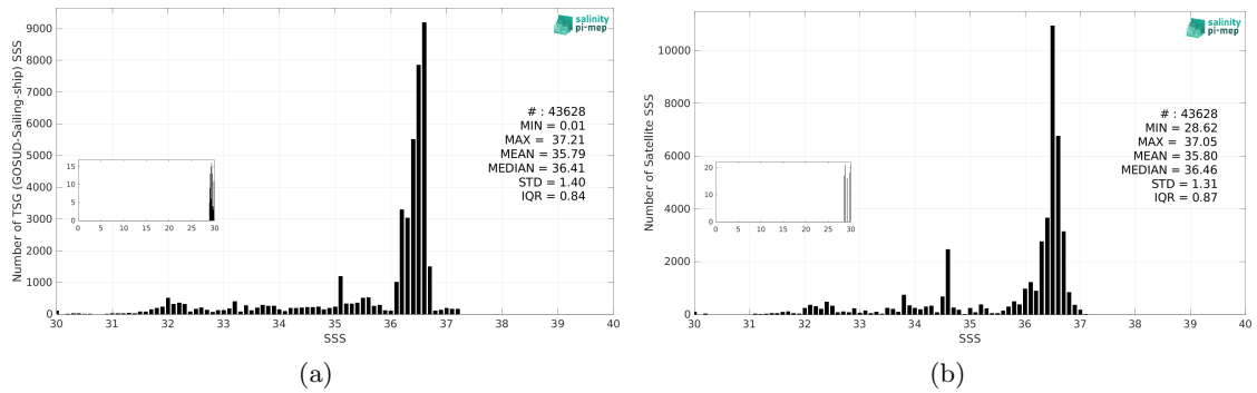
Figure 3: Histograms of SSS from TSG (GOSUD-Sailing-ship) (a) and CCI SSS L4 Merged-OI v5.5 - 30-day running (ESA) (b) considering all match-up pairs per bins of 0.1 over the Gulf Stream Pi-MEP region and for the full satellite product period.
