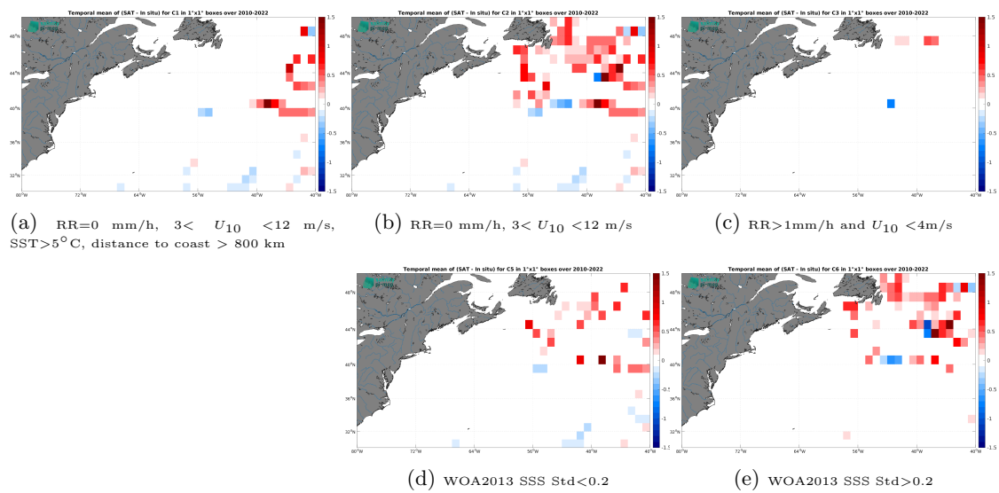
Figure 14: Temporal mean gridded over spatial boxes of size 1^\circ \times 1^\circ of \Delta SSS (CCI SSS L4 Merged-OI v5.5 - 30-day running (ESA) - TSG (GOSUD-Research-vessel)) for 5 different subdatasets corresponding to:RR=0 mm/h, 3 < U_{10} < 12 m/s, SST >5^\circ C, distance to coast > 800 km (a), RR=0 mm/h, 3 < U_{10} < 12 m/s (b), RR >1 mm/h and U_{10} < 4 m/s (c), WOA2013 SSS Std <0.2 (d), WOA2013 SSS Std >0.2 (e).
