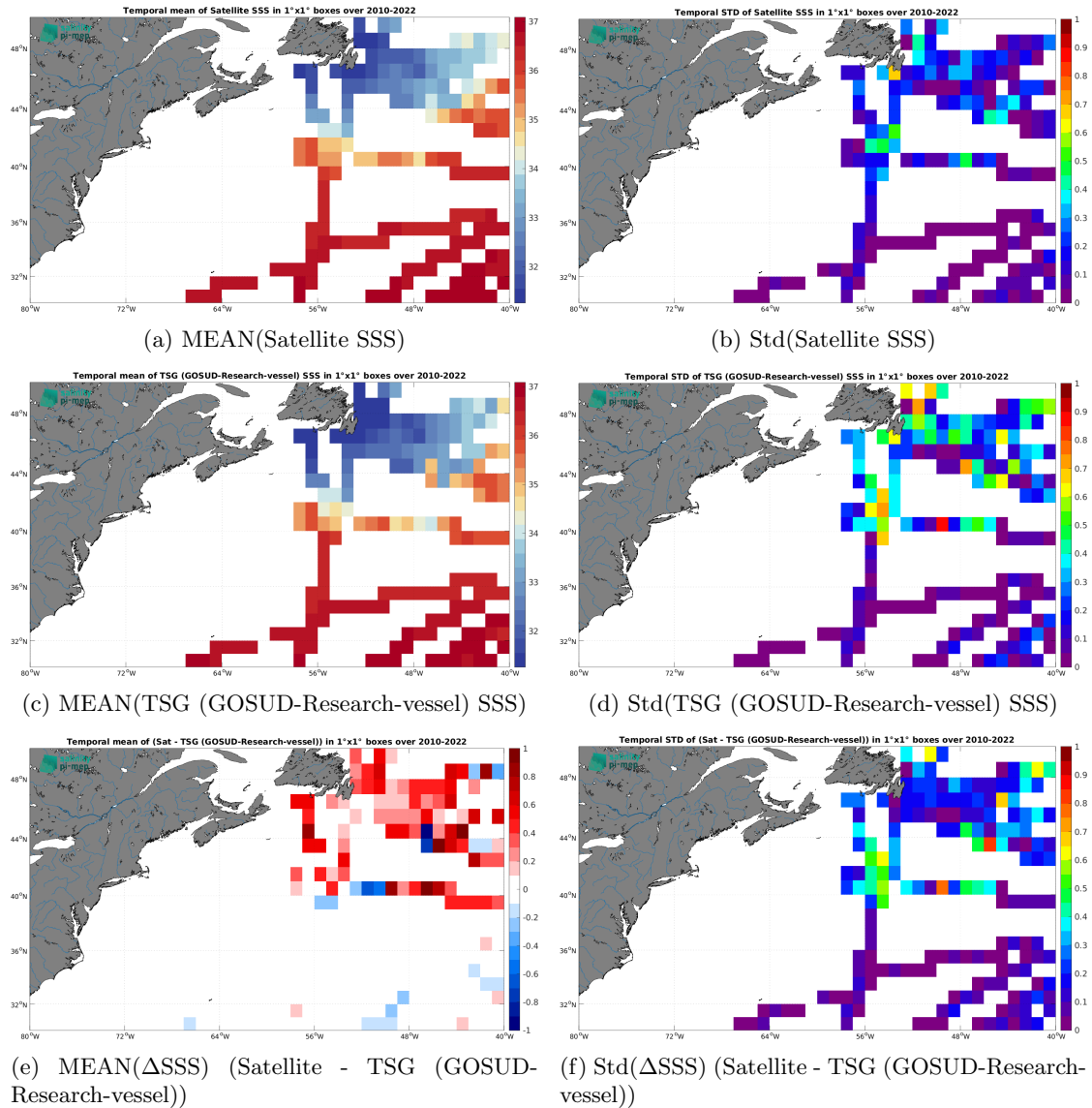
Figure 7: Temporal mean (left) and Std (right) of SSS from CCI SSS L4 Merged-OI v5.5 - 30-day running (ESA) (top), TSG (GOSUD-Research-vessel) (middle), and of \Delta SSS (Satellite - TSG (GOSUD-Research-vessel)). Only match-up pairs are used to generate these maps.
