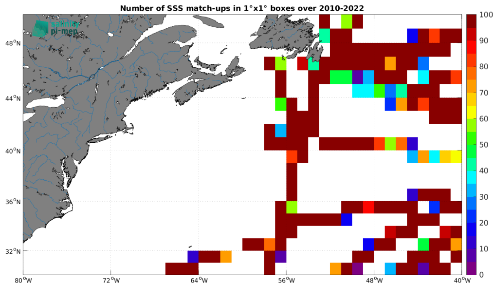
Figure 5: Number of SSS match-ups between TSG (GOSUD-Research-vessel) SSS and the CCI SSS L4 Merged-OI v5.5 - 30-day running (ESA) SSS product for the Gulf Stream Pi-MEP region over 1^\circ \times 1^\circ boxes and for the full satellite product period.
