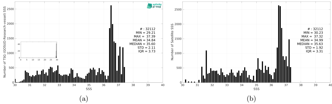
Figure 3: Histograms of SSS from TSG (GOSUD-Research-vessel) (a) and CCI SSS L4 Merged-OI v5.5 - 30-day running (ESA) (b) considering all match-up pairs per bins of 0.1 over the Gulf Stream Pi-MEP region and for the full satellite product period.
