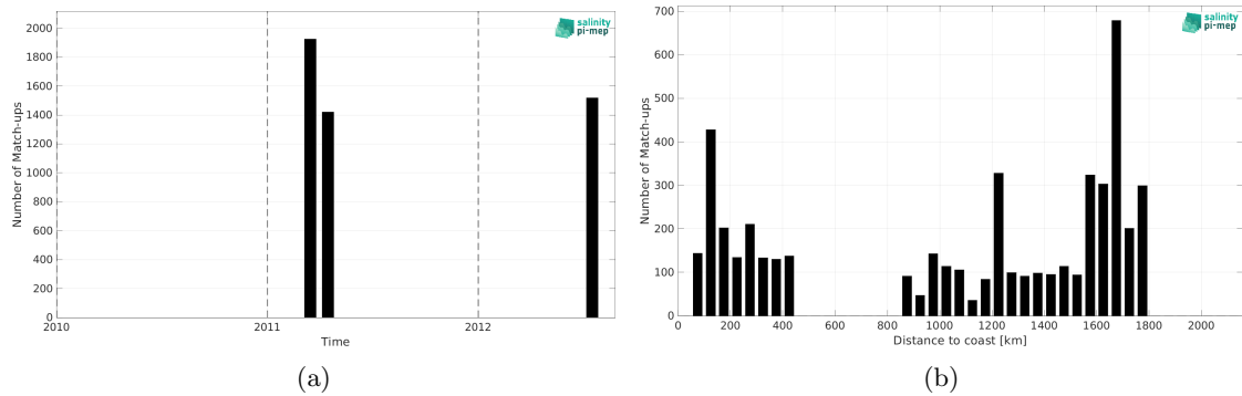
Figure 2: Number of match-ups between TSG (CSIC-UTM) and CCI SSS L4 Merged-OI v5.5 - 30-day running (ESA) SSS as a function of time (a) and as function of the distance to coast (b) over the Gulf Stream Pi-MEP region and for the full satellite product period.
