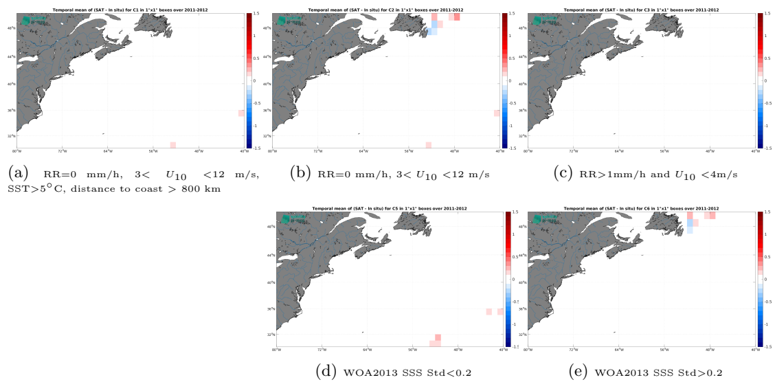
Figure 14: Temporal mean gridded over spatial boxes of size 1^\circ \times 1^\circ of \Delta SSS (CCI SSS L4 Merged-OI v5.5 - 30-day running (ESA) - TSG (CSIC-UTM)) for 5 different subdatasets corresponding to:RR=0 mm/h, 3 < U_{10} < 12 m/s, SST >5^\circ C, distance to coast > 800 km (a), RR=0 mm/h, 3 < U_{10} < 12 m/s (b), RR >1 mm/h and U_{10} < 4 m/s (c), WOA2013 SSS Std <0.2 (d), WOA2013 SSS Std >0.2 (e).
