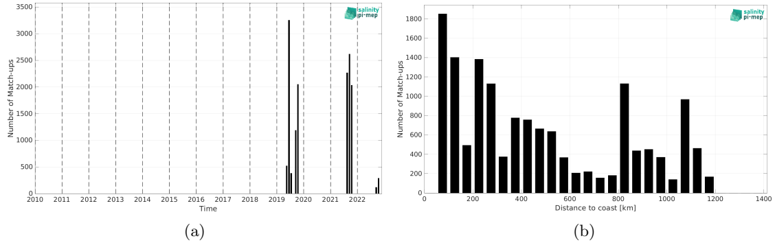
Figure 2: Number of match-ups between Saildrone and CCI SSS L4 Merged-OI v5.5 - 30-day running (ESA) SSS as a function of time (a) and as function of the distance to coast (b) over the Gulf Stream Pi-MEP region and for the full satellite product period.
