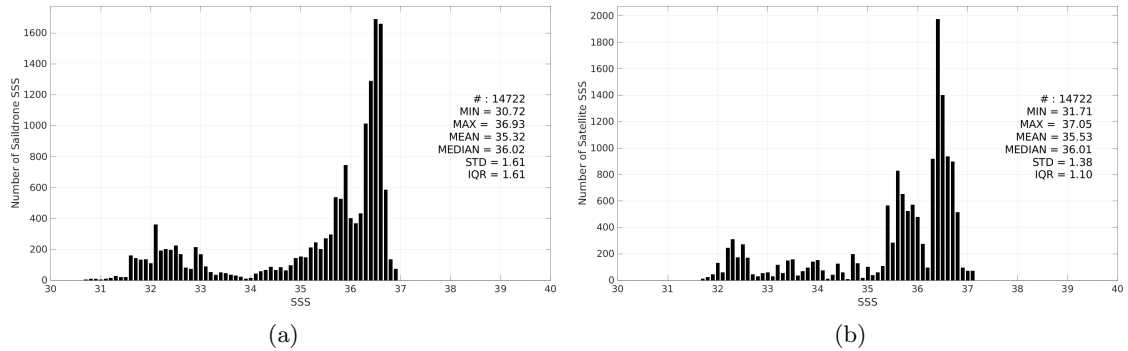
Figure 3: Histograms of SSS from Saildrone (a) and CCI SSS L4 Merged-OI v5.5 - 30-day running (ESA) (b) considering all match-up pairs per bins of 0.1 over the Gulf Stream Pi-MEP region and for the full satellite product period.
