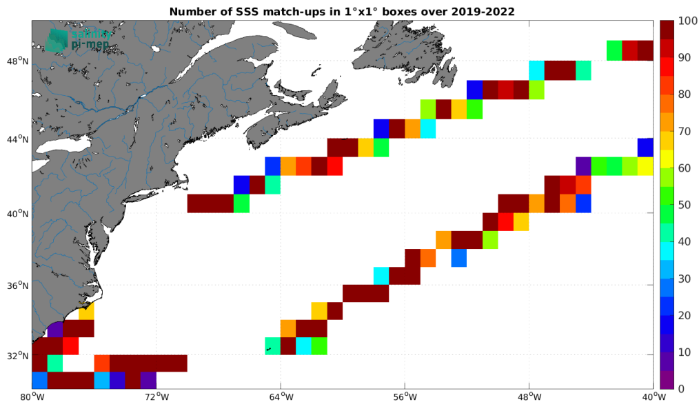
Figure 5: Number of SSS match-ups between Saildrone SSS and the CCI SSS L4 Merged-OI v5.5 - 30-day running (ESA) SSS product for the Gulf Stream Pi-MEP region over 1^\circ \times 1^\circ boxes and for the full satellite product period.
