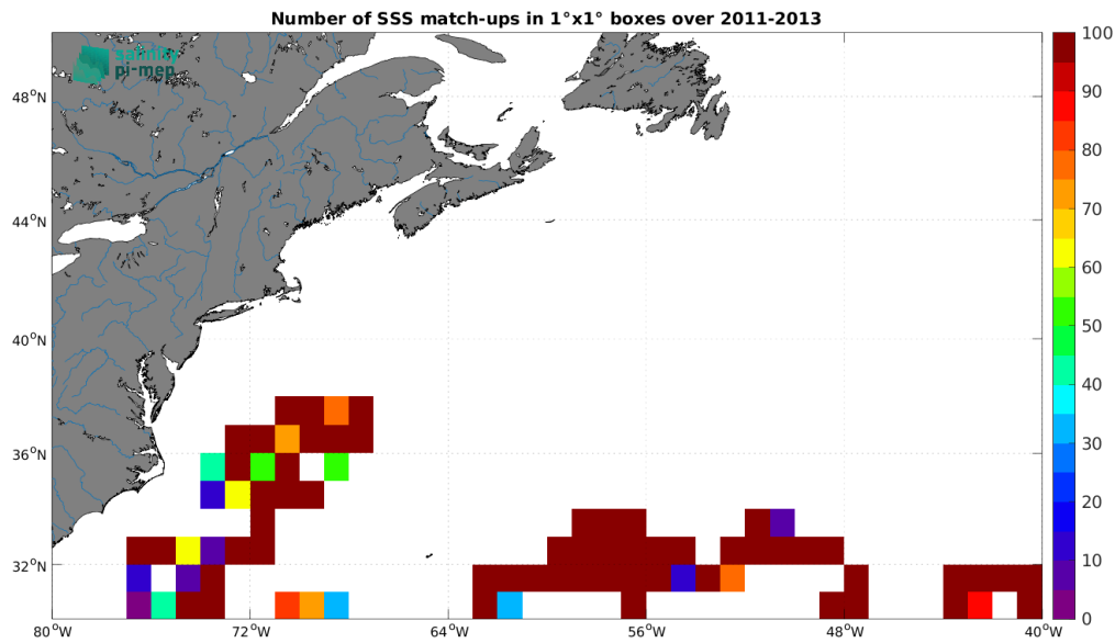
Figure 4: Number of SSS match-ups between Surface drifters SSS and the CCI SSS L4 Merged-OI v5.5 - 30-day running (ESA) SSS product for the Gulf Stream Pi-MEP region over 1^\circ \times 1^\circ boxes and for the full satellite product period.
