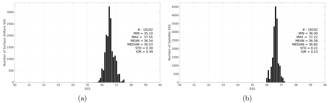
Figure 3: Histograms of SSS from Surface drifters (a) and CCI SSS L4 Merged-OI v5.5 - 30-day running (ESA) (b) considering all match-up pairs per bins of 0.1 over the Gulf Stream Pi-MEP region and for the full satellite product period.
