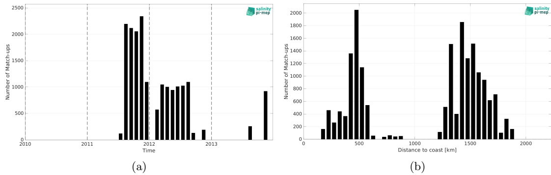
Figure 2: Number of match-ups between Surface drifters and CCI SSS L4 Merged-OI v5.5 - 30-day running (ESA) SSS as a function of time (a) and as function of the distance to coast (b) over the Gulf Stream Pi-MEP region and for the full satellite product period.
