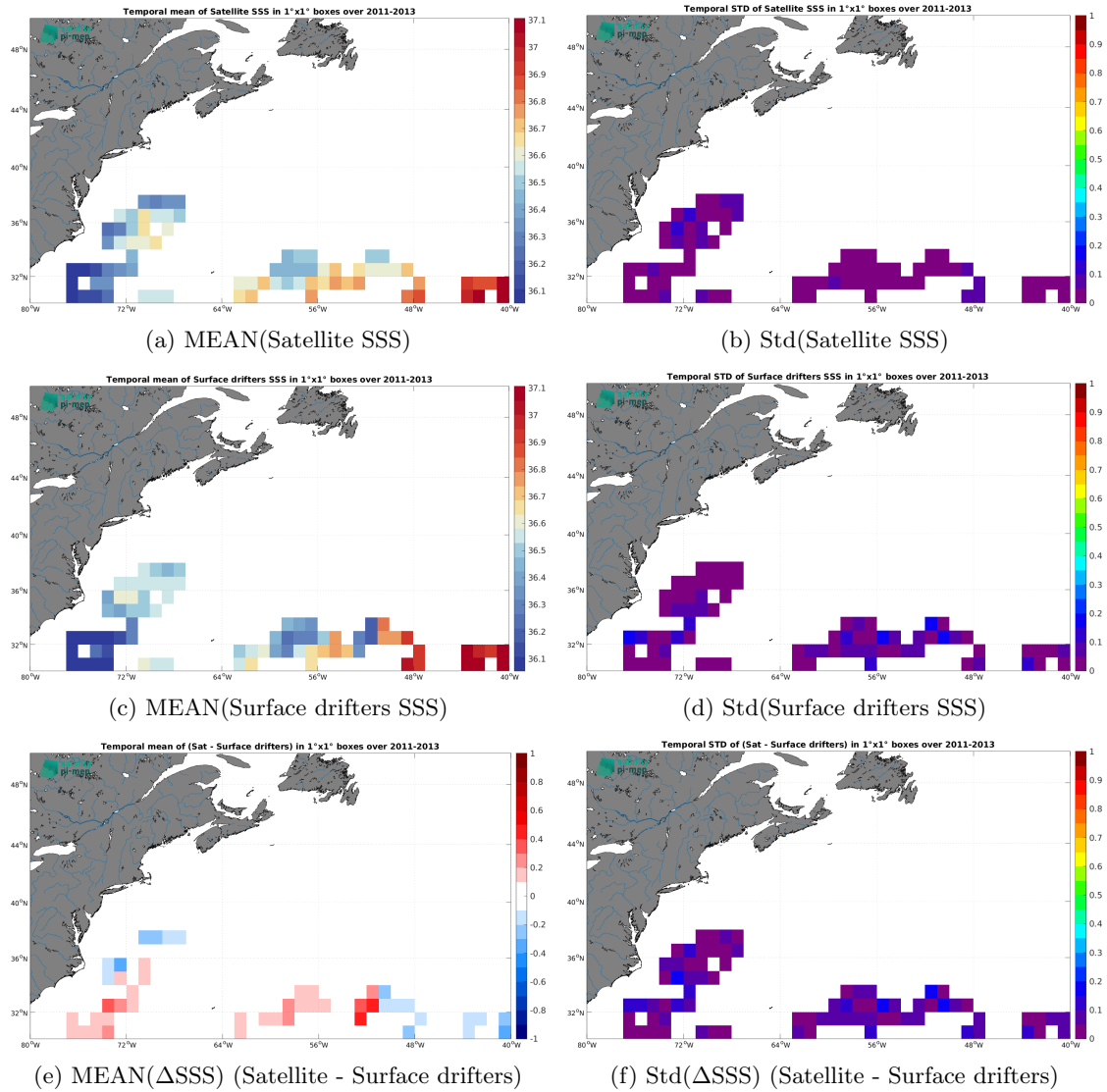
Figure 6: Temporal mean (left) and Std (right) of SSS from CCI SSS L4 Merged-OI v5.5 - 30-day running (ESA) (top), Surface drifters (middle), and of \Delta SSS (Satellite - Surface drifters). Only match-up pairs are used to generate these maps.
