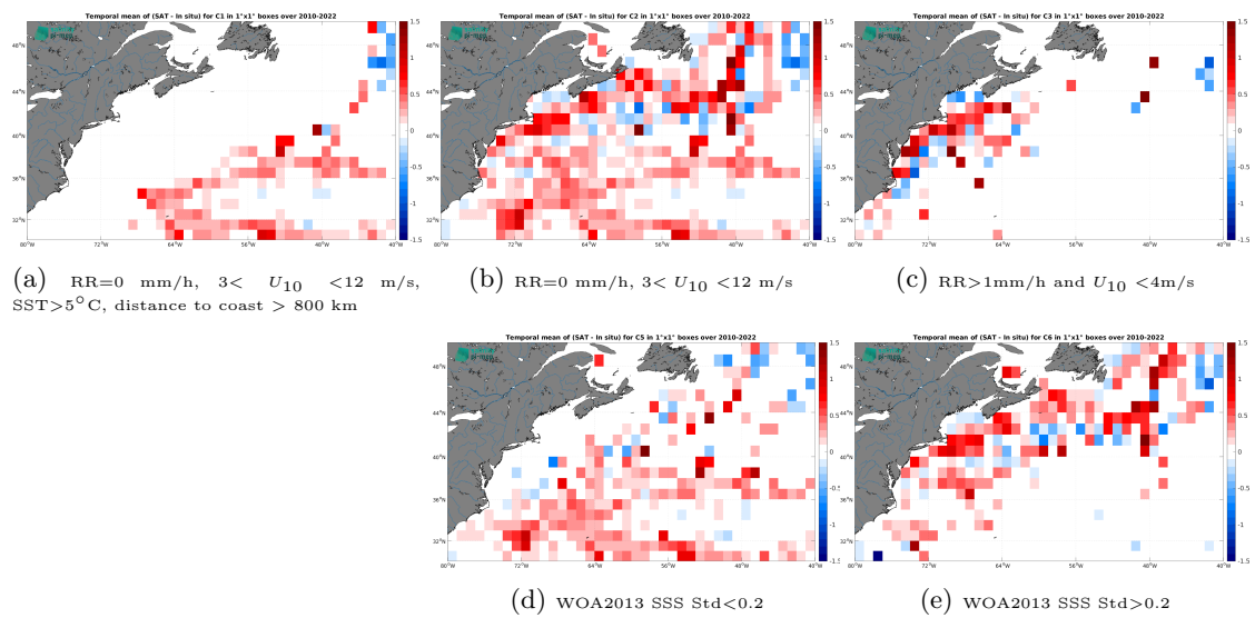
Figure 14: Temporal mean gridded over spatial boxes of size 1^\circ \times 1^\circ of \Delta SSS (CCI SSS L4 Merged-OI v4.41 - 7-day running (ESA) - TSG (SAMOS)) for 5 different subdatasets corresponding to: RR=0 mm/h, 3 < U_{10} < 12 m/s, SST > 5^\circ\text{C} , distance to coast > 800 km (a), RR=0 mm/h, 3 < U_{10} < 12 m/s (b), RR > 1 mm/h and U_{10} < 4 m/s (c), WOA2013 SSS Std < 0.2 (d), WOA2013 SSS Std > 0.2 (e).
